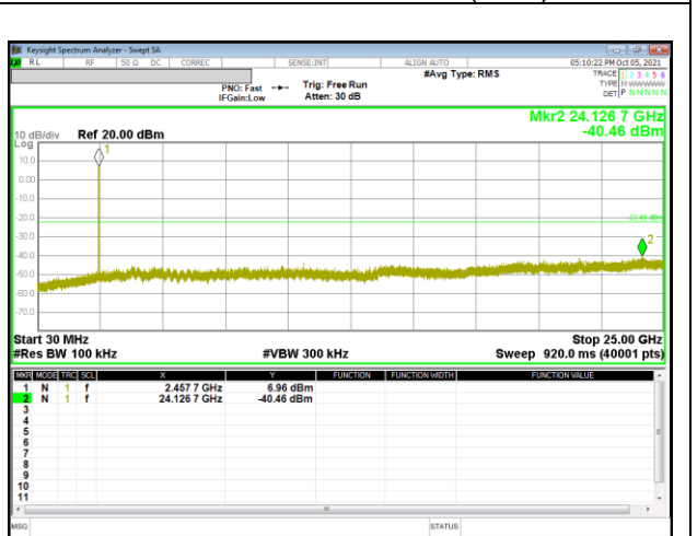
Out-Of-Band 11 Channel(8RU)
