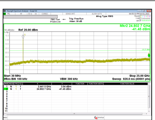
Out-Of-Band 10 Channel
