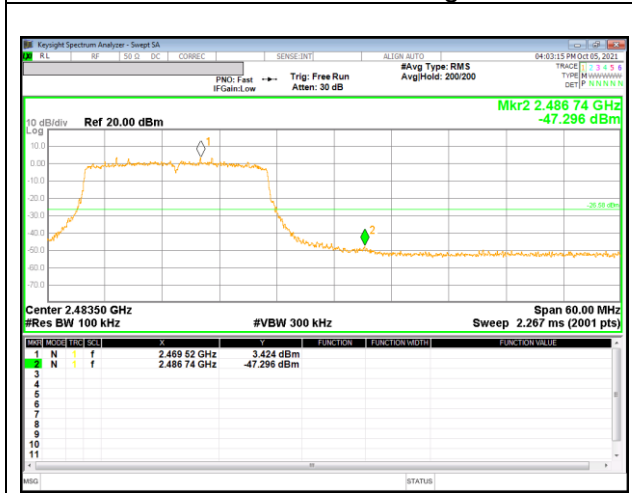
12 Channel Band-edge_SISO
