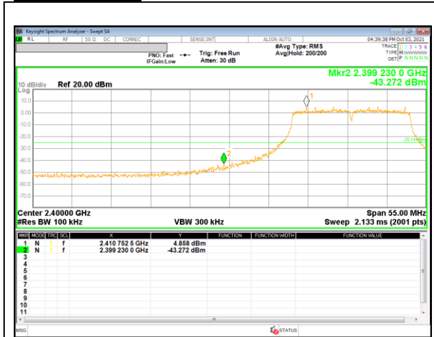
2 Channel Band-edge
