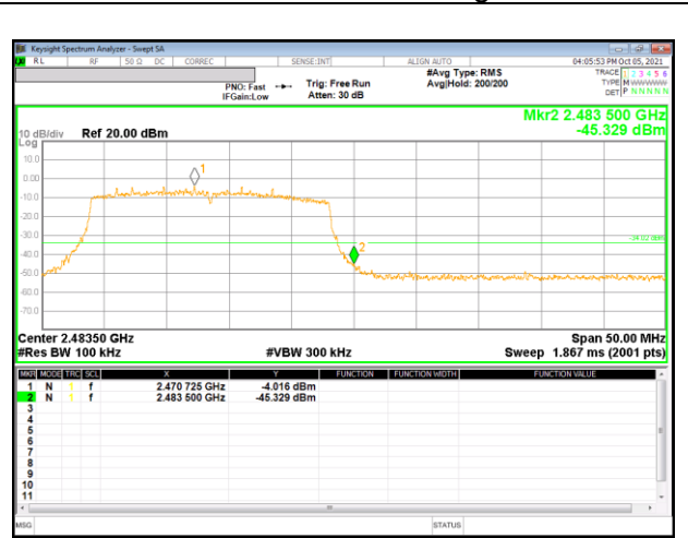
13 Channel Band-edge_SISO
