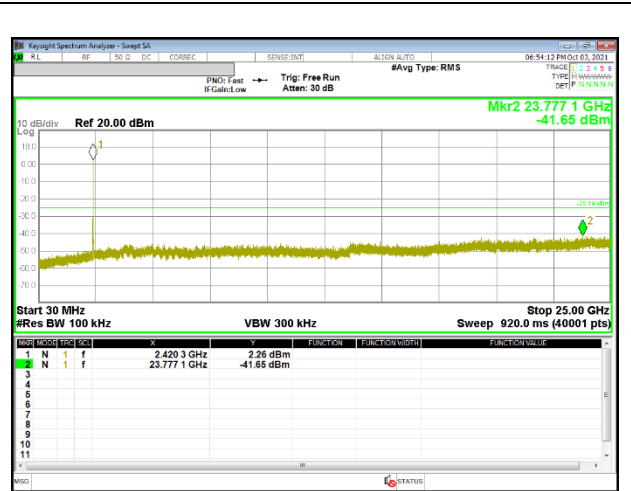
Out-Of-Band 2 Channel
