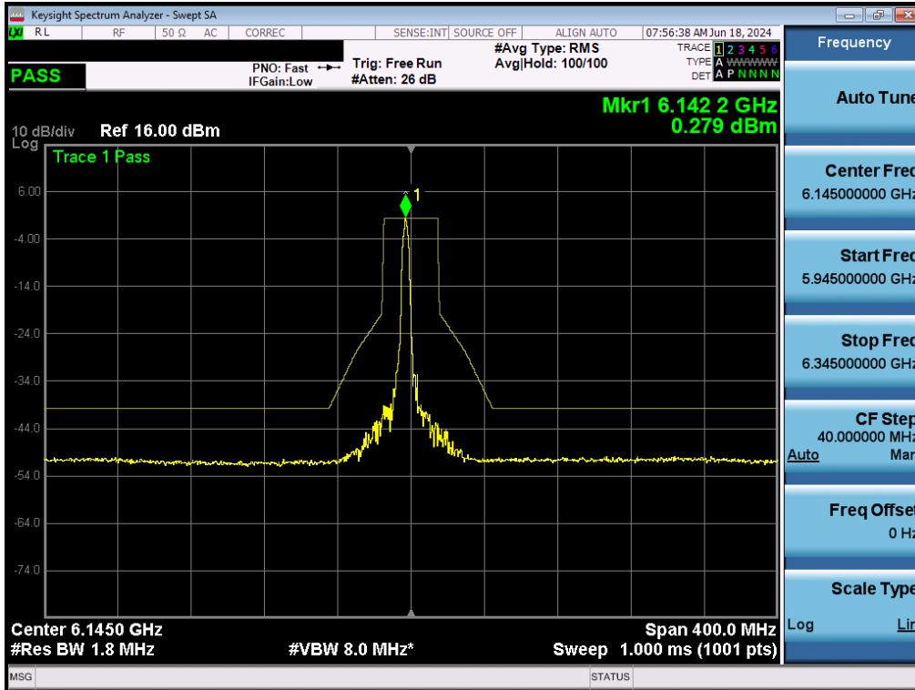
Plot 7-163. In-Band Emissions Plot MIMO ANT2 (80MHz BW 802.11ax (26 Tones) (UNII Band 5) – Ch. 39) - LPI/SP
