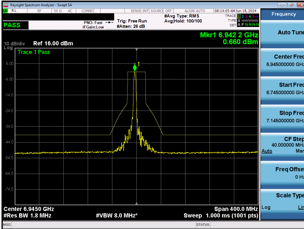
Plot 7-175. In-Band Emissions Plot MIMO ANT2 (80MHz BW 802.11ax (26 Tones) (UNII Band 8) – Ch. 199) - LPI/SP
