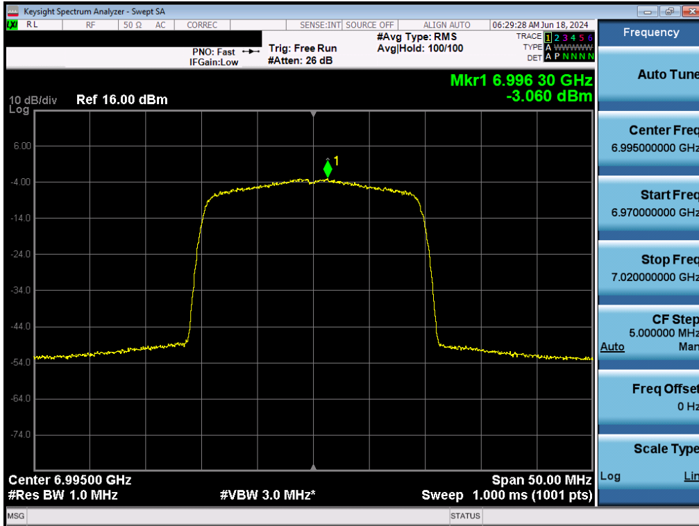
Plot 7-125. Power Spectral Density Plot MIMO ANT2 (20MHz BW 802.11ax (Full Tones) (UNII Band 8) – Ch. 209) - LPI/SP
