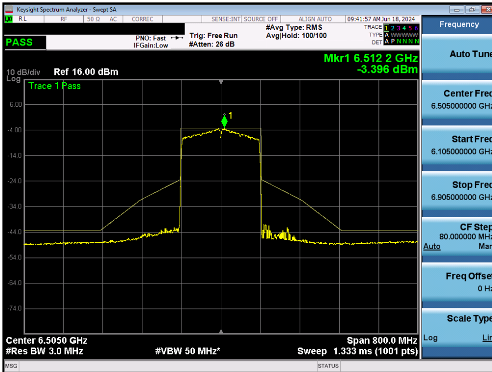
Plot 7-184. In-Band Emissions Plot MIMO ANT2 (160MHz BW 802.11ax (Full Tones) (UNII Band 6) – Ch. 111) - LPI/SP
