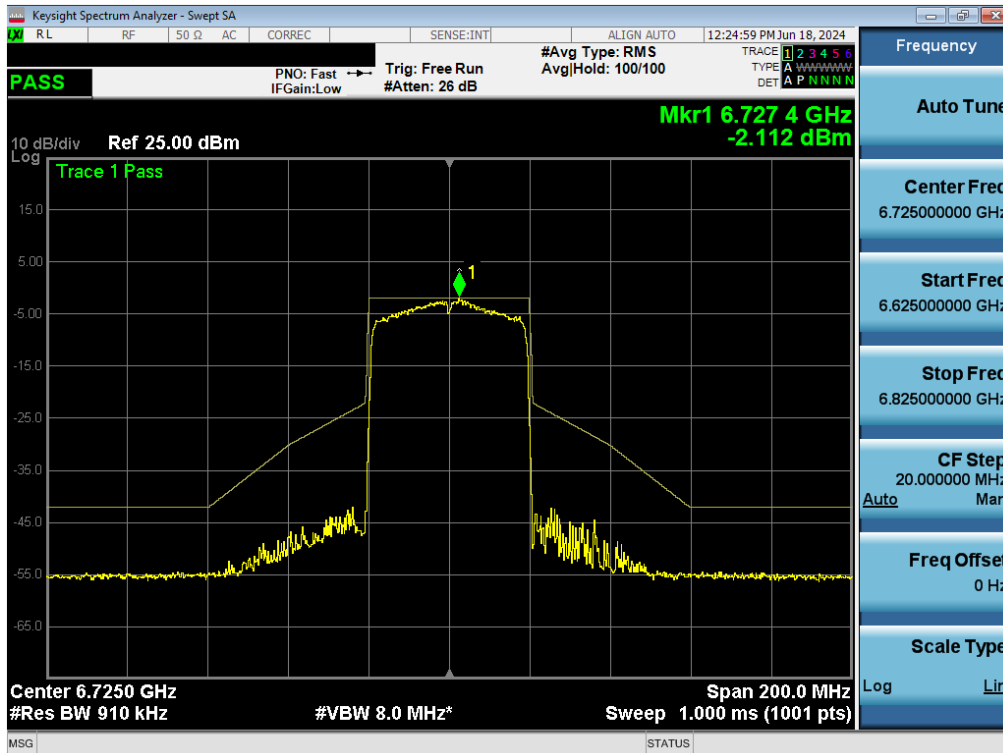
Plot 7-154. In-Band Emissions Plot MIMO ANT1 (40MHz BW 802.11ax (Full Tones) (UNII Band 7) – Ch. 155) - LPI/SP
