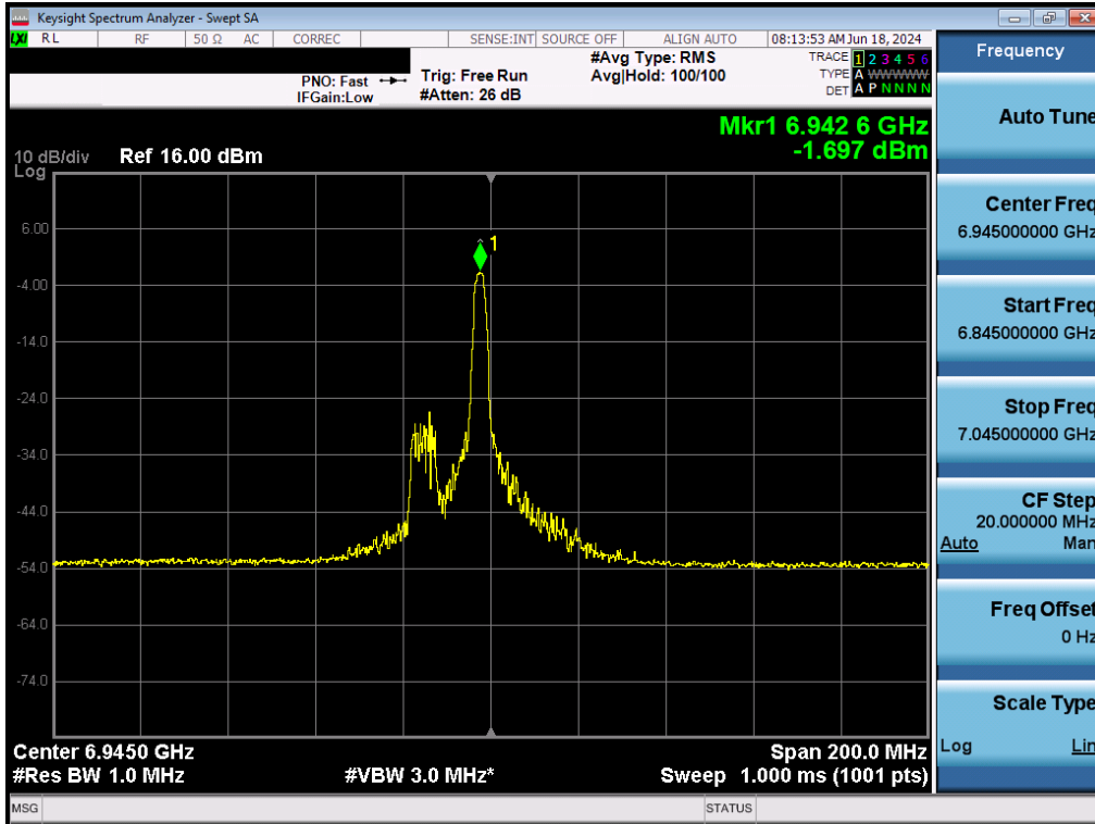
Plot 7-111. Power Spectral Density Plot MIMO ANT2 (80MHz BW 802.11ax (26 Tones) (UNII Band 8) – Ch. 199) - LPI/SP
