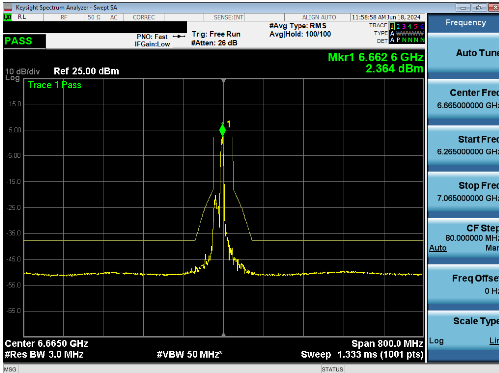
Plot 7-140. In-Band Emissions Plot MIMO ANT1 (160MHz BW 802.11ax (26 Tones) (UNII Band 7) – Ch. 143) - LPI/SP
