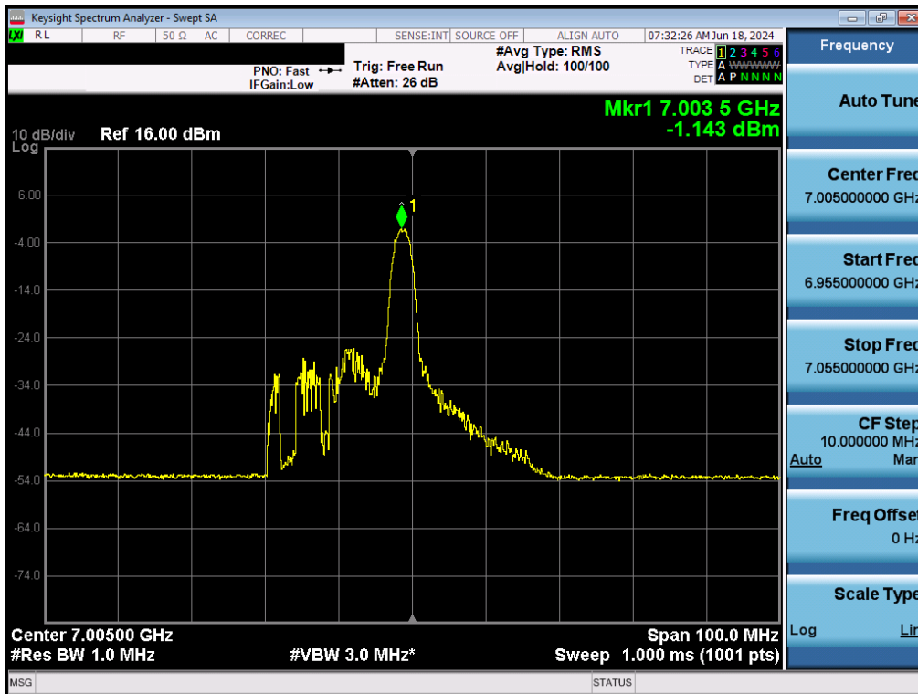
Plot 7-110. Power Spectral Density Plot MIMO ANT2 (40MHz BW 802.11ax (26 Tones) (UNII Band 8) – Ch. 211) - LPI/SP
