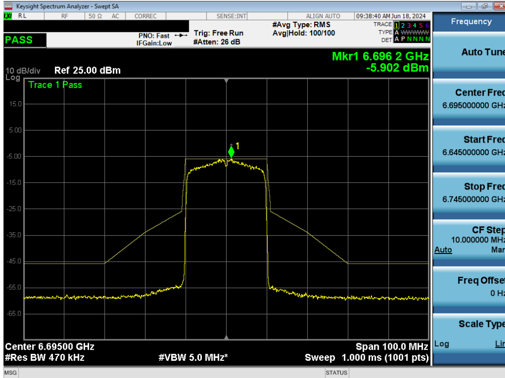
Plot 7-153. In-Band Emissions Plot MIMO ANT1 (20MHz BW 802.11ax (Full Tones) (UNII Band 7) – Ch. 149) - LPI/SP
