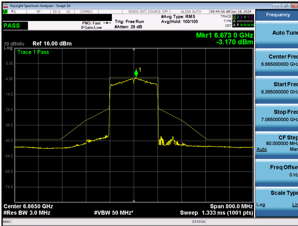
Plot 7-188. In-Band Emissions Plot MIMO ANT2 (160MHz BW 802.11ax (Full Tones) (UNII Band 7) – Ch. 143) - LPI/SP
