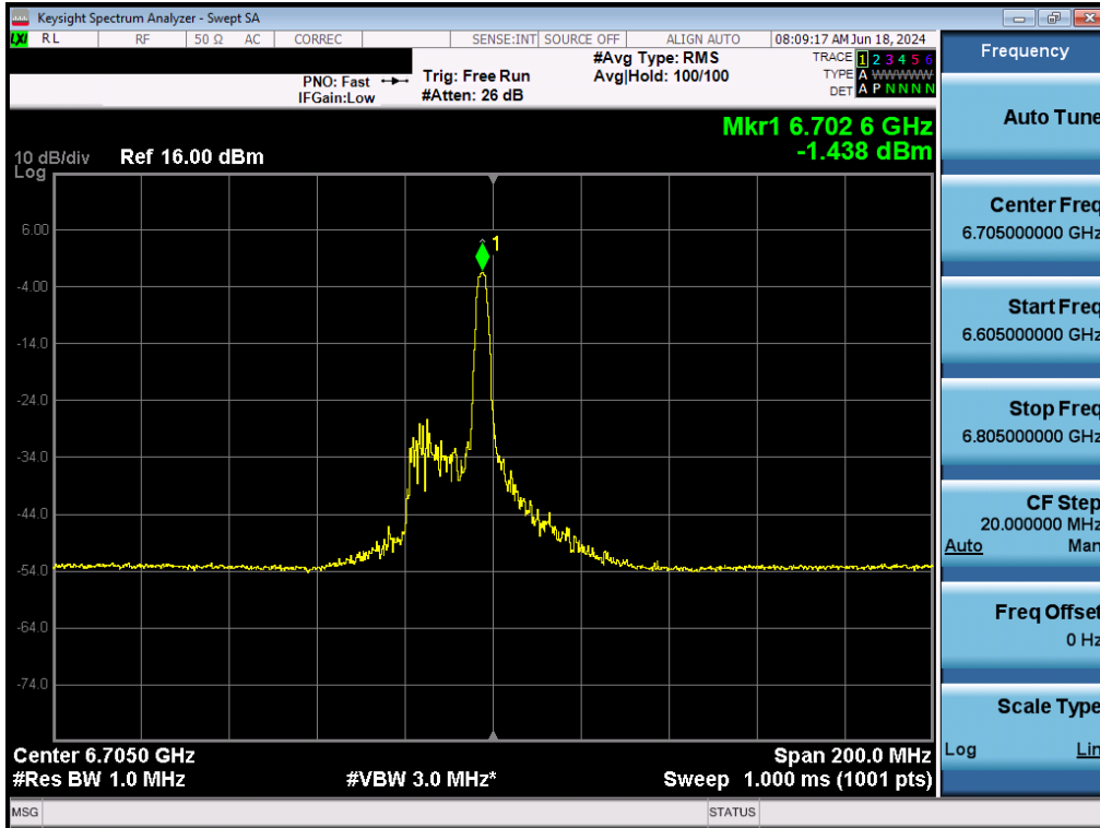
Plot 7-107. Power Spectral Density Plot MIMO ANT2 (80MHz BW 802.11ax (26 Tones) (UNII Band 7) – Ch. 151) - LPI/SP
