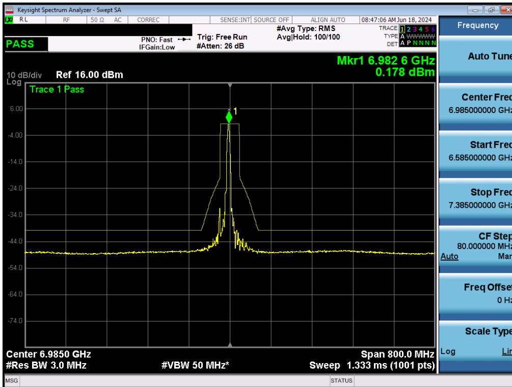
Plot 7-176. In-Band Emissions Plot MIMO ANT2 (160MHz BW 802.11ax (26 Tones) (UNII Band 8) – Ch. 207) - LPI/SP
