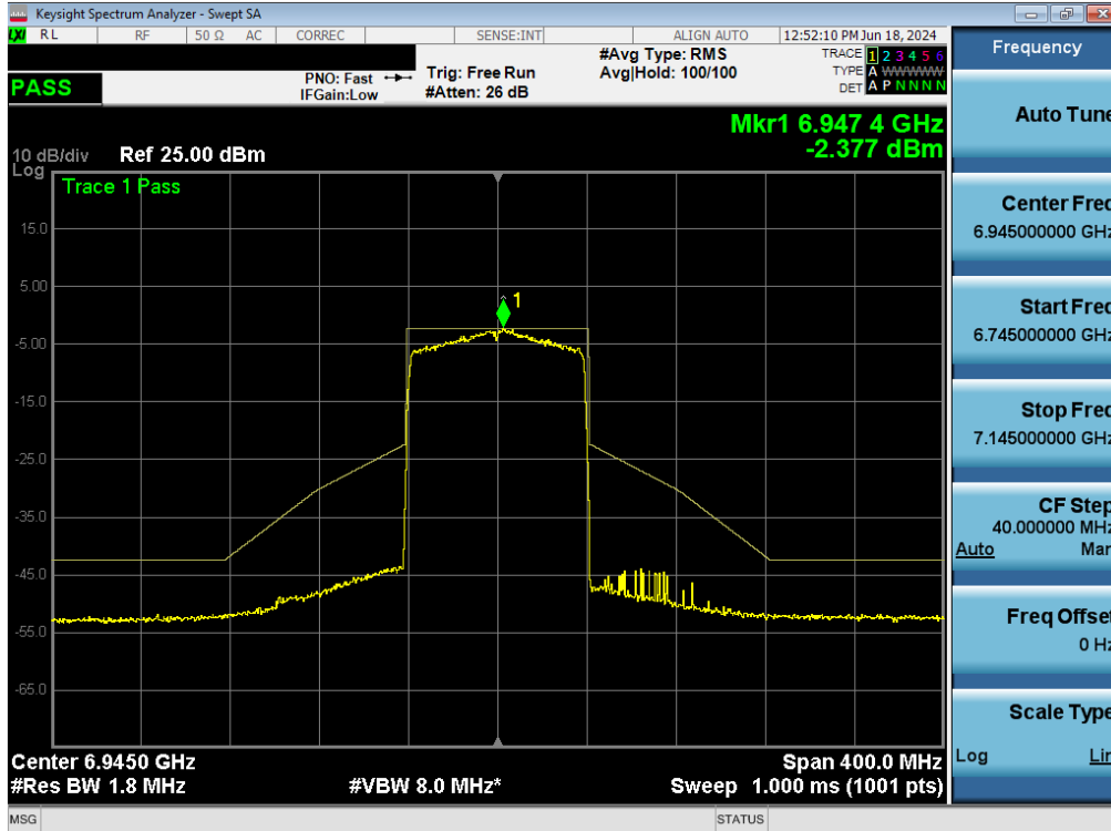
Plot 7-159. In-Band Emissions Plot MIMO ANT1 (80MHz BW 802.11ax (Full Tones) (UNII Band 8) – Ch. 199) - LPI/SP
