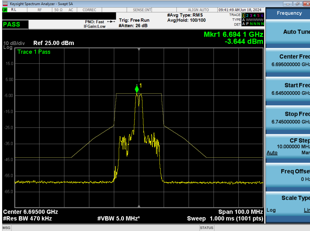
Plot 7-137. In-Band Emissions Plot MIMO ANT1 (20MHz BW 802.11ax (26 Tones) (UNII Band 7) – Ch. 149) - LPI/SP
