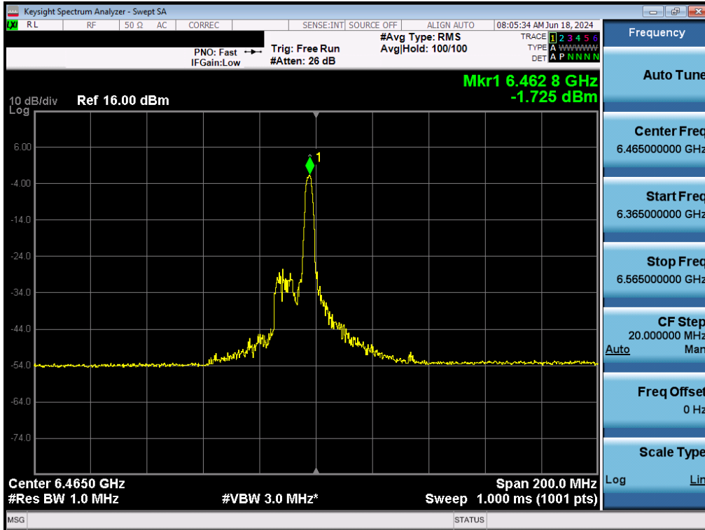
Plot 7-103. Power Spectral Density Plot MIMO ANT2 (80MHz BW 802.11ax (26 Tones) (UNII Band 6) – Ch. 103) - LPI/SP
