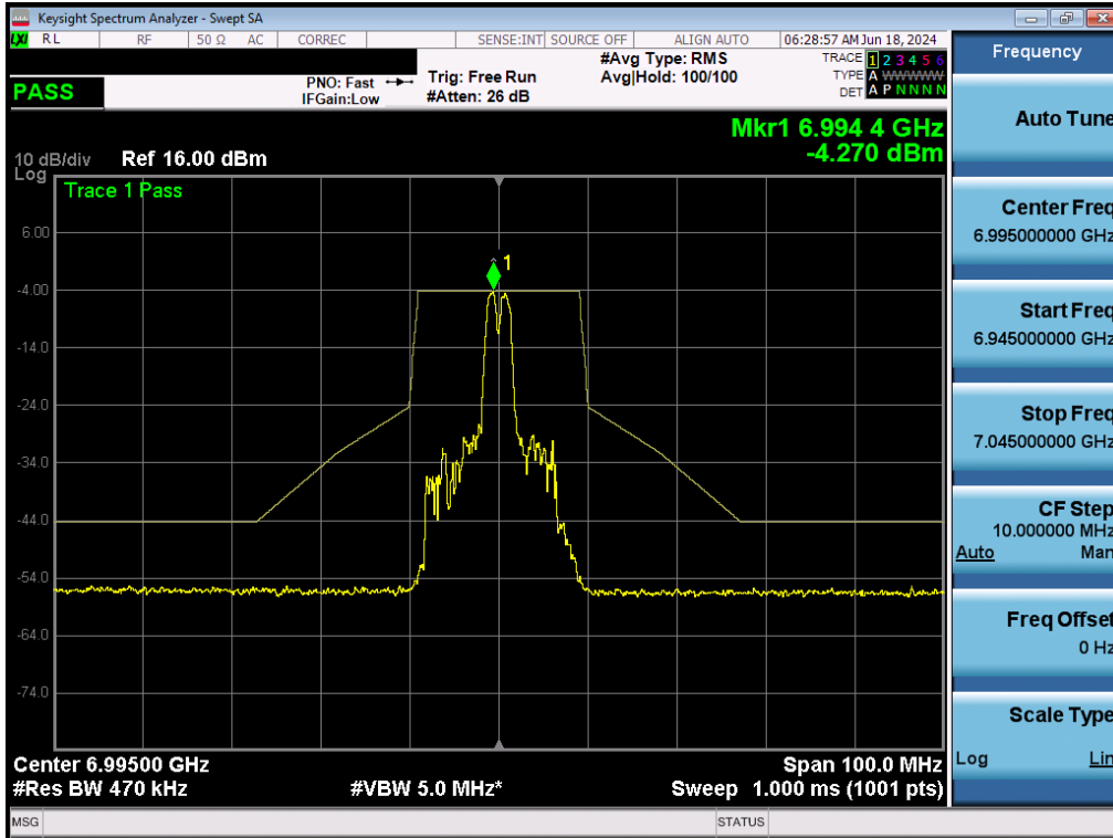
Plot 7-173. In-Band Emissions Plot MIMO ANT2 (20MHz BW 802.11ax (26 Tones) (UNII Band 8) – Ch. 209) - LPI/SP
