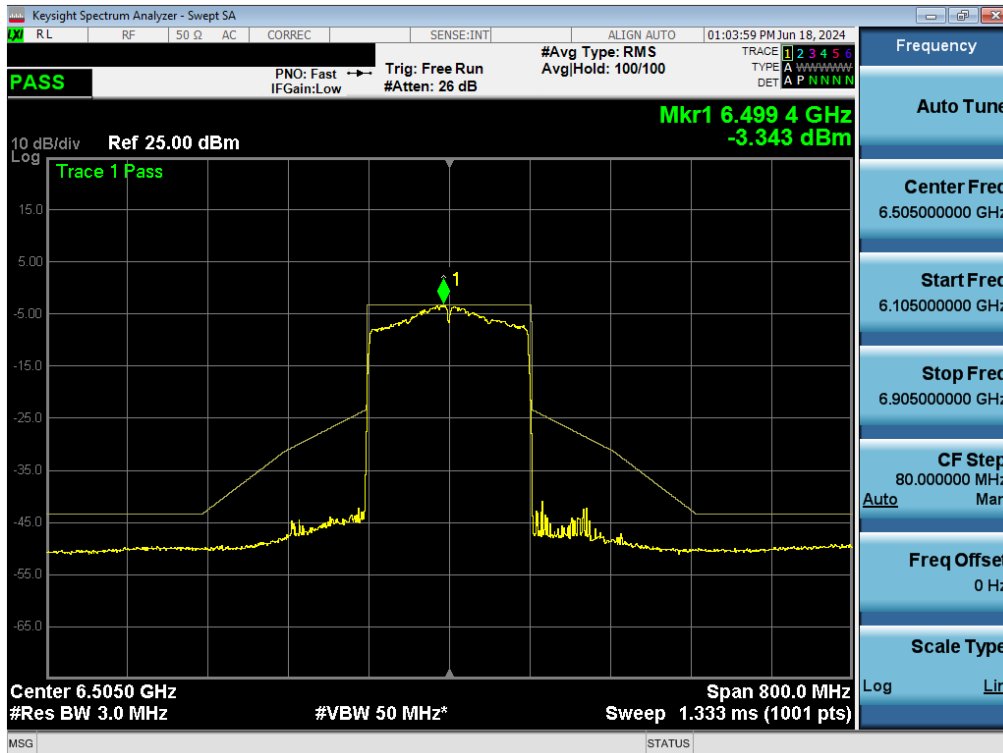
Plot 7-152. In-Band Emissions Plot MIMO ANT1 (160MHz BW 802.11ax (Full Tones) (UNII Band 6) – Ch. 111) - LPI/SP
