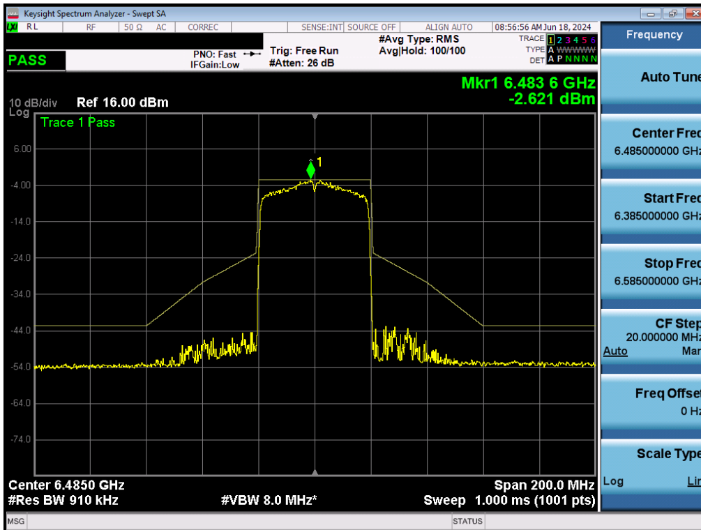
Plot 7-182. In-Band Emissions Plot MIMO ANT2 (40MHz BW 802.11ax (Full Tones) (UNII Band 6) – Ch. 107) - LPI/SP
