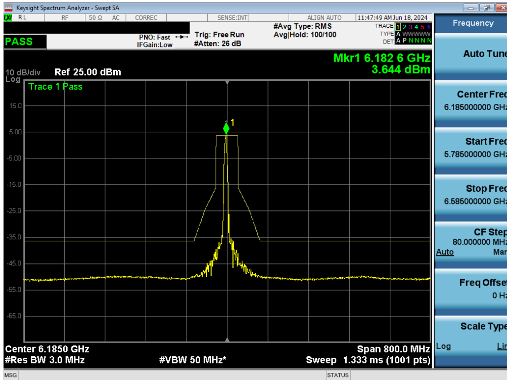
Plot 7-132. In-Band Emissions Plot MIMO ANT1 (160MHz BW 802.11ax (26 Tones) (UNII Band 5) – Ch. 47) - LPI/SP
