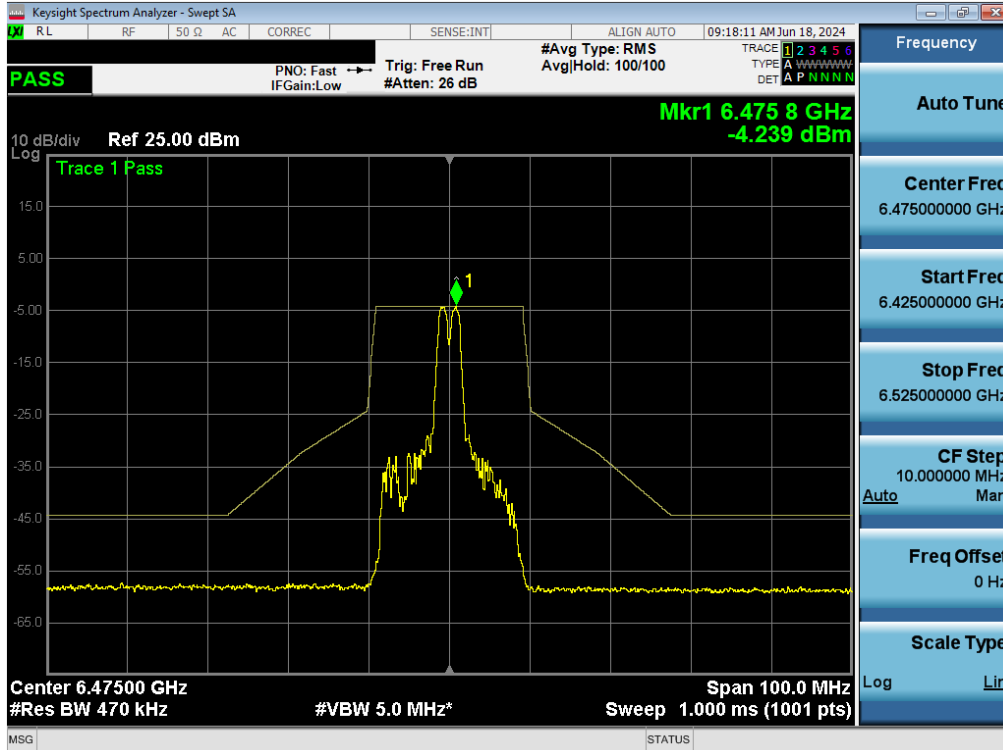
Plot 7-133. In-Band Emissions Plot MIMO ANT1 (20MHz BW 802.11ax (26 Tones) (UNII Band 6) – Ch. 105) - LPI/SP
