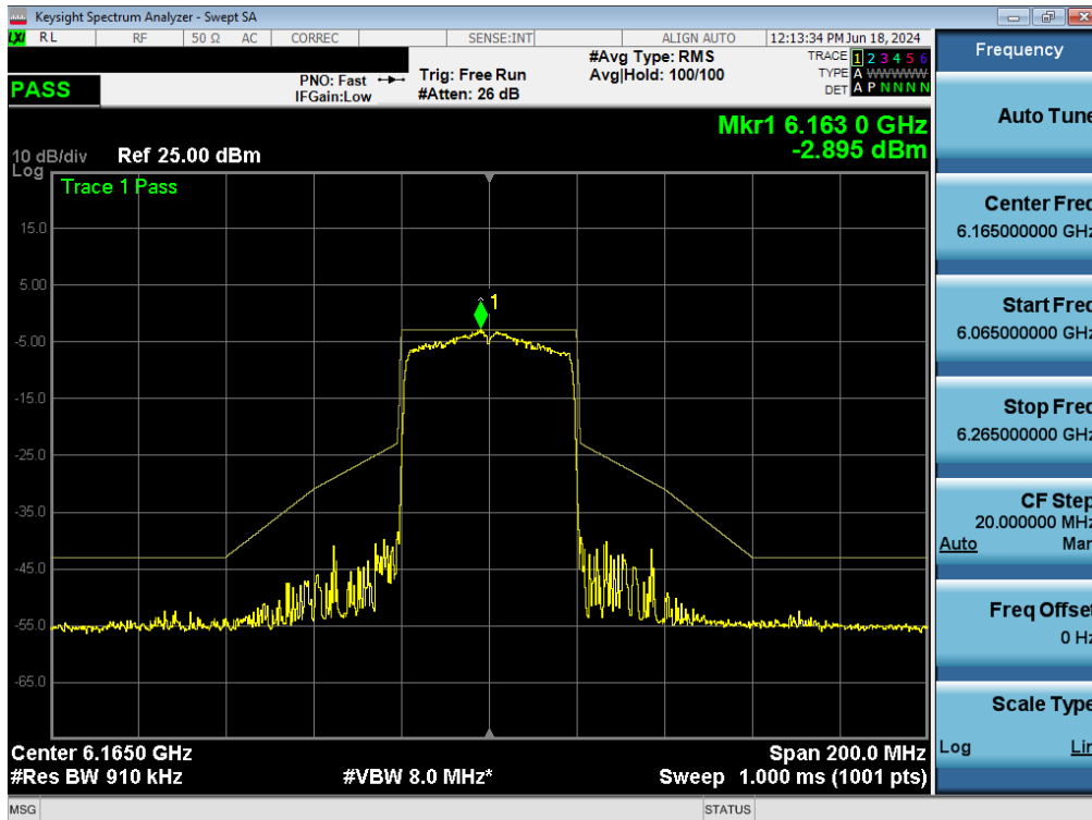
Plot 7-146. In-Band Emissions Plot MIMO ANT1 (40MHz BW 802.11ax (Full Tones) (UNII Band 5) – Ch. 43) - LPI/SP
