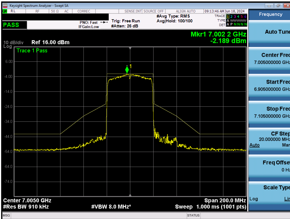
Plot 7-190. In-Band Emissions Plot MIMO ANT2 (40MHz BW 802.11ax (Full Tones) (UNII Band 8) – Ch. 211) - LPI/SP
