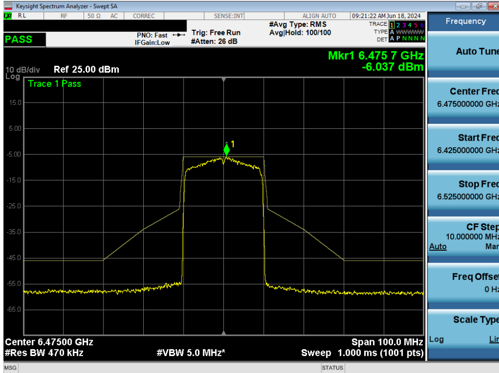
Plot 7-149. In-Band Emissions Plot MIMO ANT1 (20MHz BW 802.11ax (Full Tones) (UNII Band 6) – Ch. 105) - LPI/SP
