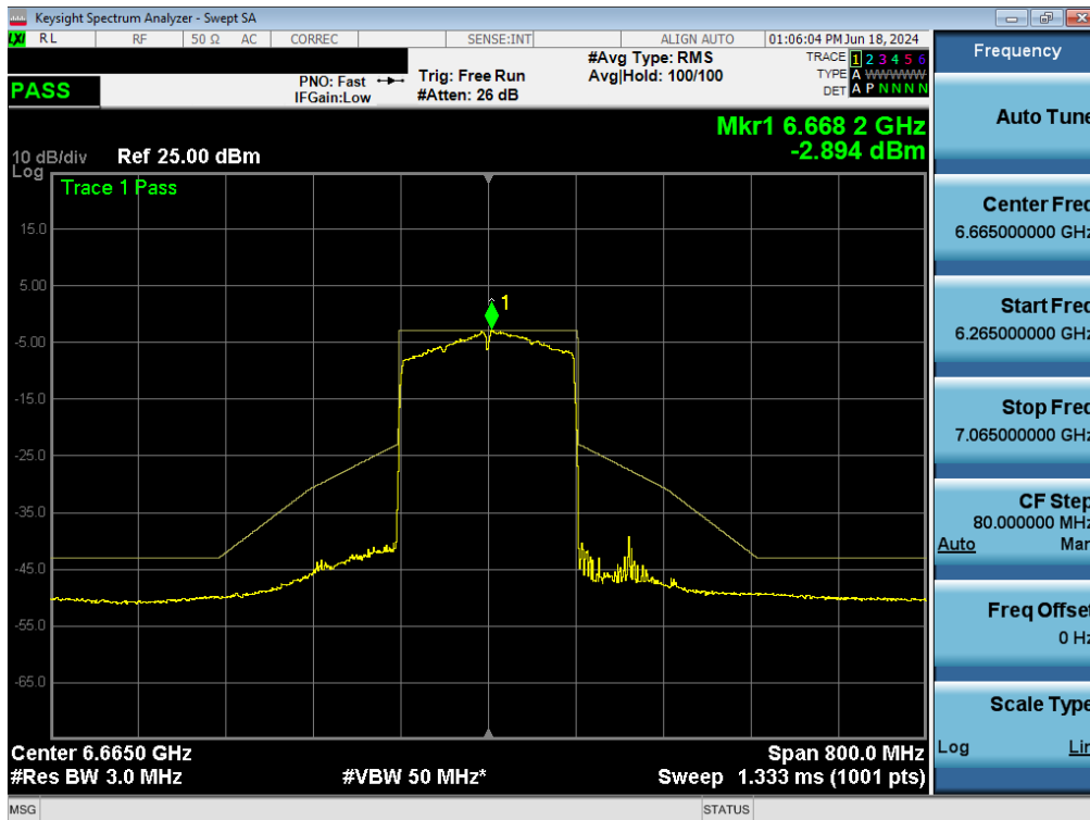
Plot 7-156. In-Band Emissions Plot MIMO ANT1 (160MHz BW 802.11ax (Full Tones) (UNII Band 7) – Ch. 143) - LPI/SP
