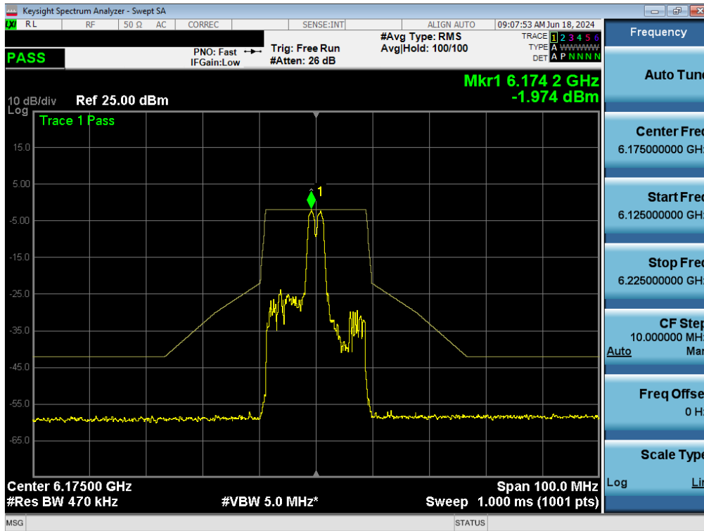
Plot 7-129. In-Band Emissions Plot MIMO ANT1 (20MHz BW 802.11ax (26 Tones) (UNII Band 5) – Ch. 45) – LPI/SP
