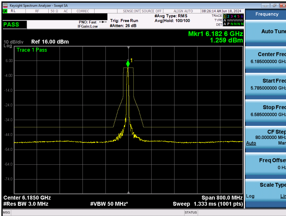
Plot 7-164. In-Band Emissions Plot MIMO ANT2 (160MHz BW 802.11ax (26 Tones) (UNII Band 5) – Ch. 47) - LPI/SP
