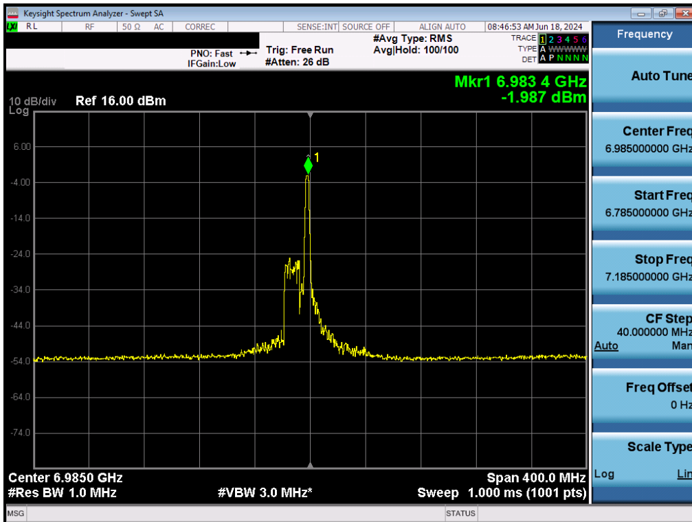
Plot 7-112. Power Spectral Density Plot MIMO ANT2 (160MHz BW 802.11ax (26 Tones) (UNII Band 8) – Ch. 207) - LPI/SP
