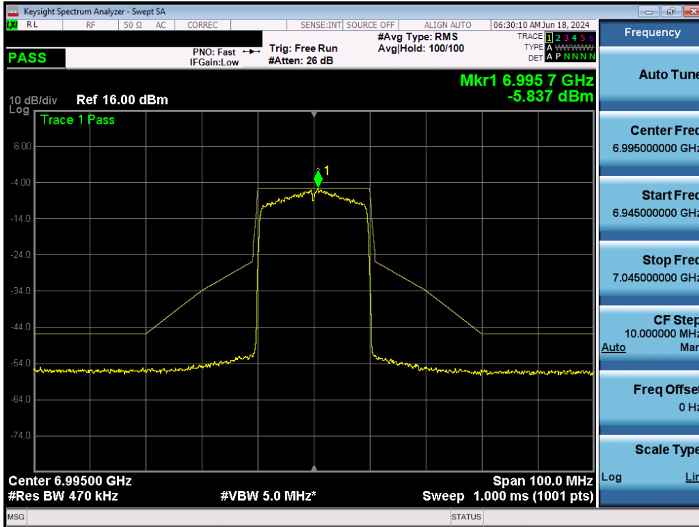
Plot 7-189. In-Band Emissions Plot MIMO ANT2 (20MHz BW 802.11ax (Full Tones) (UNII Band 8) – Ch. 209) - LPI/SP
