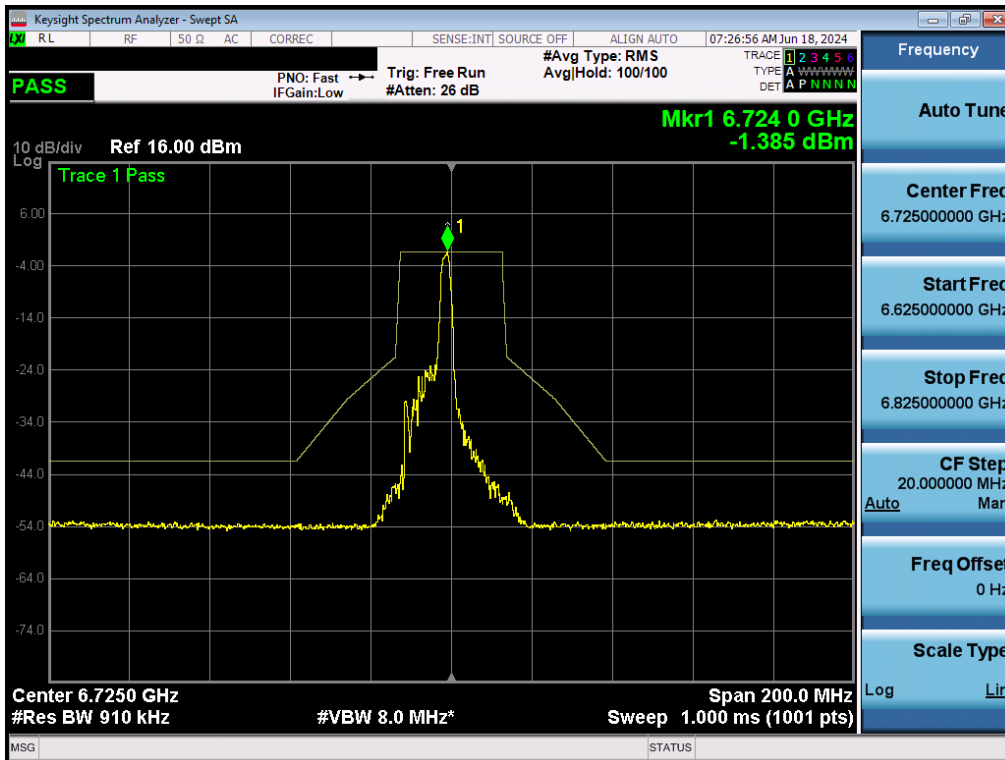
Plot 7-170. In-Band Emissions Plot MIMO ANT2 (40MHz BW 802.11ax (26 Tones) (UNII Band 7) – Ch. 155) - LPI/SP
