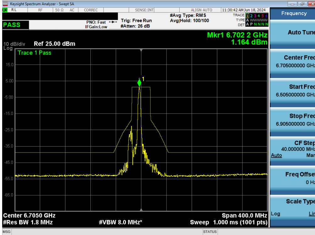
Plot 7-139. In-Band Emissions Plot MIMO ANT1 (80MHz BW 802.11ax (26 Tones) (UNII Band 7) – Ch. 151) - LPI/SP
