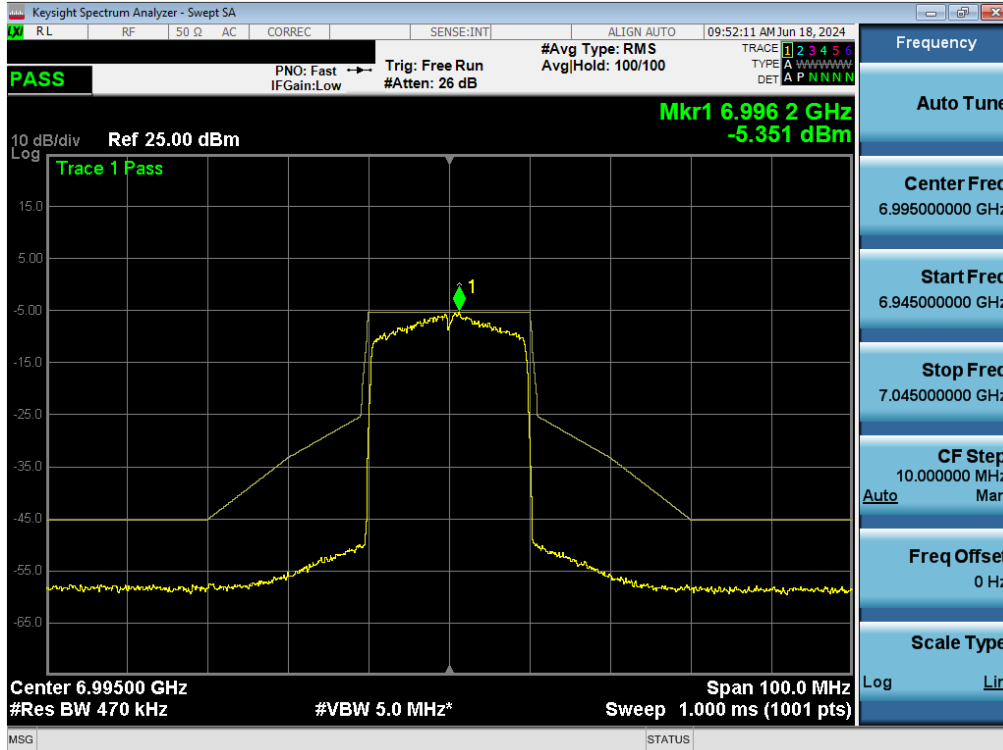
Plot 7-157. In-Band Emissions Plot MIMO ANT1 (20MHz BW 802.11ax (Full Tones) (UNII Band 8) – Ch. 209) - LPI/SP
