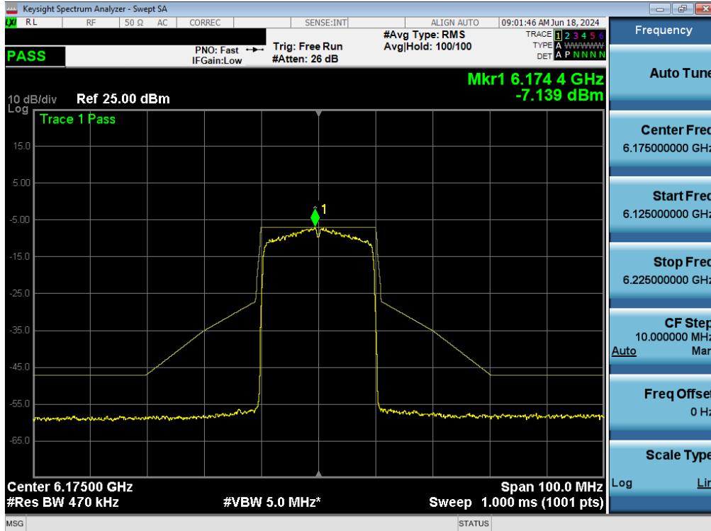
Plot 7-145. In-Band Emissions Plot MIMO ANT1 (20MHz BW 802.11ax (Full Tones) (UNII Band 5) – Ch. 45) - LPI/SP
