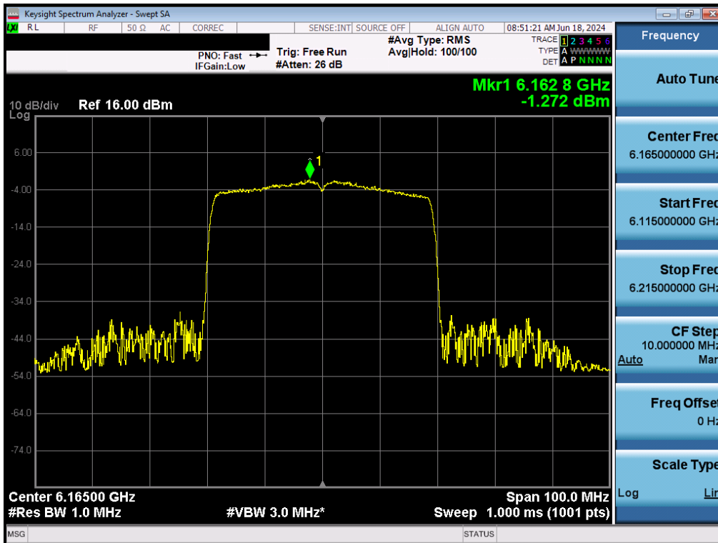
Plot 7-114. Power Spectral Density Plot MIMO ANT2 (40MHz BW 802.11ax (Full Tones) (UNII Band 5) – Ch. 43) - LPI/SP
