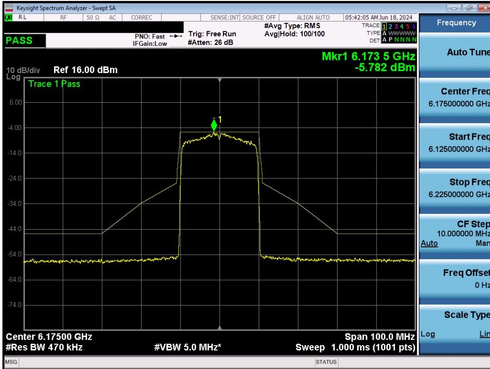
Plot 7-177. In-Band Emissions Plot MIMO ANT2 (20MHz BW 802.11ax (Full Tones) (UNII Band 5) – Ch. 45) - LPI/SP
