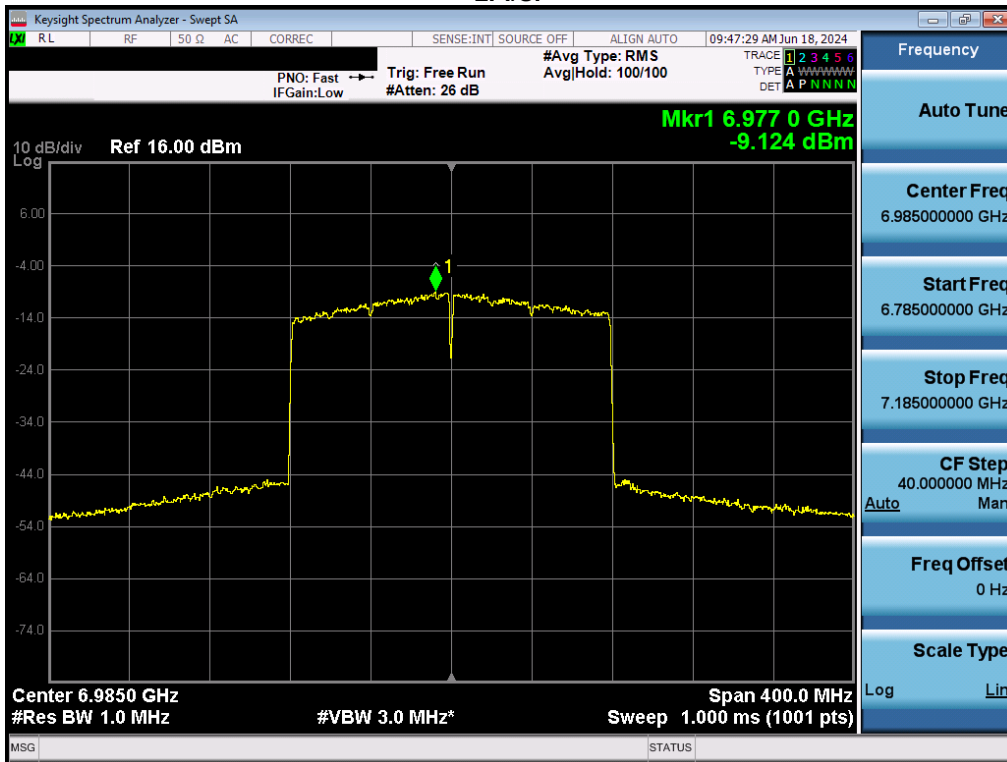
Plot 7-128. Power Spectral Density Plot MIMO ANT2 (160MHz BW 802.11ax (Full Tones) (UNII Band 8) – Ch. 207) - LPI/SP
