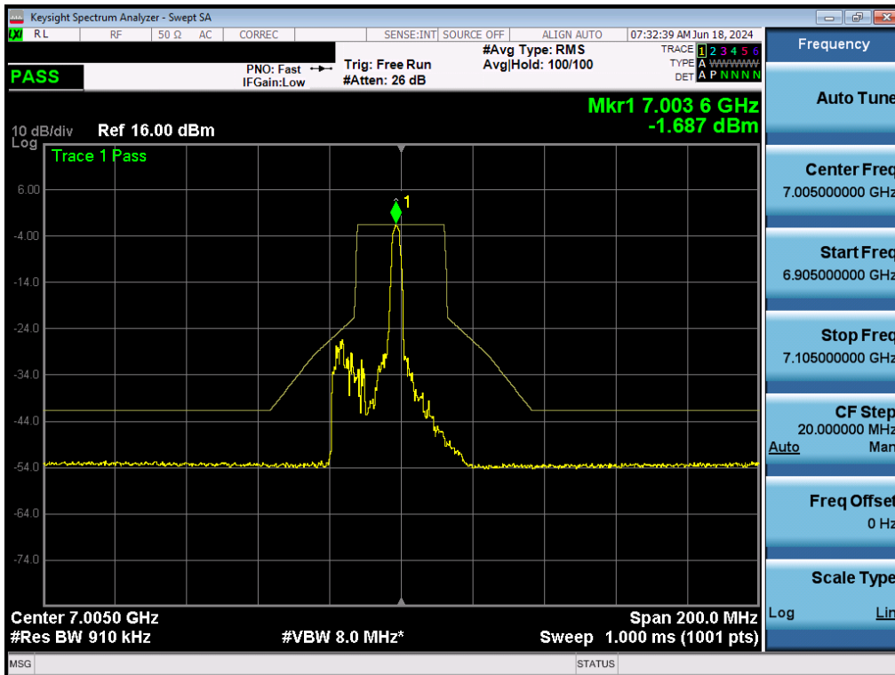
Plot 7-174. In-Band Emissions Plot MIMO ANT2 (40MHz BW 802.11ax (26 Tones) (UNII Band 8) – Ch. 211) - LPI/SP
