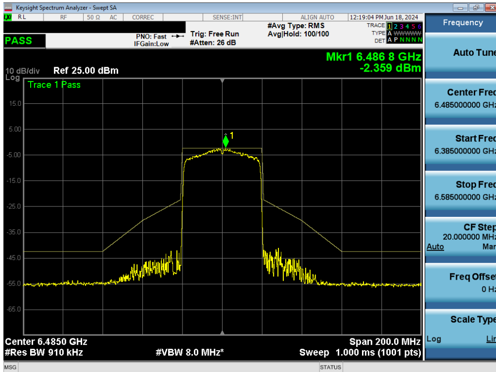
Plot 7-150. In-Band Emissions Plot MIMO ANT1 (40MHz BW 802.11ax (Full Tones) (UNII Band 6) – Ch. 107) - LPI/SP
