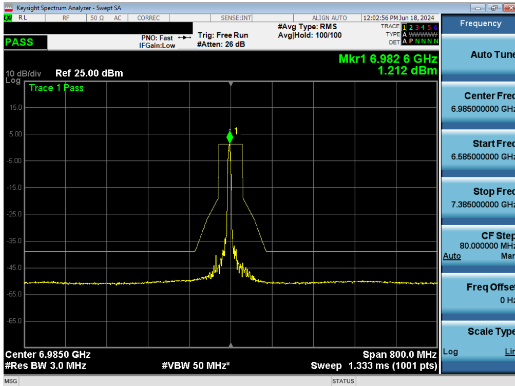
Plot 7-144. In-Band Emissions Plot MIMO ANT1 (160MHz BW 802.11ax (26 Tones) (UNII Band 8) – Ch. 207) - LPI/SP
