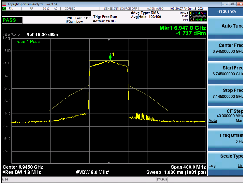
Plot 7-191. In-Band Emissions Plot MIMO ANT2 (80MHz BW 802.11ax (Full Tones) (UNII Band 8) – Ch. 199) - LPI/SP
