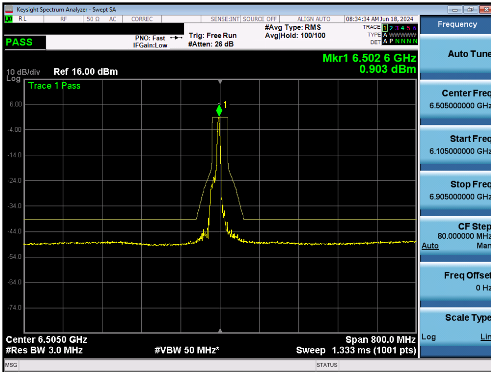
Plot 7-168. In-Band Emissions Plot MIMO ANT2 (160MHz BW 802.11ax (26 Tones) (UNII Band 6) – Ch. 111) - LPI/SP
