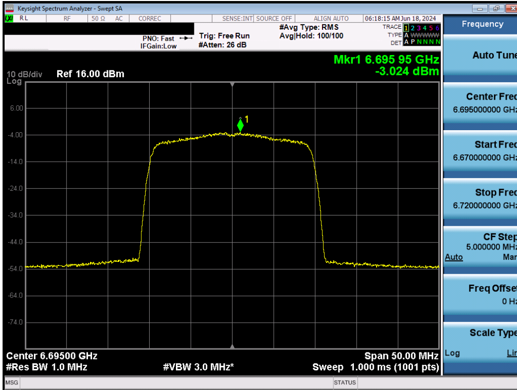
Plot 7-121. Power Spectral Density Plot MIMO ANT2 (20MHz BW 802.11ax (Full Tones) (UNII Band 7) – Ch. 149) - LPI/SP
