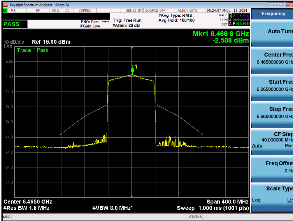
Plot 7-183. In-Band Emissions Plot MIMO ANT2 (80MHz BW 802.11ax (Full Tones) (UNII Band 6) – Ch. 103) - LPI/SP
