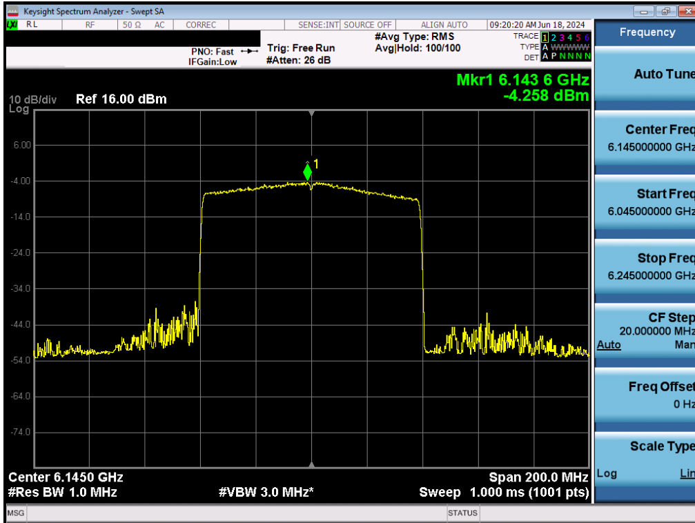
Plot 7-115. Power Spectral Density Plot MIMO ANT2 (80MHz BW 802.11ax (Full Tones) (UNII Band 5) – Ch. 39) - LPI/SP
