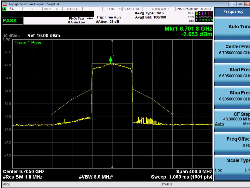
Plot 7-187. In-Band Emissions Plot MIMO ANT2 (80MHz BW 802.11ax (Full Tones) (UNII Band 7) – Ch. 151) - LPI/SP
