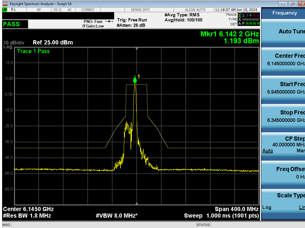
Plot 7-131. In-Band Emissions Plot MIMO ANT1 (80MHz BW 802.11ax (26 Tones) (UNII Band 5) – Ch. 39) - LPI/SP
