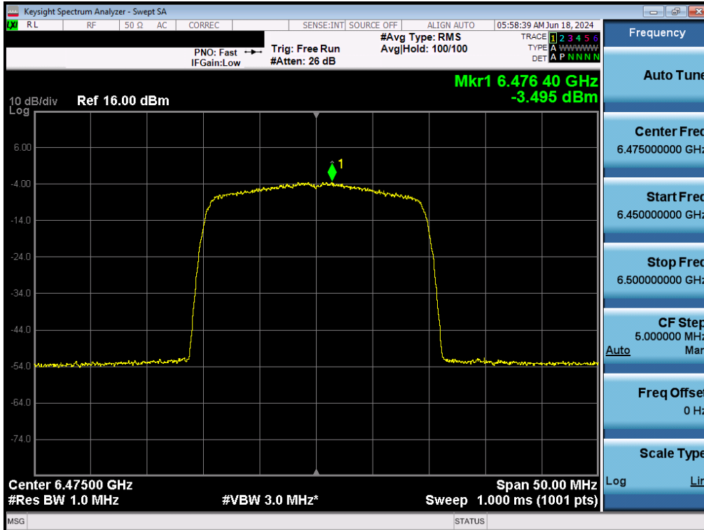
Plot 7-117. Power Spectral Density Plot MIMO ANT2 (20MHz BW 802.11ax (Full Tones) (UNII Band 6) – Ch. 105) - LPI/SP
