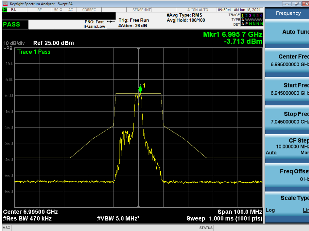
Plot 7-141. In-Band Emissions Plot MIMO ANT1 (20MHz BW 802.11ax (26 Tones) (UNII Band 8) – Ch. 209) - LPI/SP
