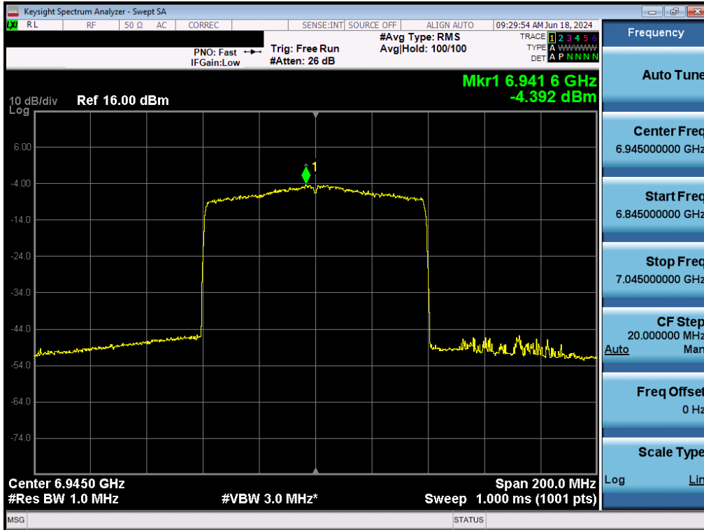
Plot 7-127. Power Spectral Density Plot MIMO ANT2 (80MHz BW 802.11ax (Full Tones) (UNII Band 8) – Ch. 199) - LPI/SP
