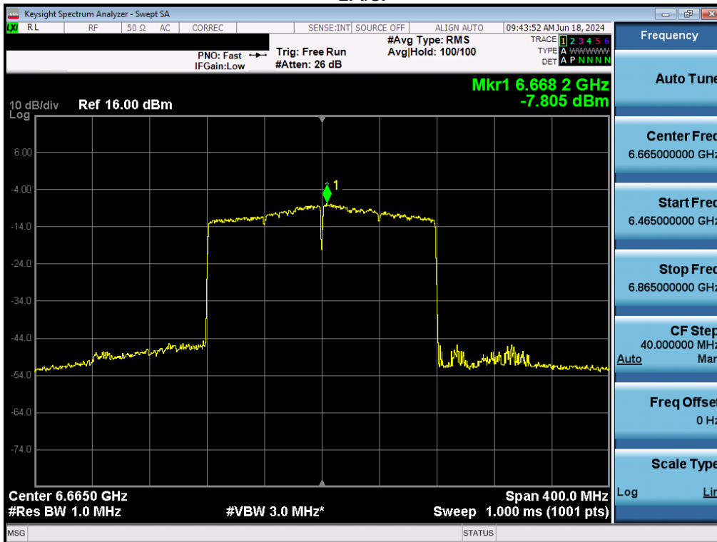
Plot 7-124. Power Spectral Density Plot MIMO ANT2 (160MHz BW 802.11ax (Full Tones) (UNII Band 7) – Ch. 143) - LPI/SP
