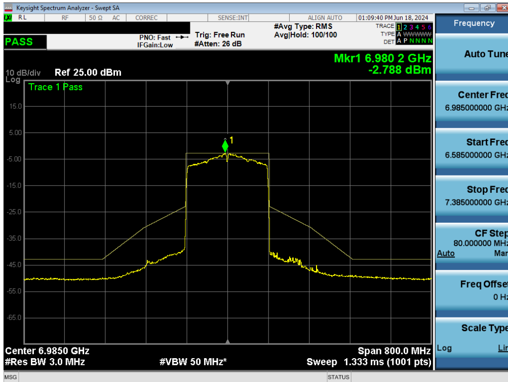
Plot 7-160. In-Band Emissions Plot MIMO ANT1 (160MHz BW 802.11ax (Full Tones) (UNII Band 8) – Ch. 207) - LPI/SP
