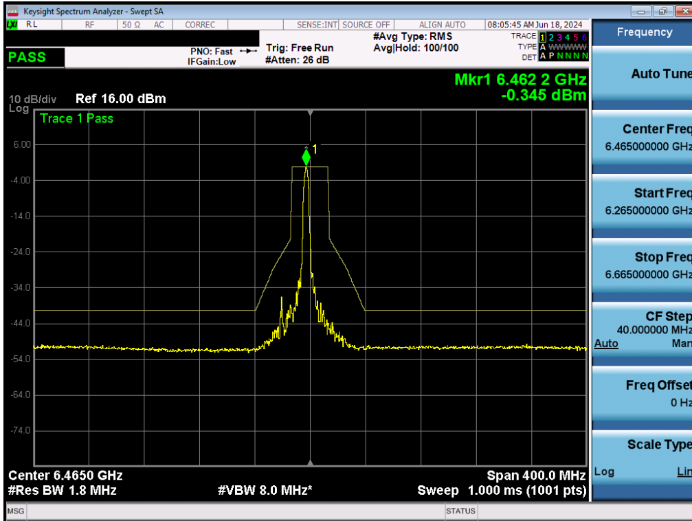
Plot 7-167. In-Band Emissions Plot MIMO ANT2 (80MHz BW 802.11ax (26 Tones) (UNII Band 6) – Ch. 103) - LPI/SP
