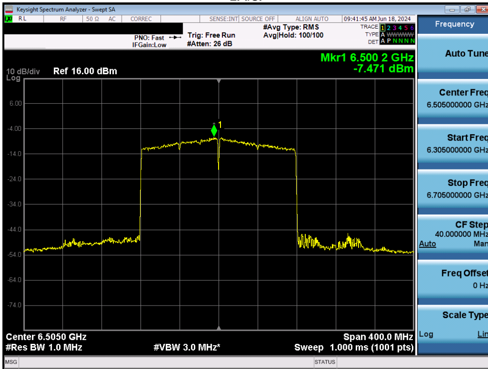
Plot 7-120. Power Spectral Density Plot MIMO ANT2 (160MHz BW 802.11ax (Full Tones) (UNII Band 6) – Ch. 111) - LPI/SP
