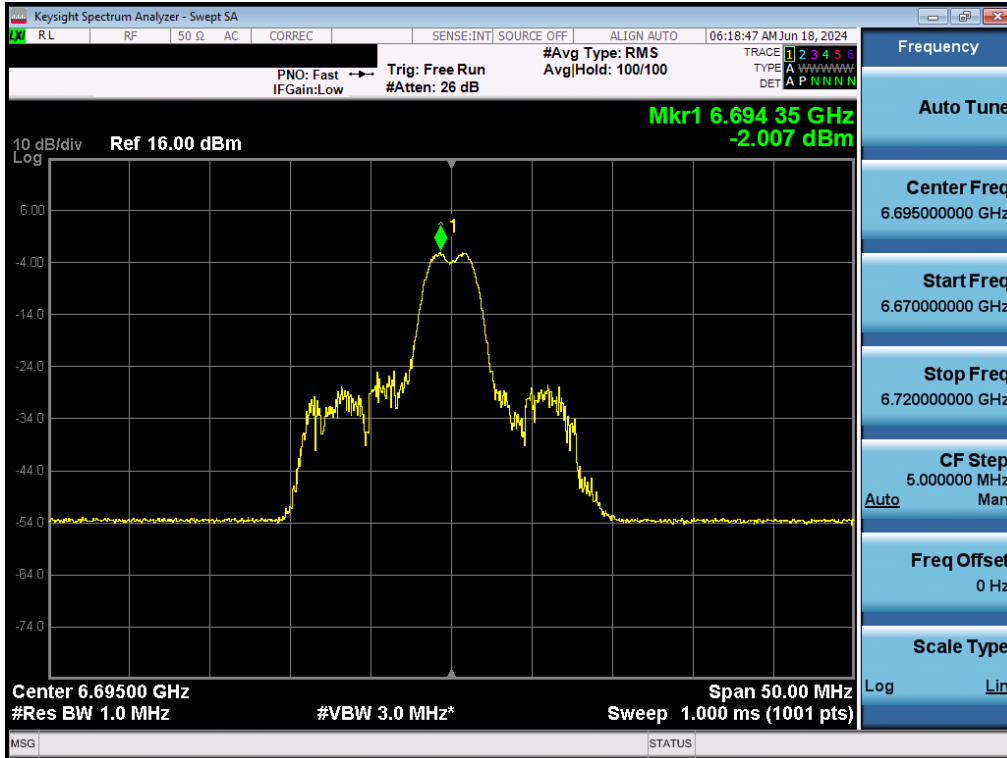
Plot 7-105. Power Spectral Density Plot MIMO ANT2 (20MHz BW 802.11ax (26 Tones) (UNII Band 7) – Ch. 149) - LPI/SP
