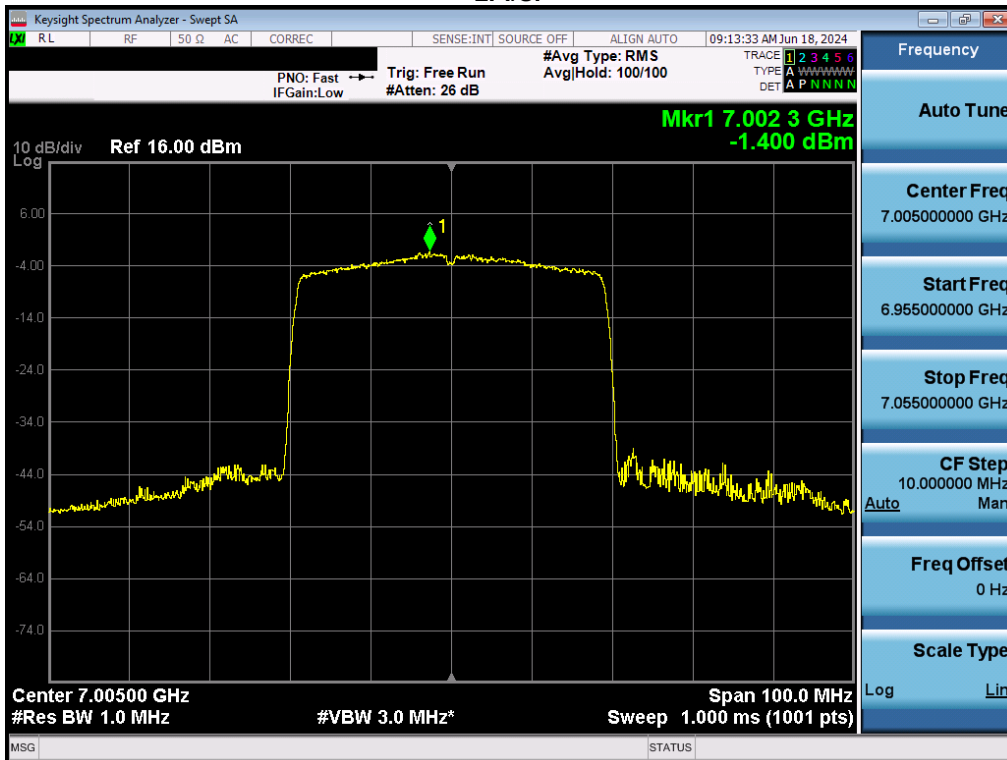
Plot 7-126. Power Spectral Density Plot MIMO ANT2 (40MHz BW 802.11ax (Full Tones) (UNII Band 8) – Ch. 211) - LPI/SP
