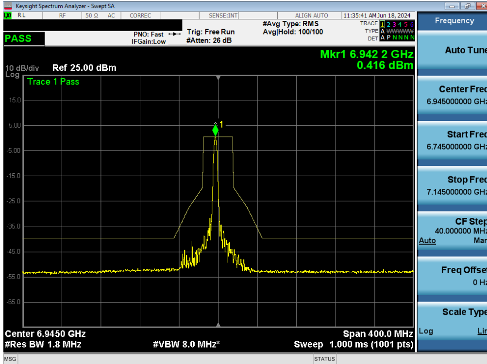
Plot 7-143. In-Band Emissions Plot MIMO ANT1 (80MHz BW 802.11ax (26 Tones) (UNII Band 8) – Ch. 199) - LPI/SP
