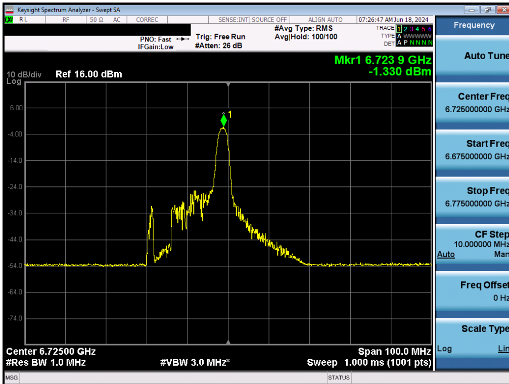
Plot 7-106. Power Spectral Density Plot MIMO ANT2 (40MHz BW 802.11ax (26 Tones) (UNII Band 7) – Ch. 155) - LPI/SP
