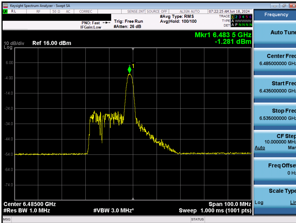
Plot 7-102. Power Spectral Density Plot MIMO ANT2 (40MHz BW 802.11ax (26 Tones) (UNII Band 6) – Ch. 107) - LPI/SP
