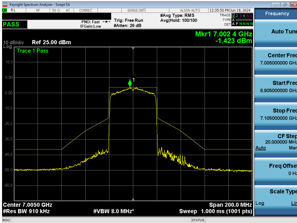
Plot 7-158. In-Band Emissions Plot MIMO ANT1 (40MHz BW 802.11ax (Full Tones) (UNII Band 8) – Ch. 211) - LPI/SP
