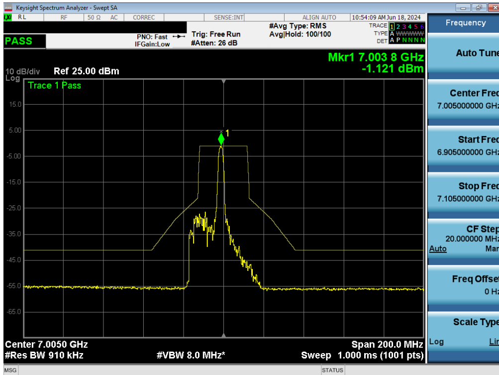
Plot 7-142. In-Band Emissions Plot MIMO ANT1 (40MHz BW 802.11ax (26 Tones) (UNII Band 8) – Ch. 211) - LPI/SP
