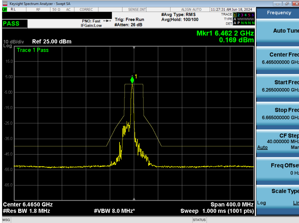
Plot 7-135. In-Band Emissions Plot MIMO ANT1 (80MHz BW 802.11ax (26 Tones) (UNII Band 6) – Ch. 103) - LPI/SP
