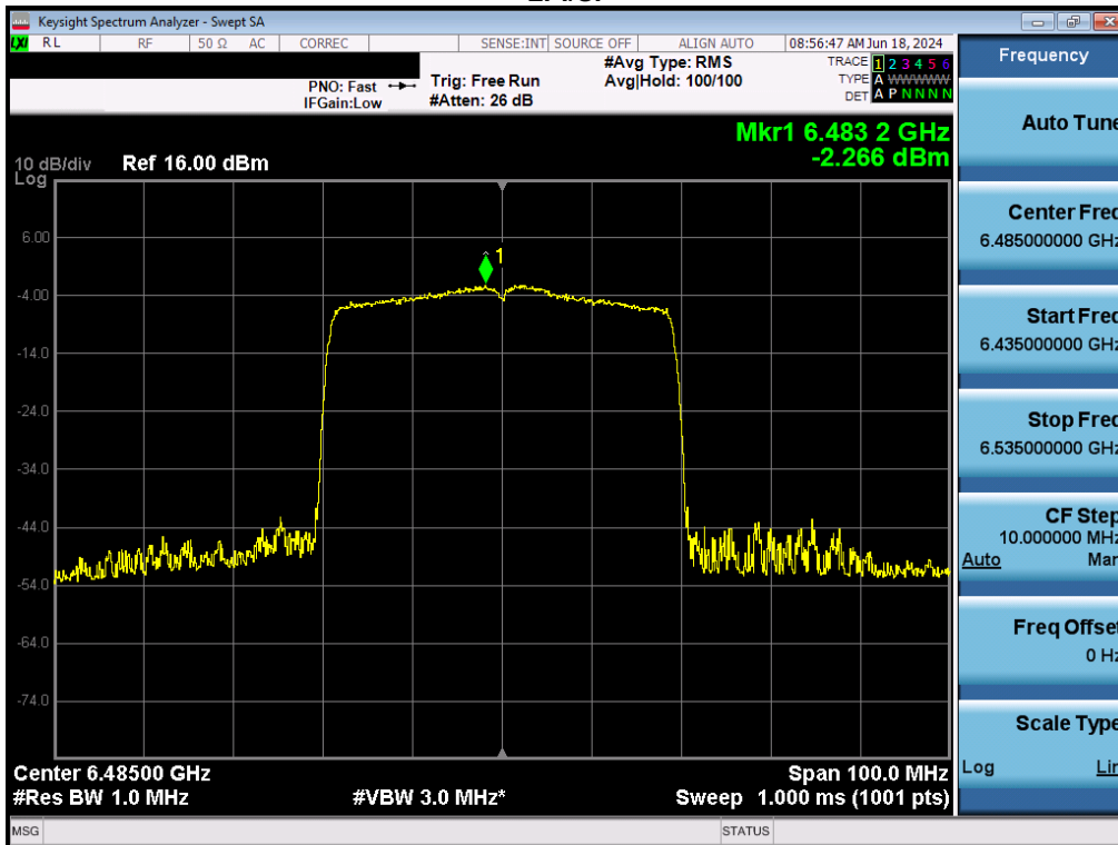
Plot 7-118. Power Spectral Density Plot MIMO ANT2 (40MHz BW 802.11ax (Full Tones) (UNII Band 6) – Ch. 107) - LPI/SP
