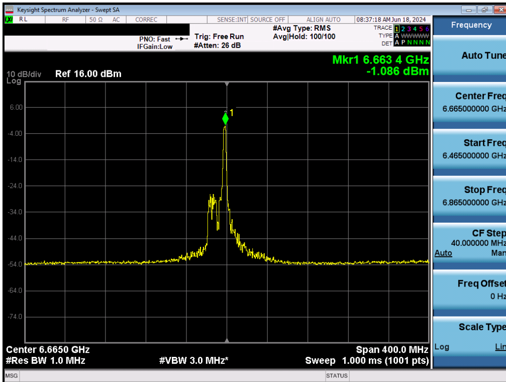
Plot 7-108. Power Spectral Density Plot MIMO ANT2 (160MHz BW 802.11ax (26 Tones) (UNII Band 7) – Ch. 143) - LPI/SP
