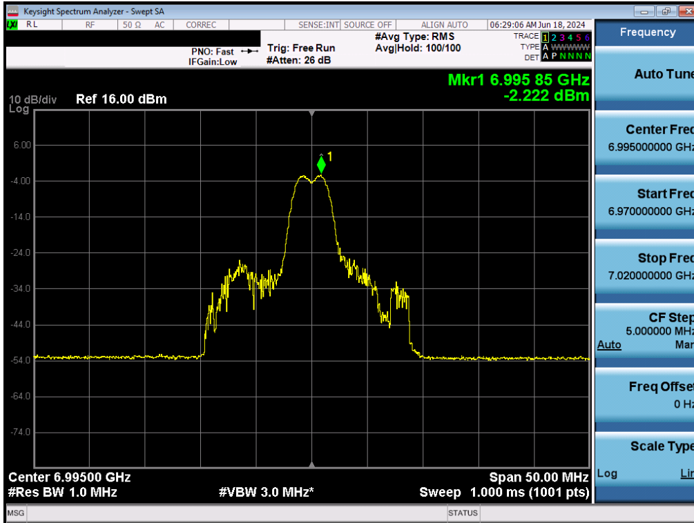
Plot 7-109. Power Spectral Density Plot MIMO ANT2 (20MHz BW 802.11ax (26 Tones) (UNII Band 8) – Ch. 209) - LPI/SP
