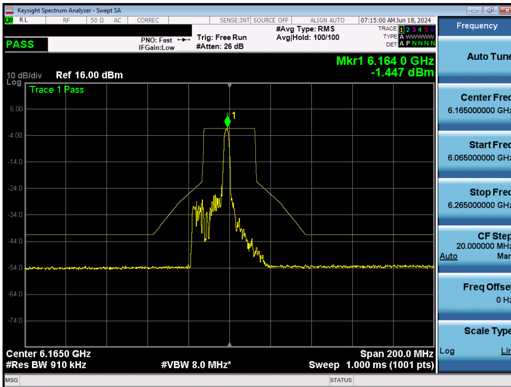
Plot 7-162. In-Band Emissions Plot MIMO ANT2 (40MHz BW 802.11ax (26 Tones) (UNII Band 5) – Ch. 43) - LPI/SP
