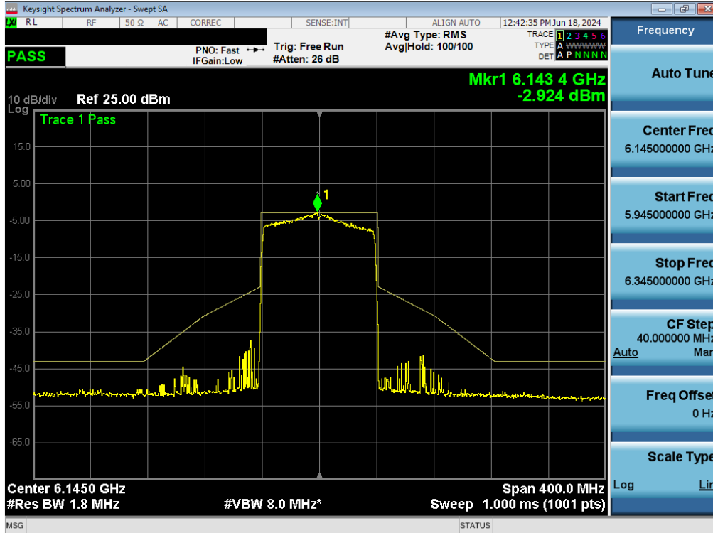
Plot 7-147. In-Band Emissions Plot MIMO ANT1 (80MHz BW 802.11ax (Full Tones) (UNII Band 5) – Ch. 39) - LPI/SP
