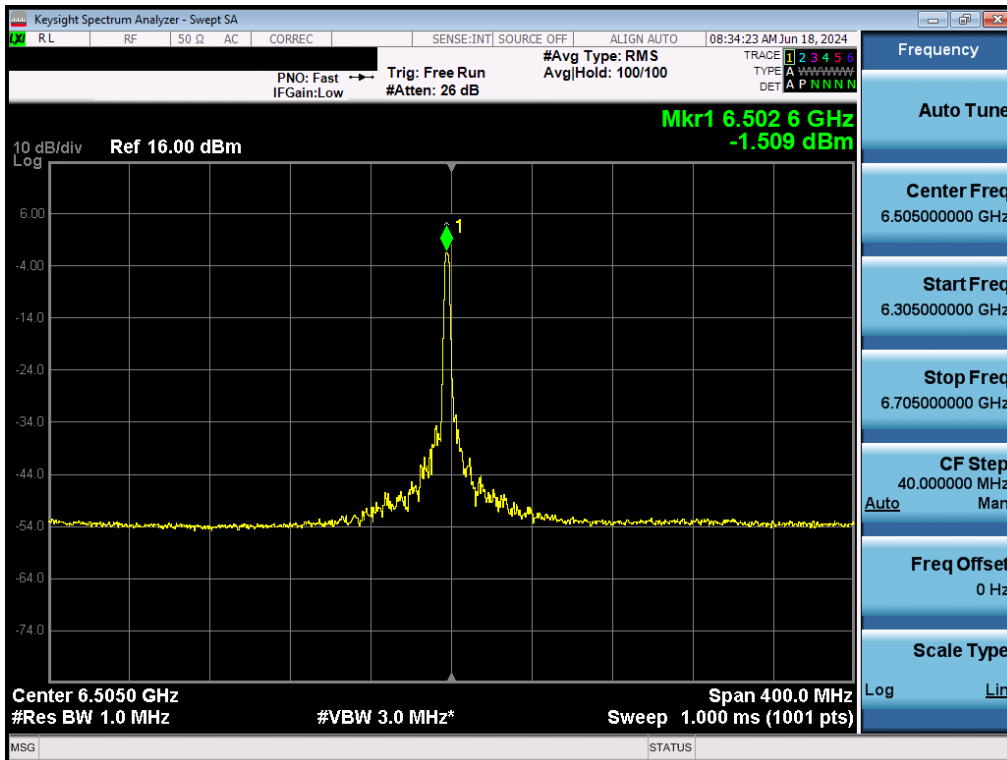
Plot 7-104. Power Spectral Density Plot MIMO ANT2 (160MHz BW 802.11ax (26 Tones) (UNII Band 6) – Ch. 111) - LPI/SP
