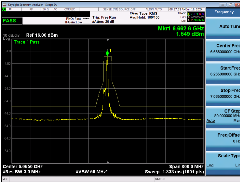
Plot 7-172. In-Band Emissions Plot MIMO ANT2 (160MHz BW 802.11ax (26 Tones) (UNII Band 7) – Ch. 143) - LPI/SP
