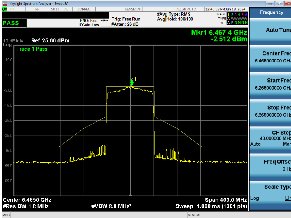
Plot 7-151. In-Band Emissions Plot MIMO ANT1 (80MHz BW 802.11ax (Full Tones) (UNII Band 6) – Ch. 103) - LPI/SP
