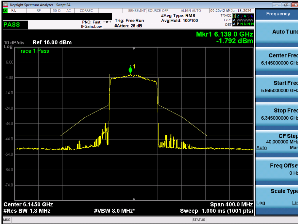
Plot 7-179. In-Band Emissions Plot MIMO ANT2 (80MHz BW 802.11ax (Full Tones) (UNII Band 5) – Ch. 39) - LPI/SP
