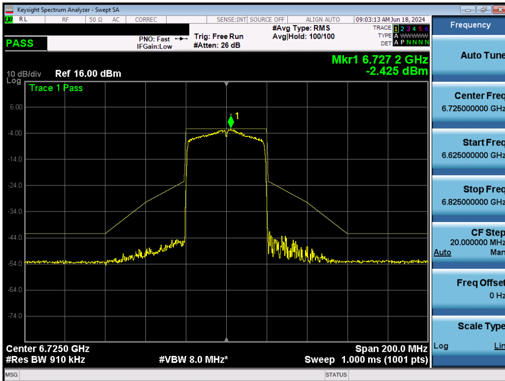
Plot 7-186. In-Band Emissions Plot MIMO ANT2 (40MHz BW 802.11ax (Full Tones) (UNII Band 7) – Ch. 155) - LPI/SP
