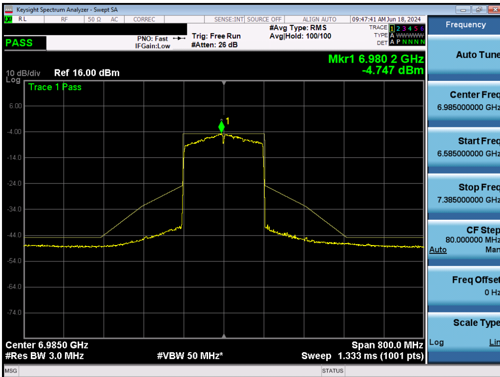
Plot 7-192. In-Band Emissions Plot MIMO ANT2 (160MHz BW 802.11ax (Full Tones) (UNII Band 8) – Ch. 207) - LPI/SP
