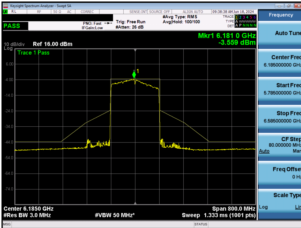
Plot 7-180. In-Band Emissions Plot MIMO ANT2 (160MHz BW 802.11ax (Full Tones) (UNII Band 5) – Ch. 47) - LPI/SP
