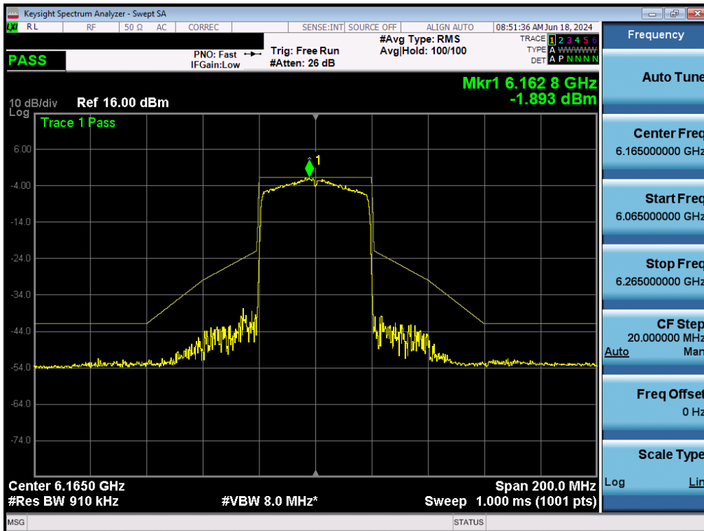
Plot 7-178. In-Band Emissions Plot MIMO ANT2 (40MHz BW 802.11ax (Full Tones) (UNII Band 5) – Ch. 43) - LPI/SP
