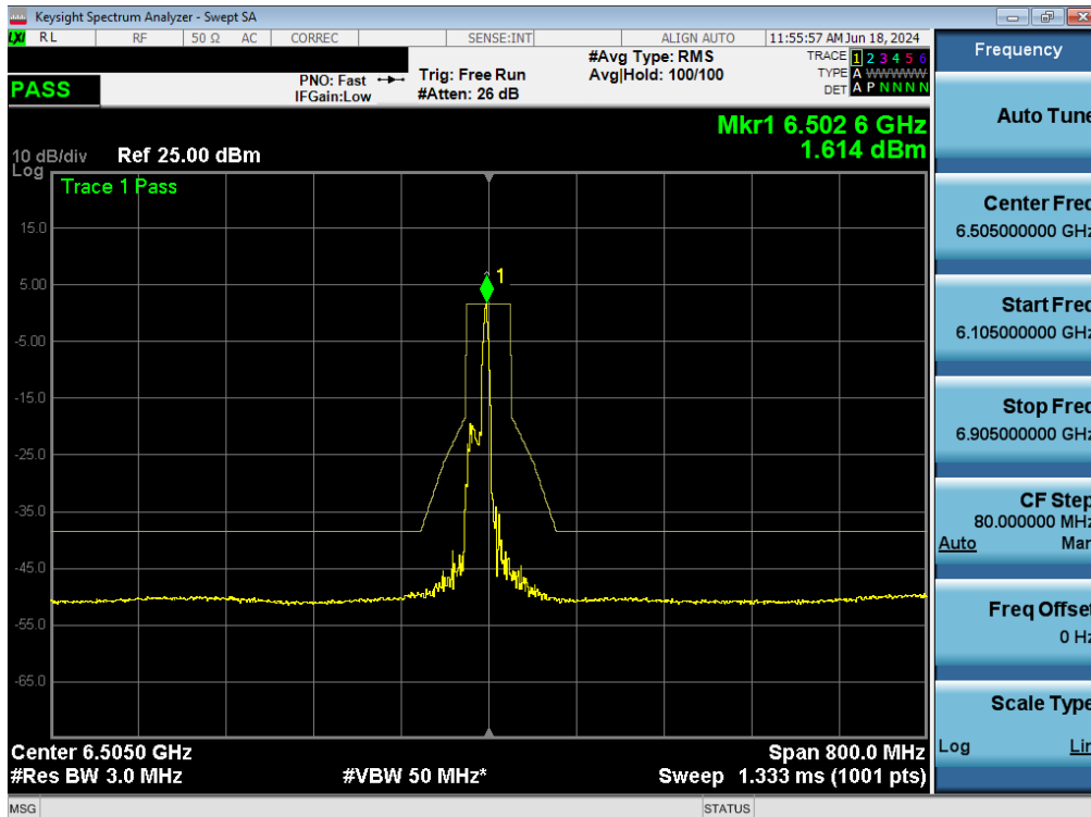
Plot 7-136. In-Band Emissions Plot MIMO ANT1 (160MHz BW 802.11ax (26 Tones) (UNII Band 6) – Ch. 111) - LPI/SP
