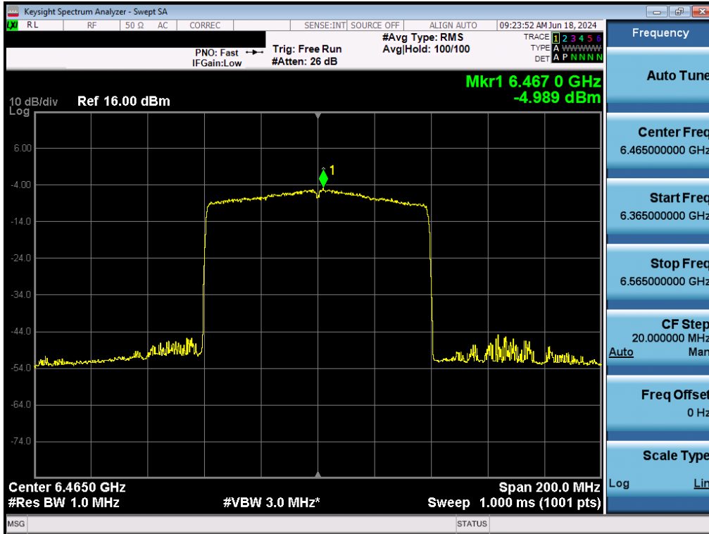
Plot 7-119. Power Spectral Density Plot MIMO ANT2 (80MHz BW 802.11ax (Full Tones) (UNII Band 6) – Ch. 103) - LPI/SP
