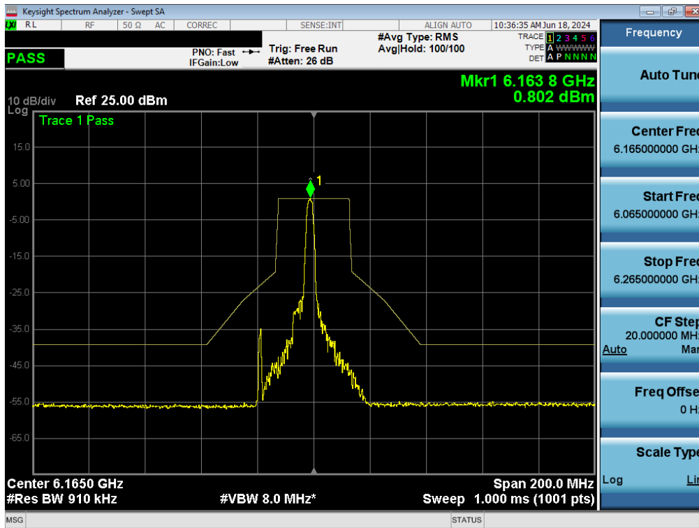
Plot 7-130. In-Band Emissions Plot MIMO ANT1 (40MHz BW 802.11ax (26 Tones) (UNII Band 5) – Ch. 43) - LPI/SP
