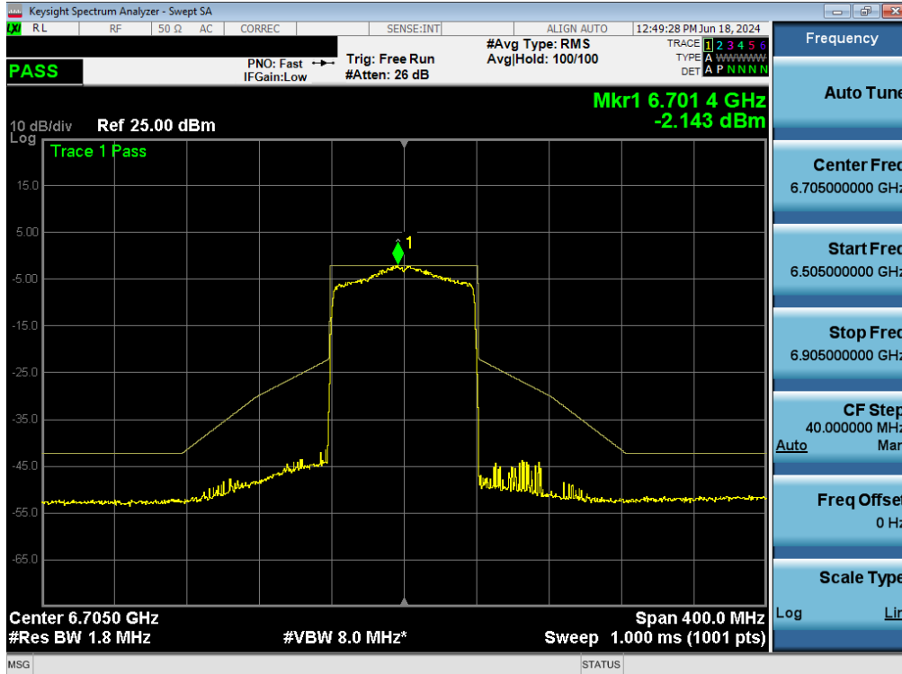
Plot 7-155. In-Band Emissions Plot MIMO ANT1 (80MHz BW 802.11ax (Full Tones) (UNII Band 7) – Ch. 151) – LPI/SP
