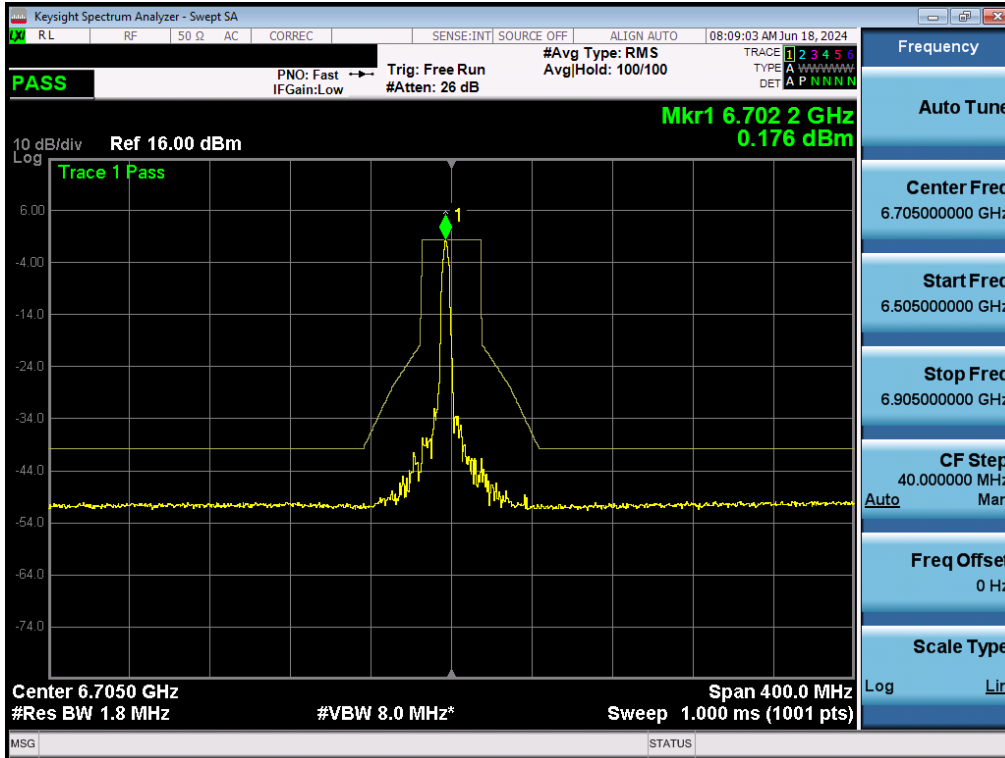
Plot 7-171. In-Band Emissions Plot MIMO ANT2 (80MHz BW 802.11ax (26 Tones) (UNII Band 7) – Ch. 151) - LPI/SP
