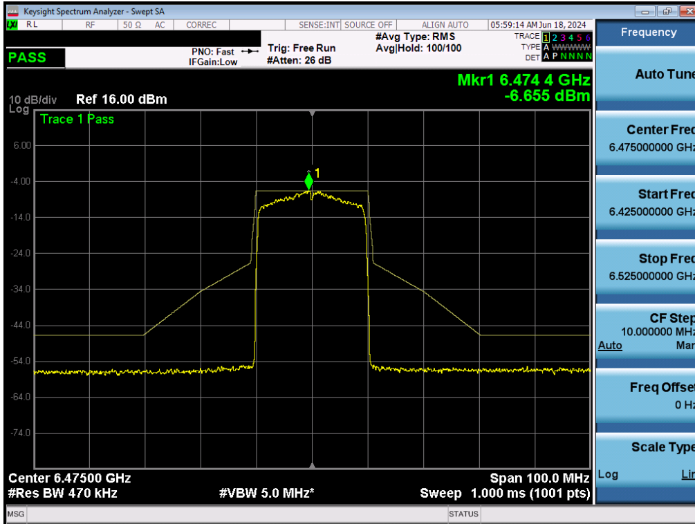
Plot 7-181. In-Band Emissions Plot MIMO ANT2 (20MHz BW 802.11ax (Full Tones) (UNII Band 6) – Ch. 105) - LPI/SP
