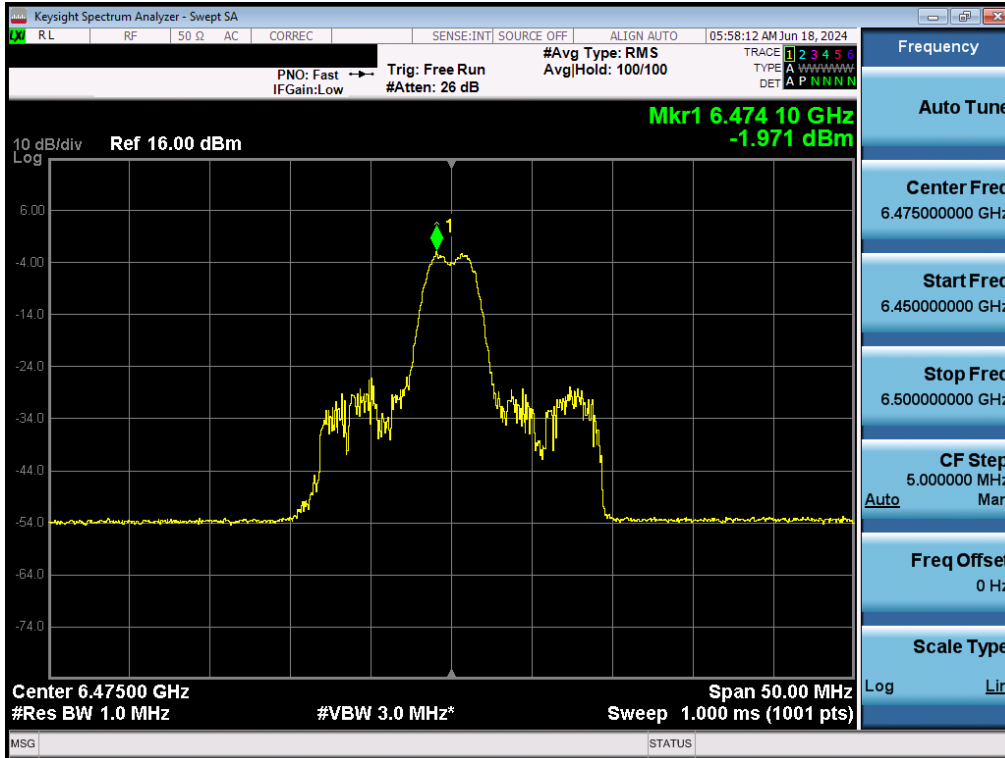
Plot 7-101. Power Spectral Density Plot MIMO ANT2 (20MHz BW 802.11ax (26 Tones) (UNII Band 6) – Ch. 105) - LPI/SP
