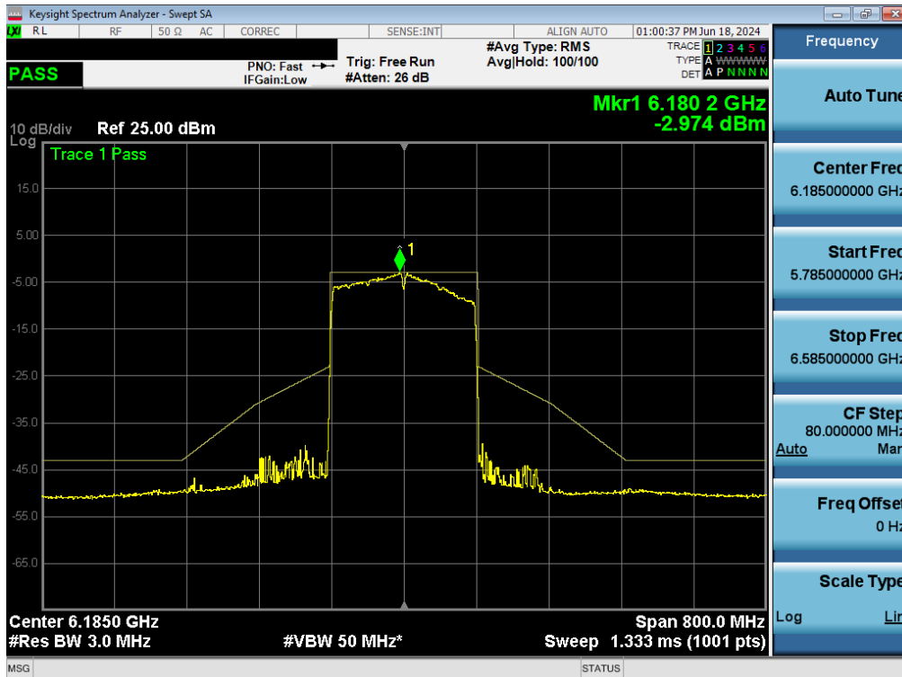
Plot 7-148. In-Band Emissions Plot MIMO ANT1 (160MHz BW 802.11ax (Full Tones) (UNII Band 5) – Ch. 47) - LPI/SP
