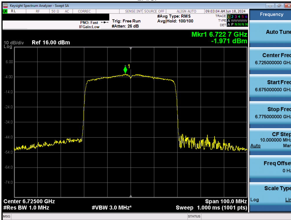
Plot 7-122. Power Spectral Density Plot MIMO ANT2 (40MHz BW 802.11ax (Full Tones) (UNII Band 7) – Ch. 155) - LPI/SP
