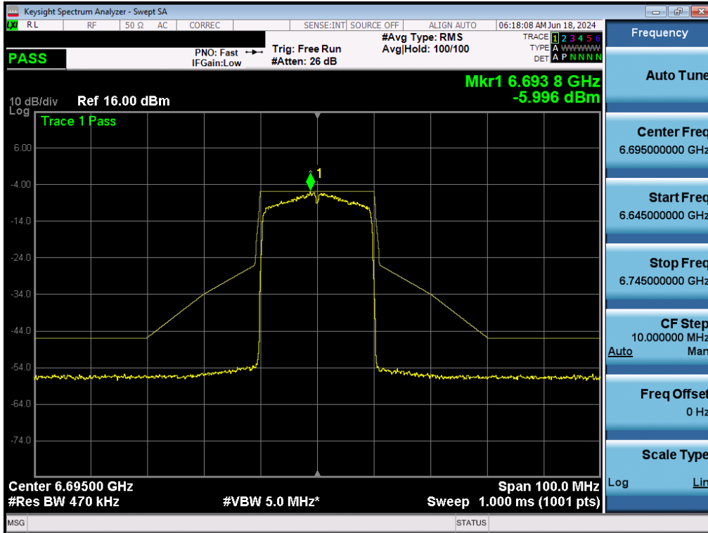
Plot 7-185. In-Band Emissions Plot MIMO ANT2 (20MHz BW 802.11ax (Full Tones) (UNII Band 7) – Ch. 149) - LPI/SP
