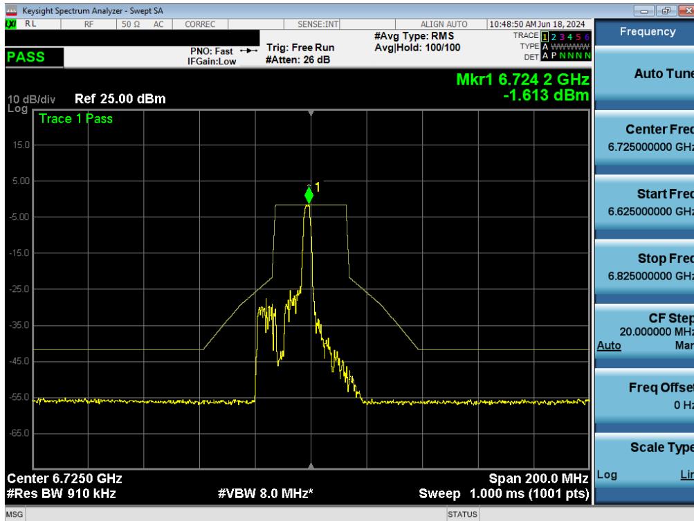
Plot 7-138. In-Band Emissions Plot MIMO ANT1 (40MHz BW 802.11ax (26 Tones) (UNII Band 7) – Ch. 155) - LPI/SP
