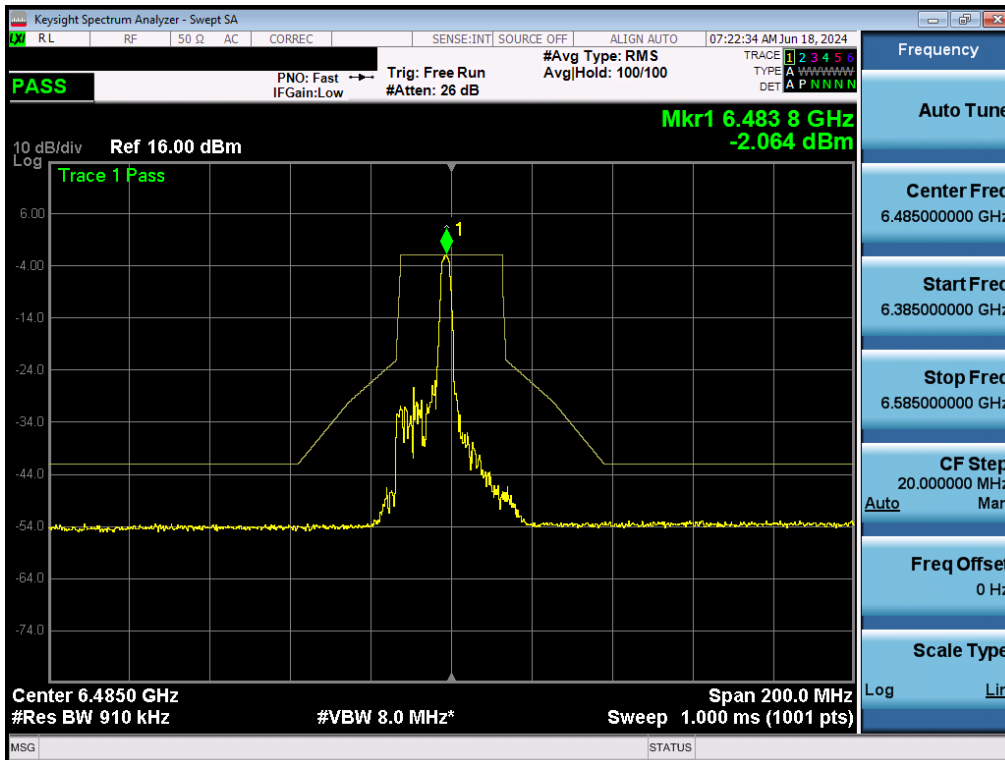
Plot 7-166. In-Band Emissions Plot MIMO ANT2 (40MHz BW 802.11ax (26 Tones) (UNII Band 6) – Ch. 107) - LPI/SP
