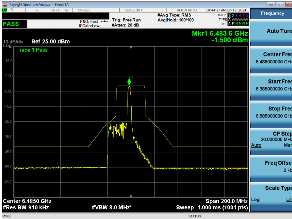
Plot 7-134. In-Band Emissions Plot MIMO ANT1 (40MHz BW 802.11ax (26 Tones) (UNII Band 6) – Ch. 107) - LPI/SP
