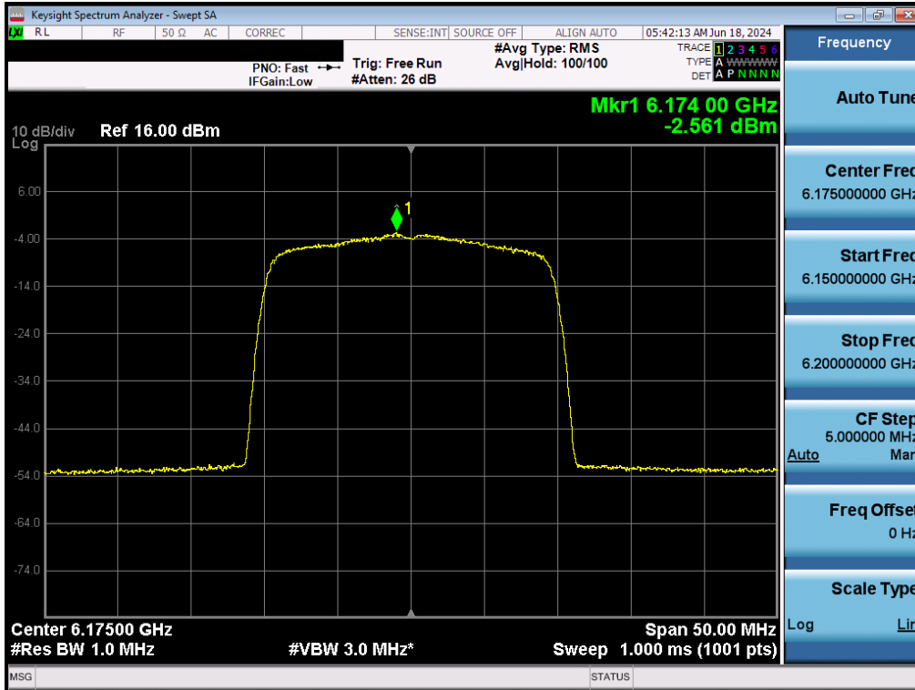
Plot 7-113. Power Spectral Density Plot MIMO ANT2 (20MHz BW 802.11ax (Full Tones) (UNII Band 5) – Ch. 45) - LPI/SP
