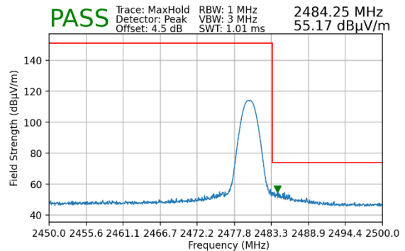
Plot 7-94. Radiated Restricted Upper Band Edge Measurement (Peak) – Ant2
