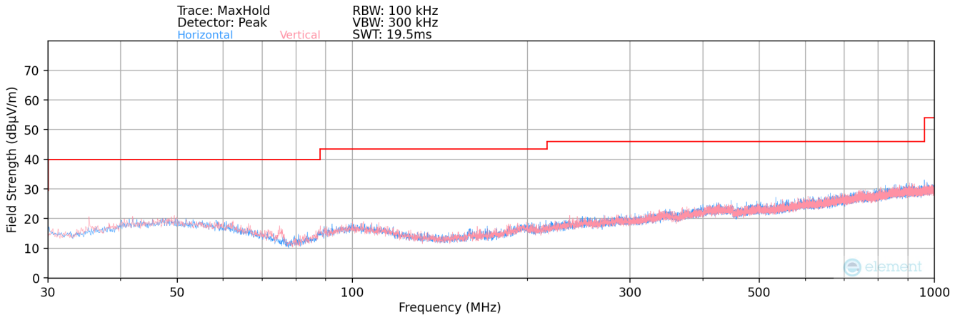
Plot 7-153. Radiated Spurious Plot below 1GHz SISO ANT1
