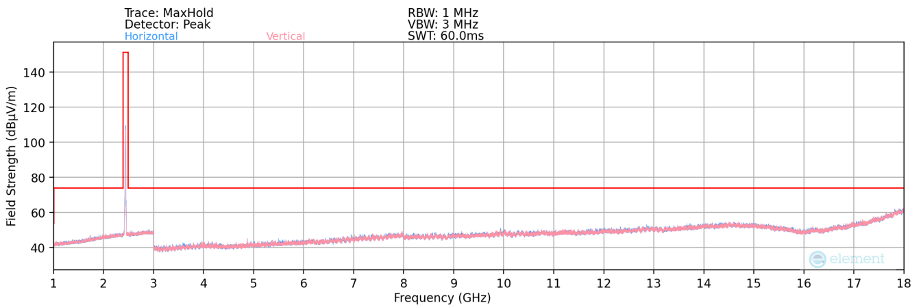
Plot 7-155. Radiated Spurious Plot above 1GHz SISO ANT1 (802.11b – Ch. 6)
