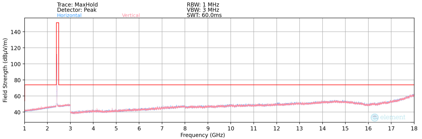
Plot 7-164. Radiated Spurious Plot above 1GHz MIMO (802.11b – Ch. 1)
