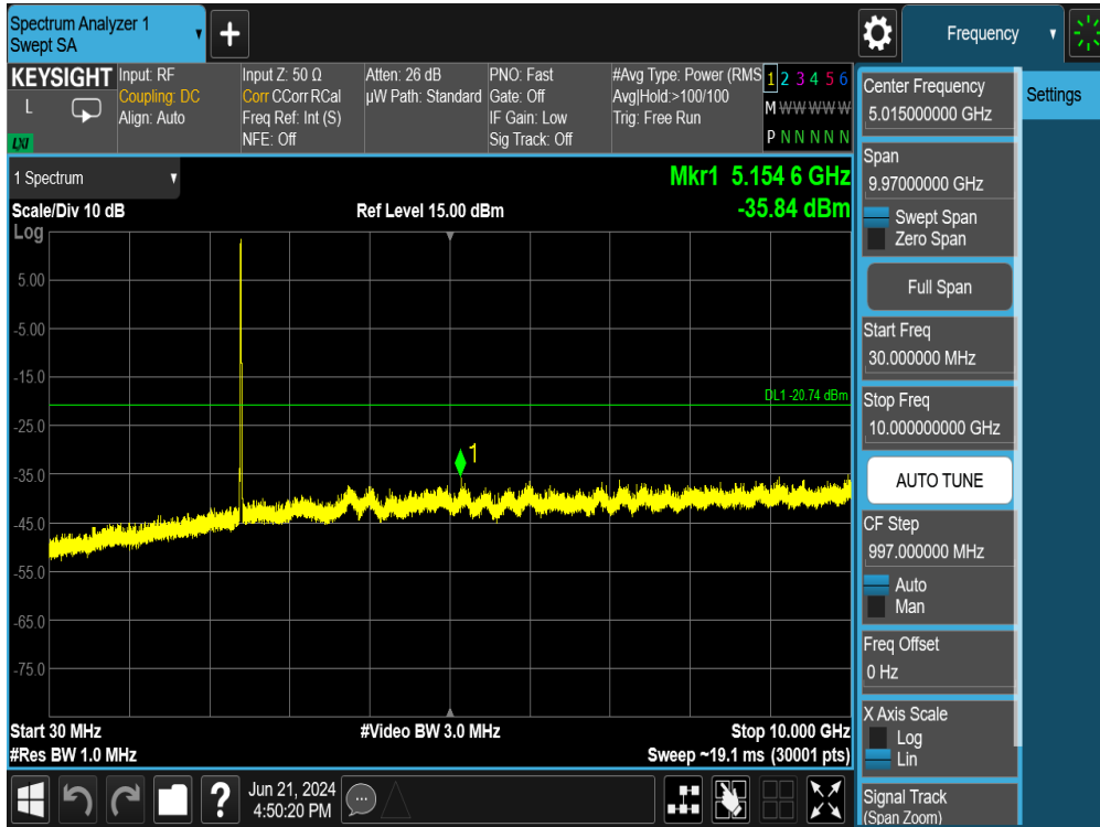
Plot 7-147. Conducted Spurious Plot MIMO ANT2 (802.11b – Ch. 1)
