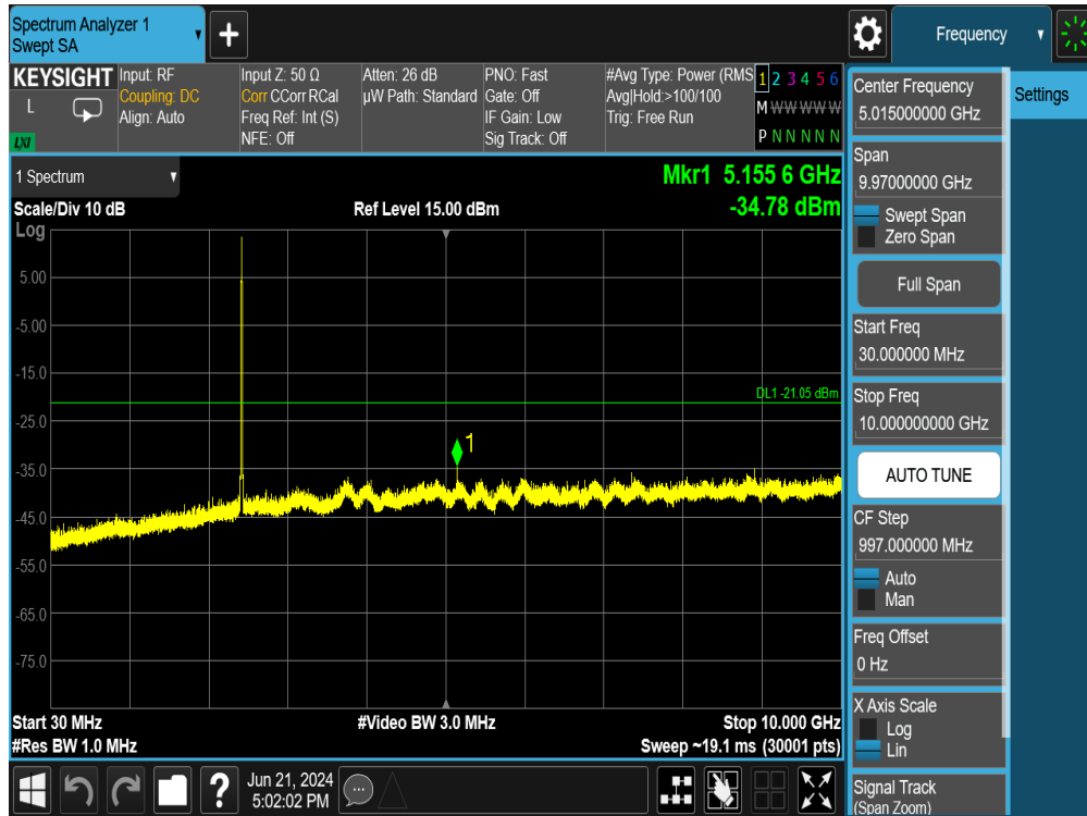
Plot 7-143. Conducted Spurious Plot MIMO ANT1 (802.11b – Ch. 6)
