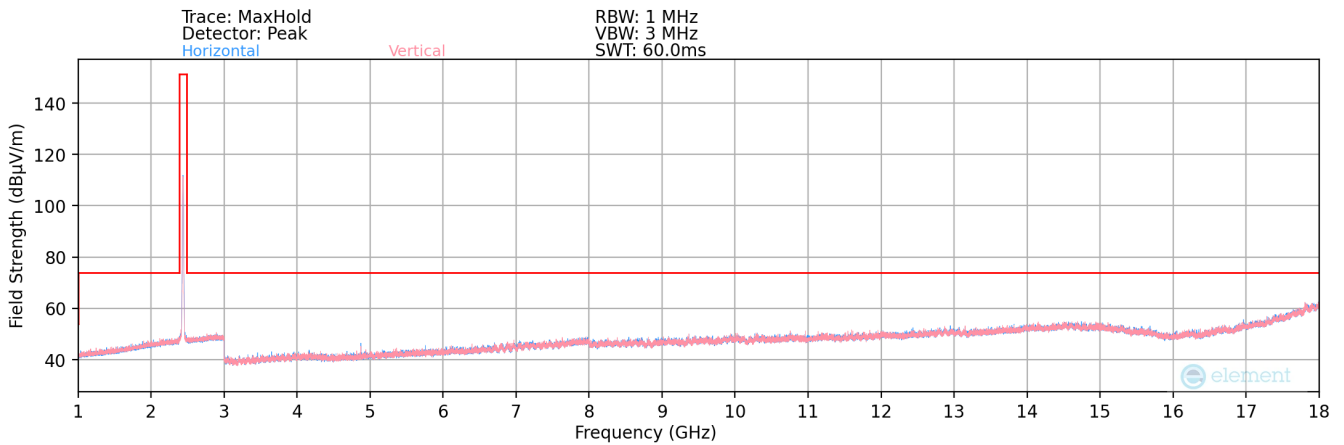
Plot 7-165. Radiated Spurious Plot above 1GHz MIMO (802.11b – Ch. 6)
