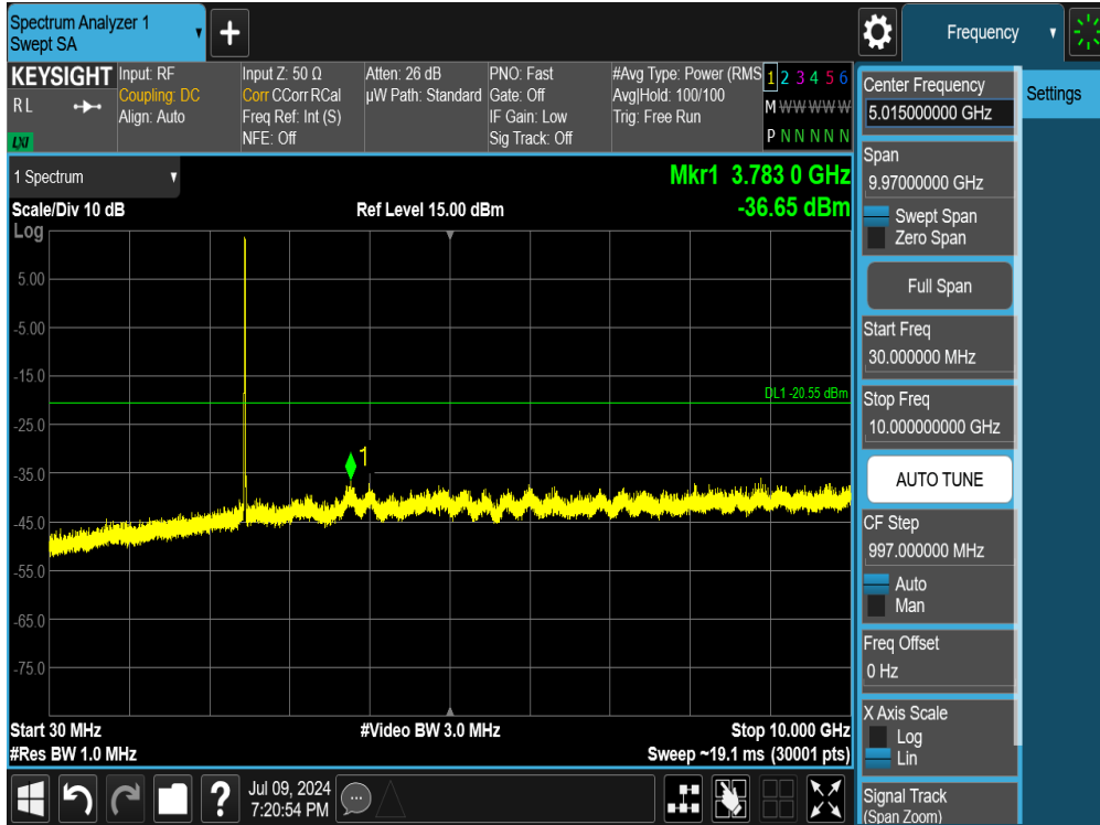
Plot 7-133. Conducted Spurious Plot SISO ANT1 (802.11b – Ch. 11)
