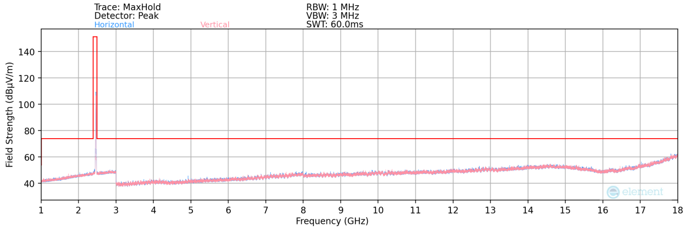
Plot 7-156. Radiated Spurious Plot above 1GHz SISO ANT1 (802.11b – Ch. 11)
