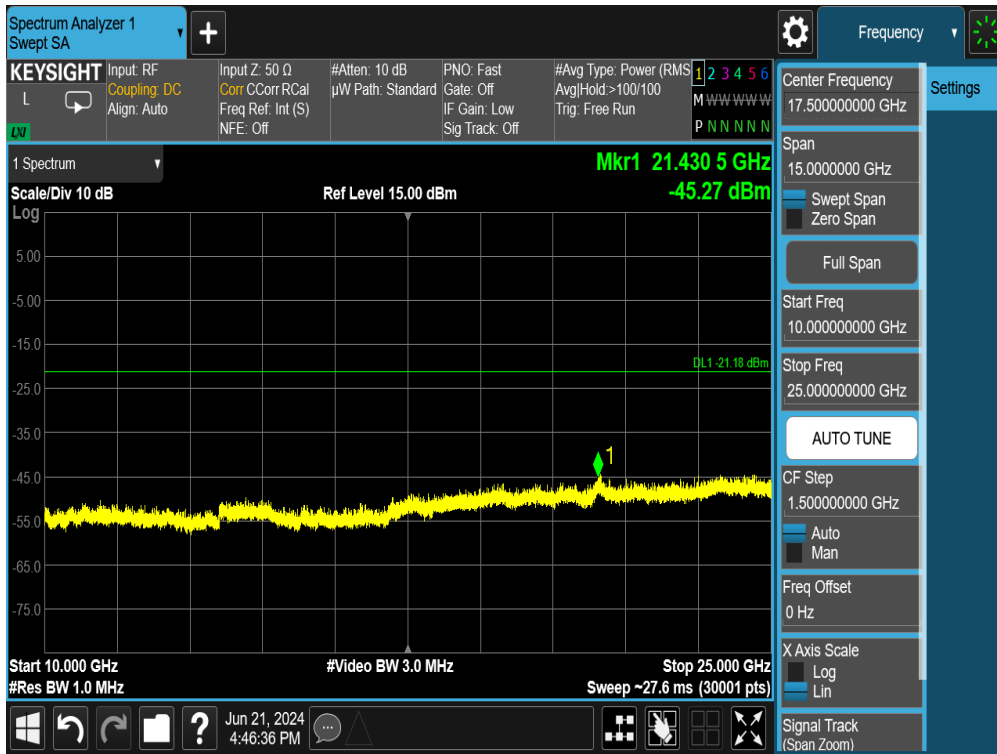
Plot 7-138. Conducted Spurious Plot SISO ANT2 (802.11b – Ch. 6)
