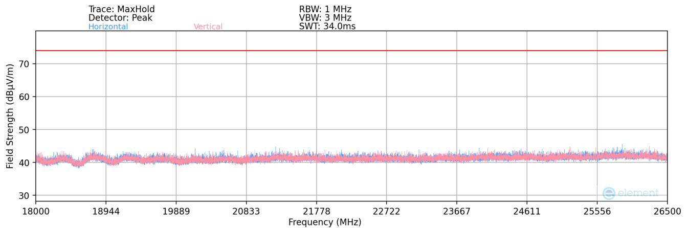
Plot 7-162. Radiated Spurious Plot above 18GHz SISO ANT2
