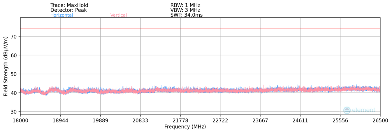
Plot 7-167. Radiated Spurious Plot above 18GHz MIMO
