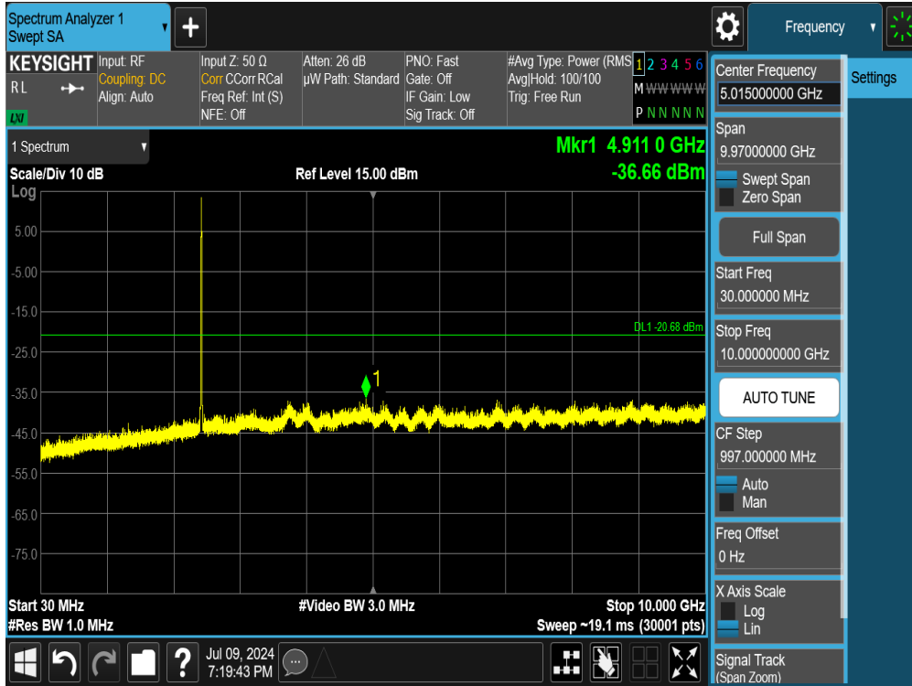
Plot 7-131. Conducted Spurious Plot SISO ANT1 (802.11b – Ch. 6)
