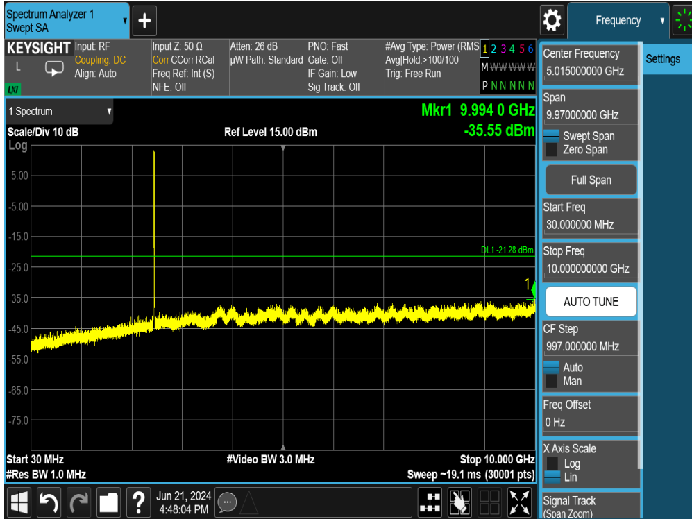
Plot 7-139. Conducted Spurious Plot SISO ANT2 (802.11b – Ch. 11)
