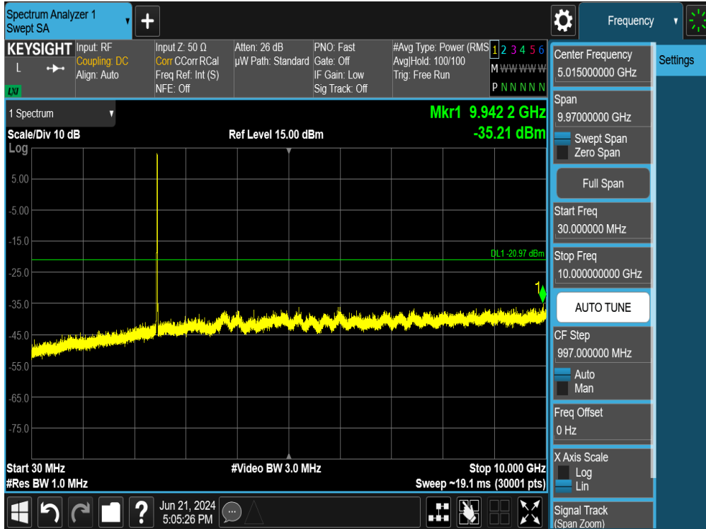
Plot 7-145. Conducted Spurious Plot MIMO ANT1 (802.11b – Ch. 11)
