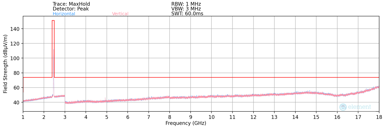
Plot 7-166. Radiated Spurious Plot above 1GHz MIMO (802.11b – Ch. 11)
