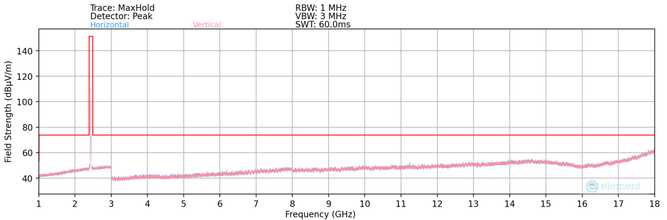
Plot 7-159. Radiated Spurious Plot above 1GHz SISO ANT2 (802.11b – Ch. 1)
