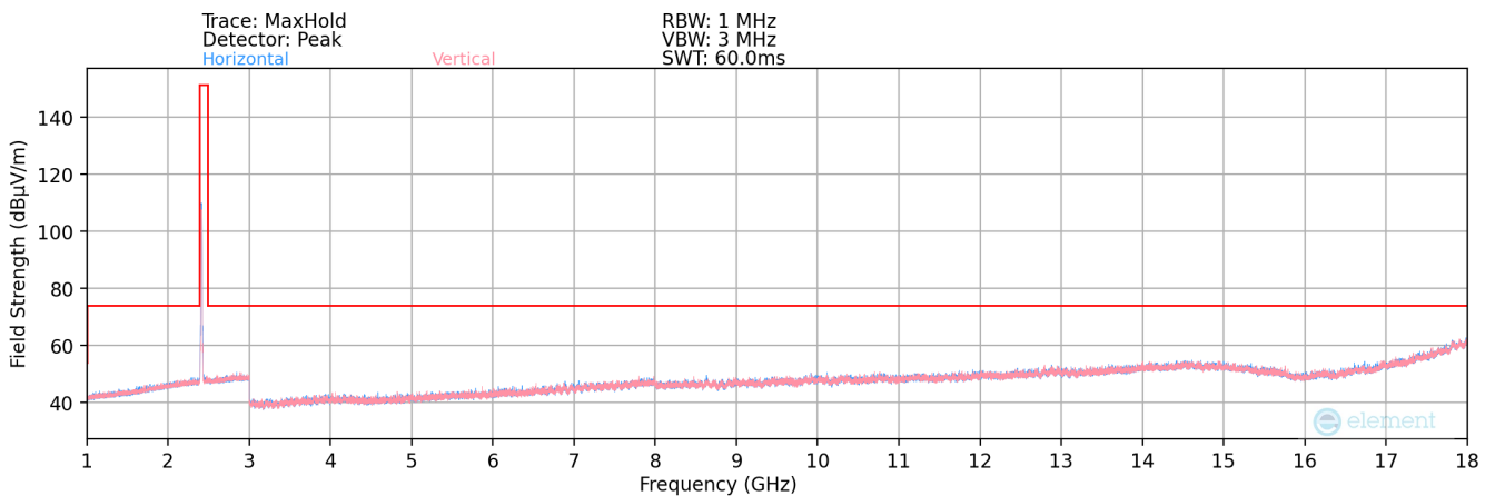
Plot 7-160. Radiated Spurious Plot above 1GHz SISO ANT2 (802.11b – Ch. 6)
