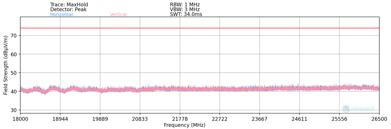
Plot 7-157. Radiated Spurious Plot above 18GHz SISO ANT1
