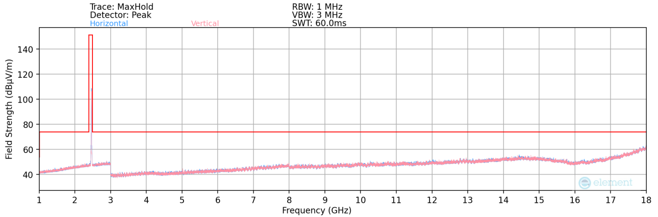
Plot 7-161. Radiated Spurious Plot above 1GHz SISO ANT2 (802.11b – Ch. 11)
