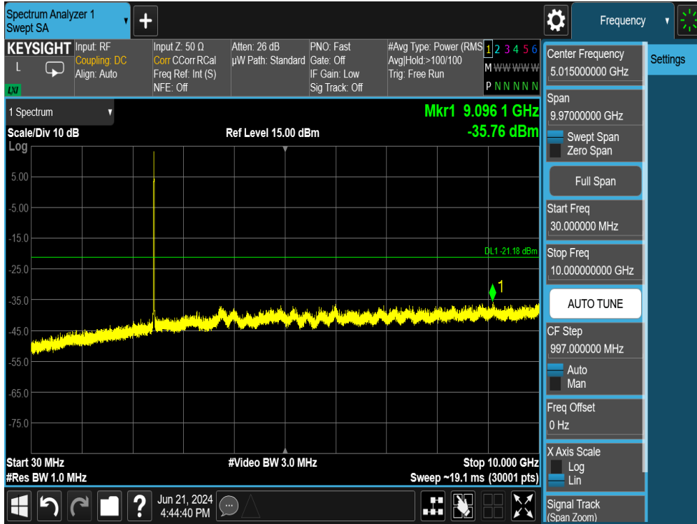
Plot 7-137. Conducted Spurious Plot SISO ANT2 (802.11b – Ch. 6)
