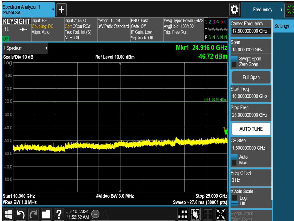
Plot 7-132. Conducted Spurious Plot SISO ANT1 (802.11b – Ch. 6)
