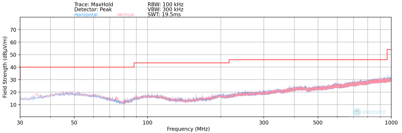
Plot 7-158. Radiated Spurious Plot below 1GHz SISO ANT2
