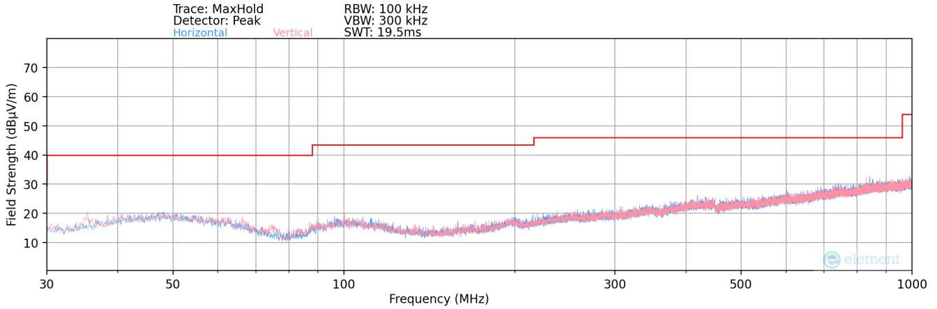
Plot 7-163. Radiated Spurious Plot below 1GHz MIMO
