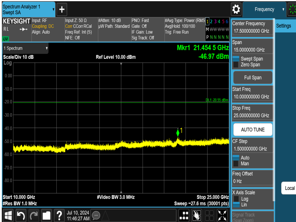
Plot 7-134. Conducted Spurious Plot SISO ANT1 (802.11b – Ch. 11)
