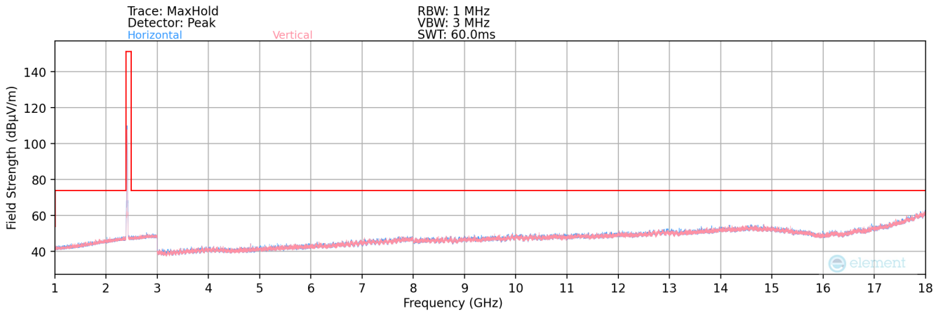
Plot 7-154. Radiated Spurious Plot above 1GHz SISO ANT1 (802.11b – Ch. 1)
