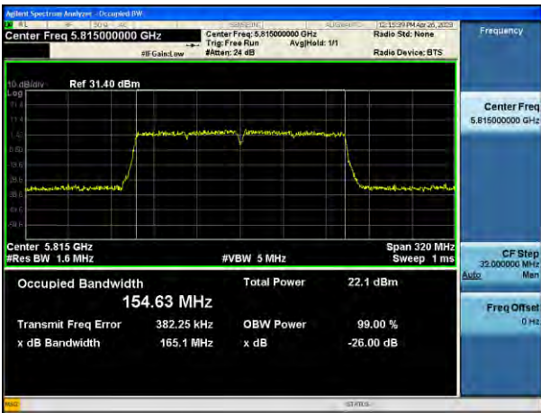
802.11ac_VHT160 UNII 4 BAND 26 dB Bandwidth(CH 163)
