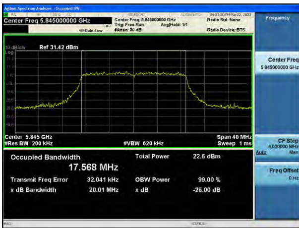
802.11ac_VHT20 UNII 4 BAND 26 dB Bandwidth(CH 169)
