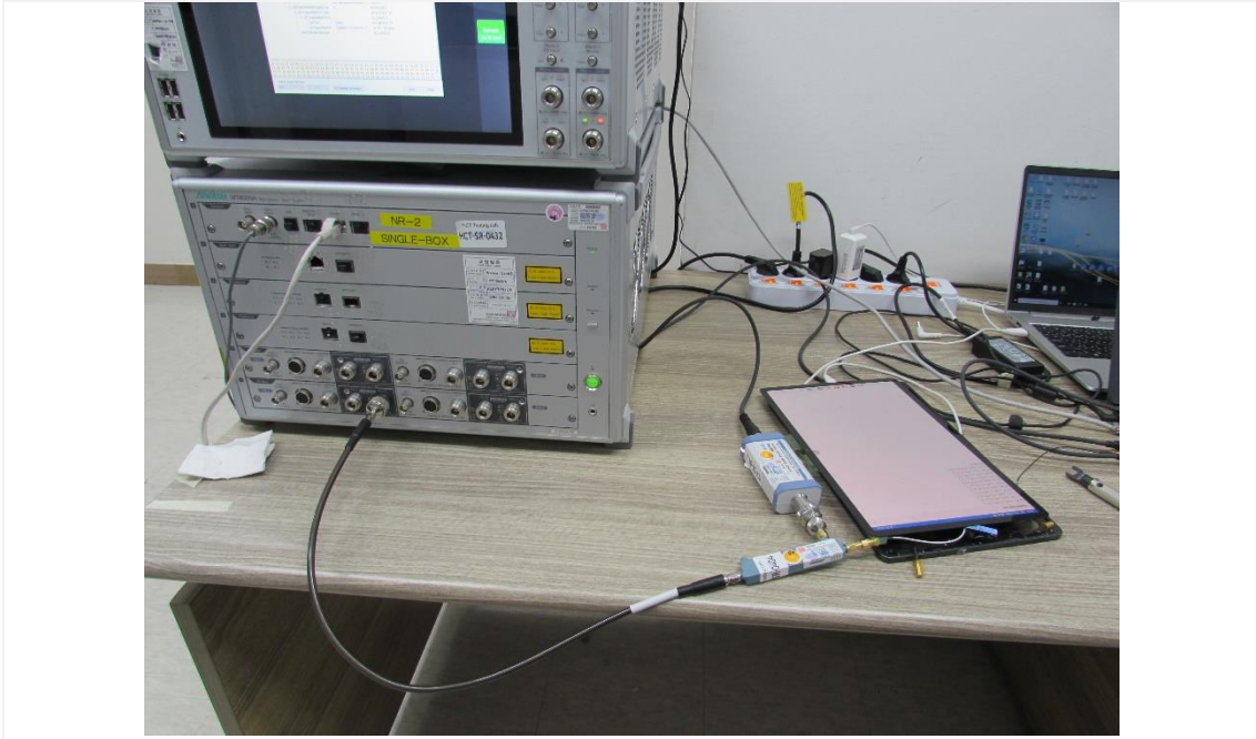
Test setup photo-4 (8-1(c) 5G Sub 6 SA)
