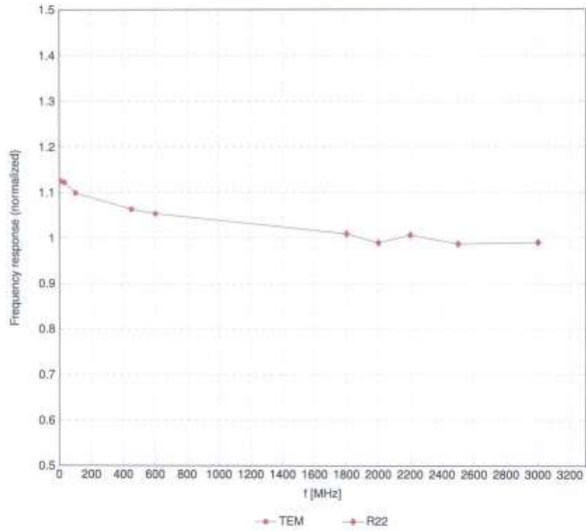
Frequency Response of E-Field (TEM-Cell:ff110 EXX, Waveguide:R22)
