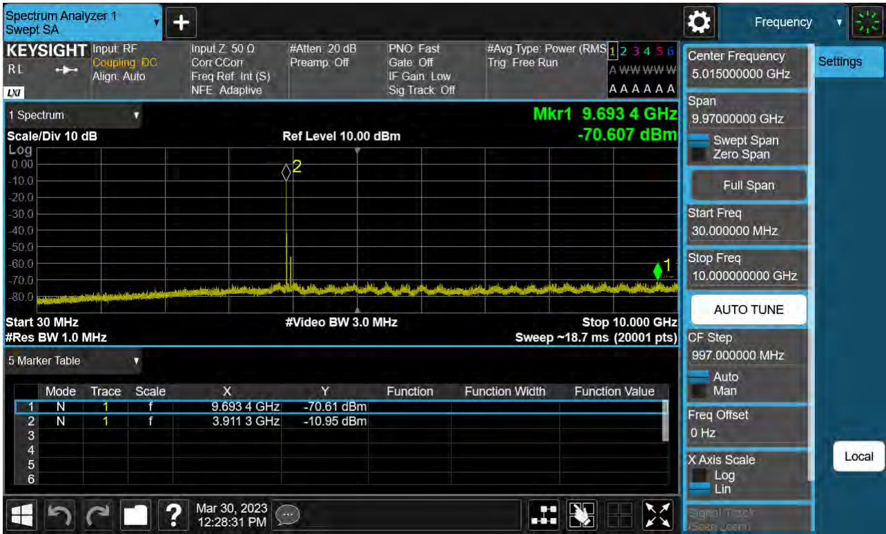
Sub6 n77. Conducted Spurious Plot_1 (663000ch_70 MHz_BPSK)
