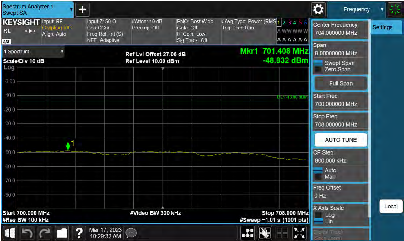
Sub6 n71. Upper Extended Band Edge Plot (20 M BW Ch.137600 BPSK_ Full RB)
