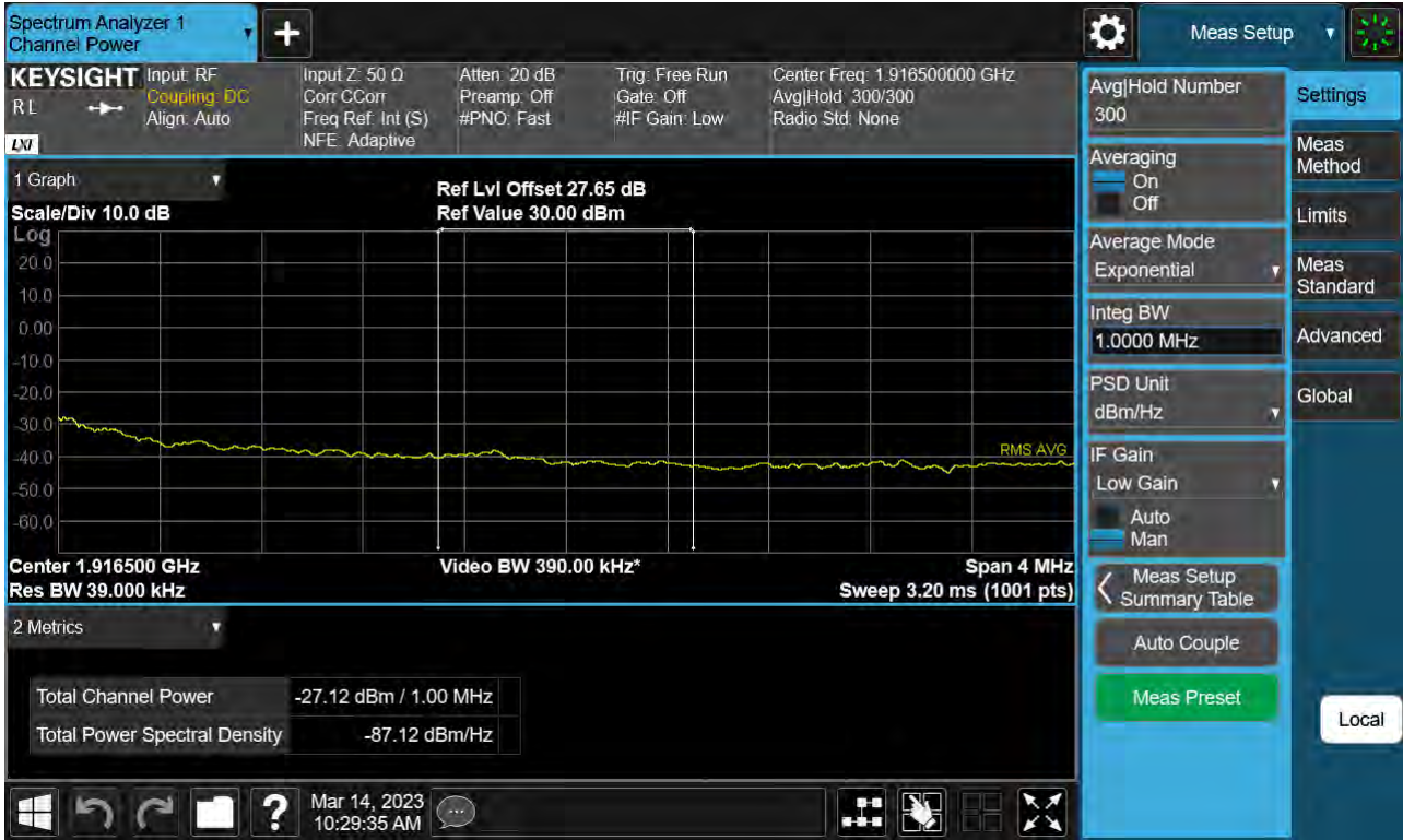
Sub6 n25(2). Upper Extended Band Edge Plot (10 M BW Ch.382000 BPSK_RB50_0) -2
