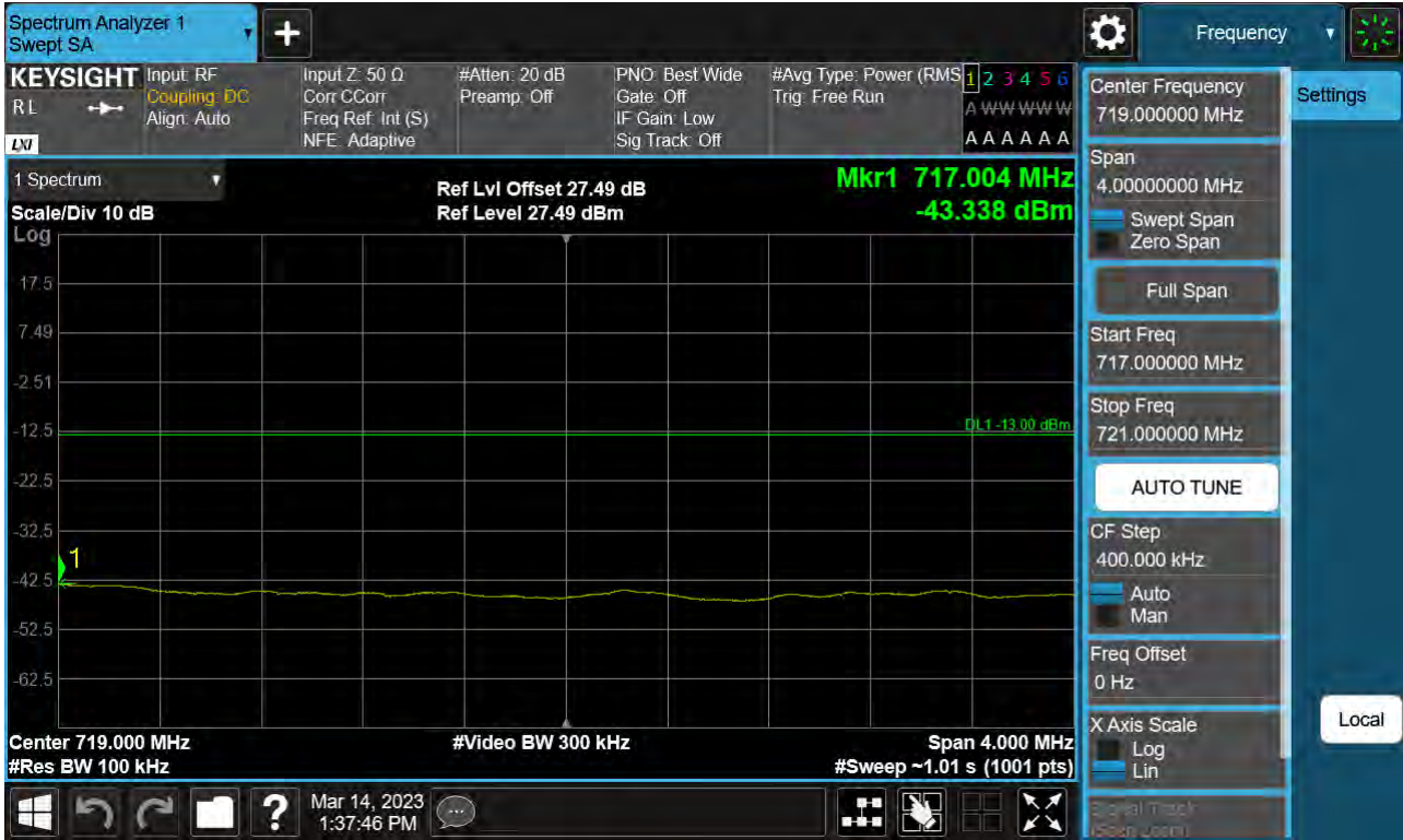
Sub6 n12. Upper Extended Band Edge Plot (15M BW Ch.141700 BPSK_RB75_0)
