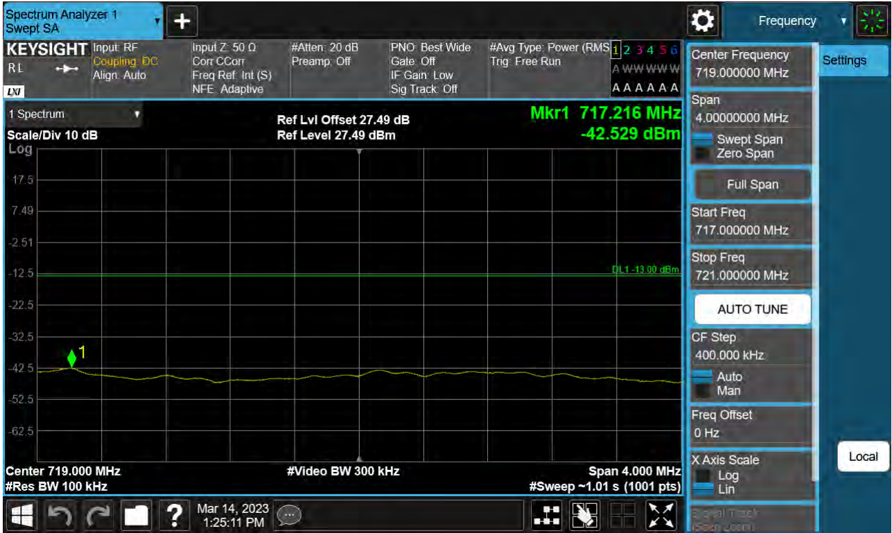
Sub6 n12. Upper Extended Band Edge Plot (10M BW Ch.142200 BPSK_RB50_0)
