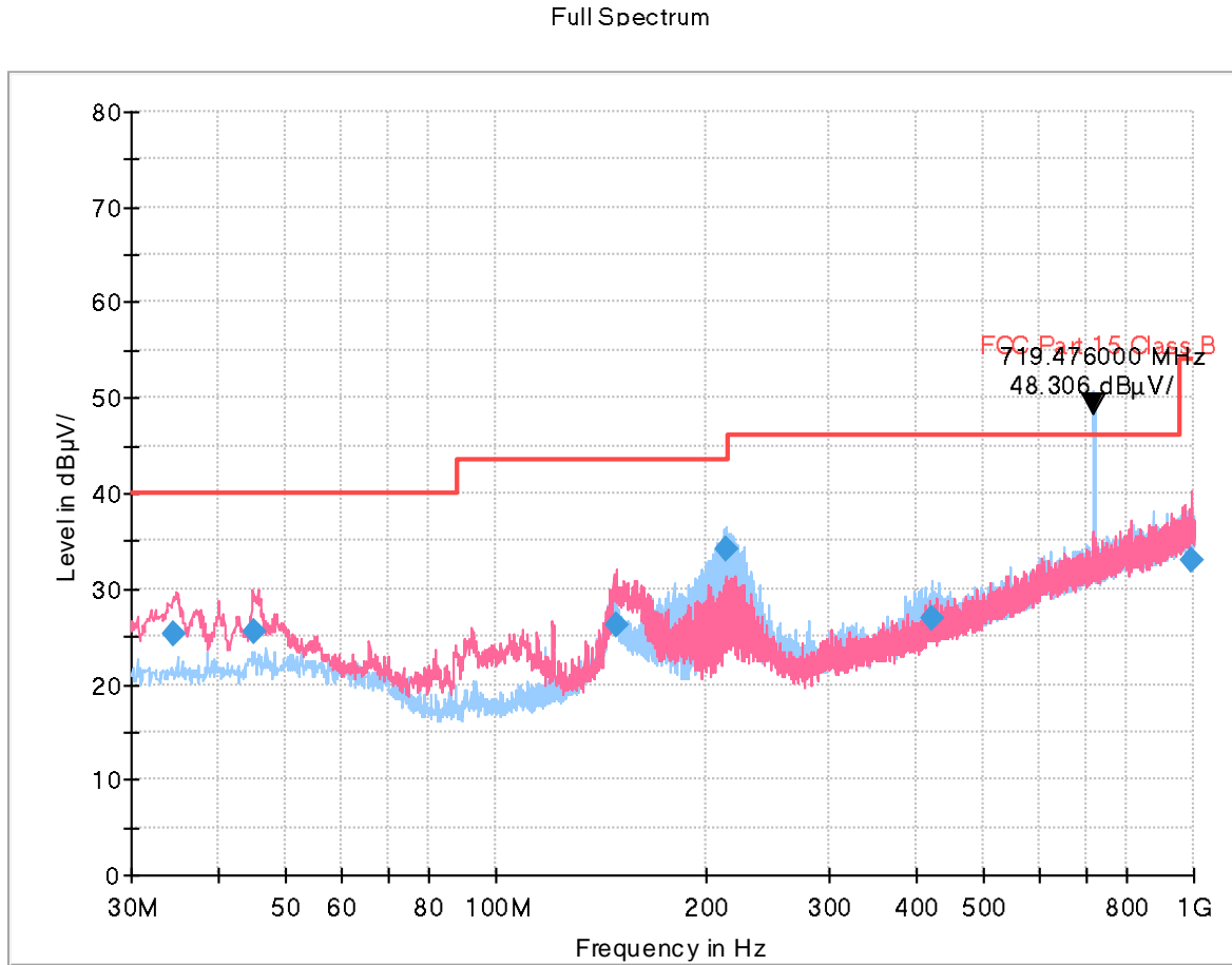
Figure 5: [EUT+TA + SPEN + Book Cover Keyboard] LTE B29 Low ch Idle
