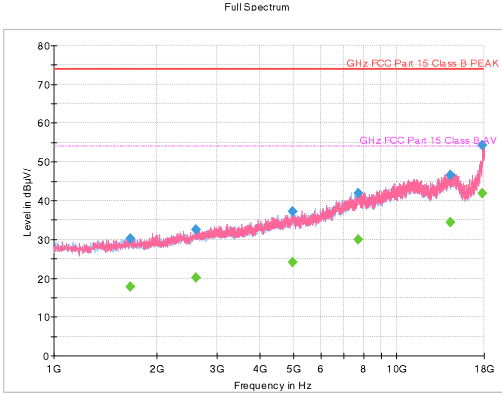
Figure 7: [EUT+TA + SPEN + Book Cover Keyboard] LTE B26+5G NR n26 High ch Idle
