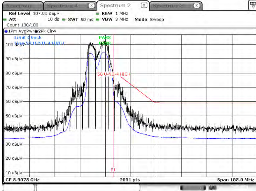
Average Result (802.11n HT20, Ch.177, Z-H)
