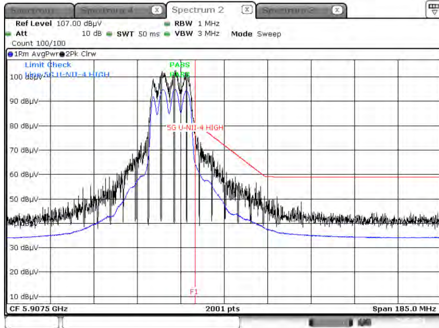
Average Result (802.11a, Ch.177, Z-H)
