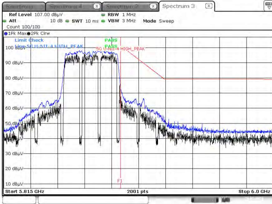
Peak(max) Result (802.11ac_VHT40, Ch.175, Z-H)
