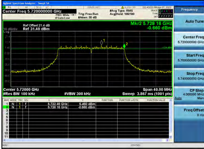
802.11ac_VHT20 CH.144
