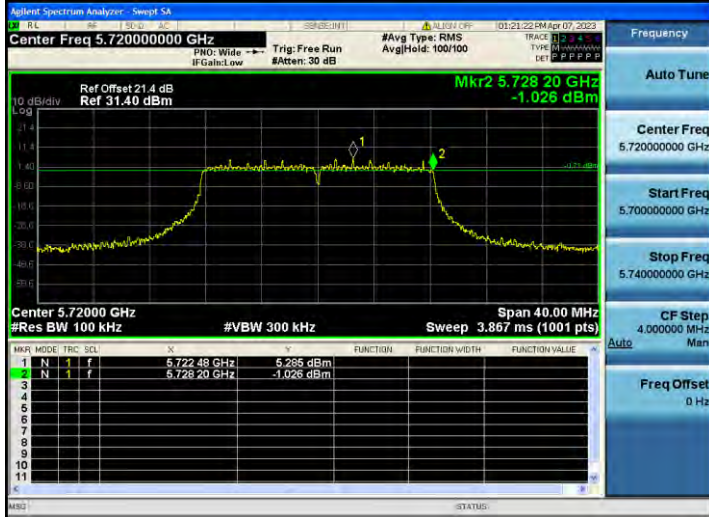
802.11ac_VHT20 CH.144
