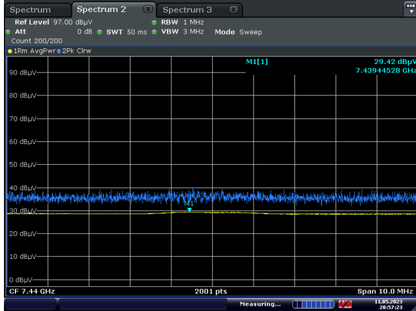
Radiated Spurious Emissions plot – Average Result (Ch. 39 3rd Harmonic, Y-V)
