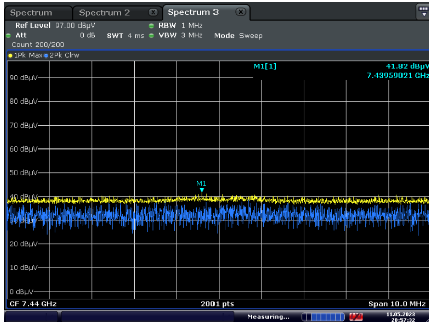
Radiated Spurious Emissions plot – Peak Result (Ch. 39 3rd Harmonic, Y-V)
