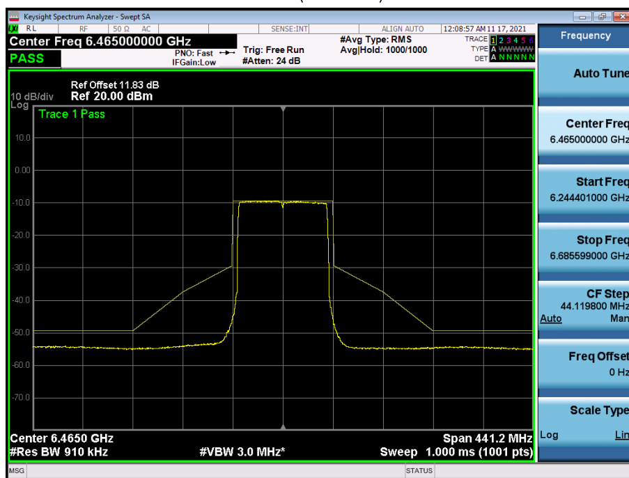
802.11ax HE80 Ch.103(6465 MHz) 996 Tones 67 RU
