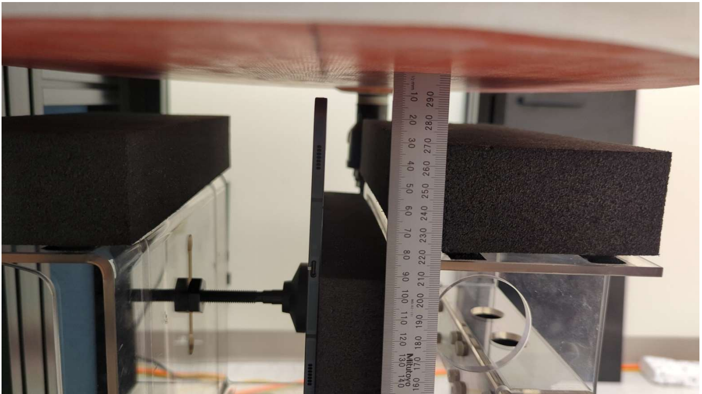
Photograph 18: Body & Hotspot, Edge Left, 11 mm, Side View
