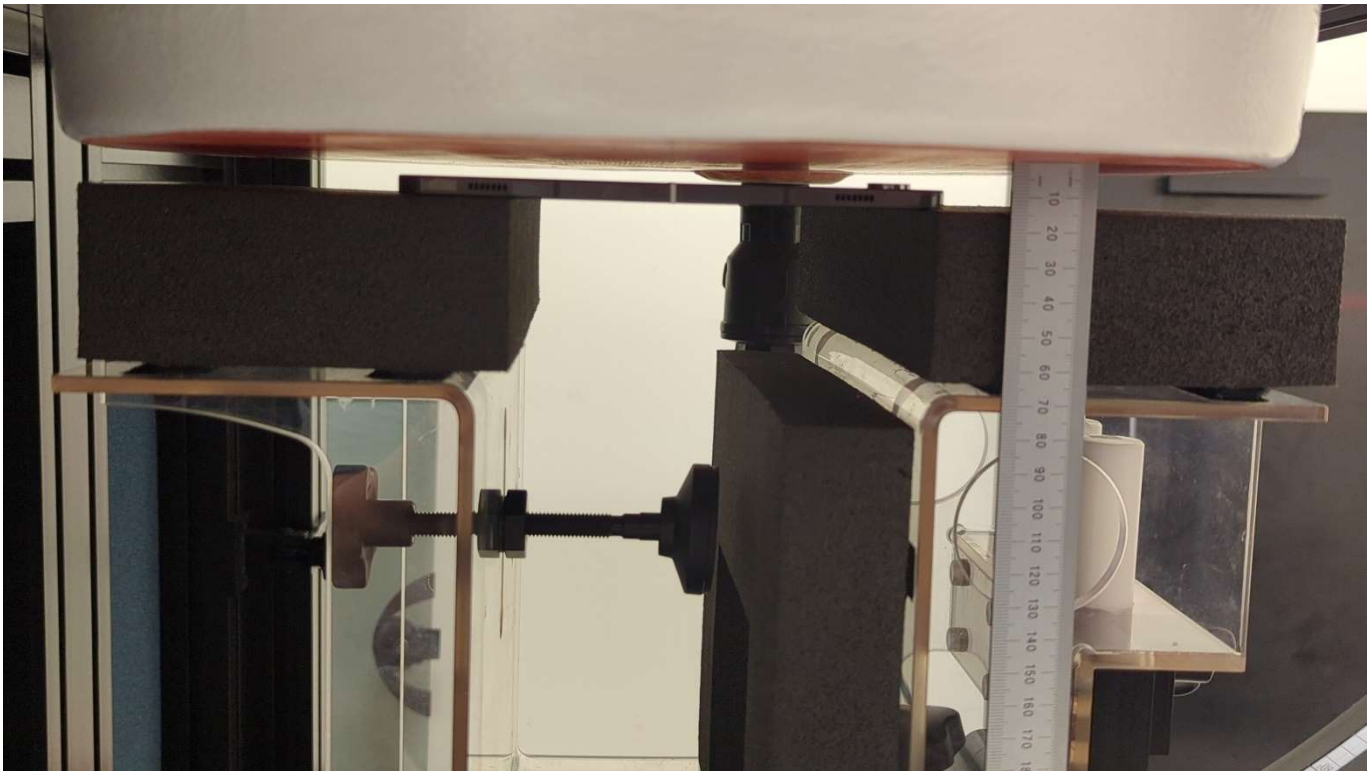
Photograph 7: Body & Hotspot, Back, 7 mm, Side View
