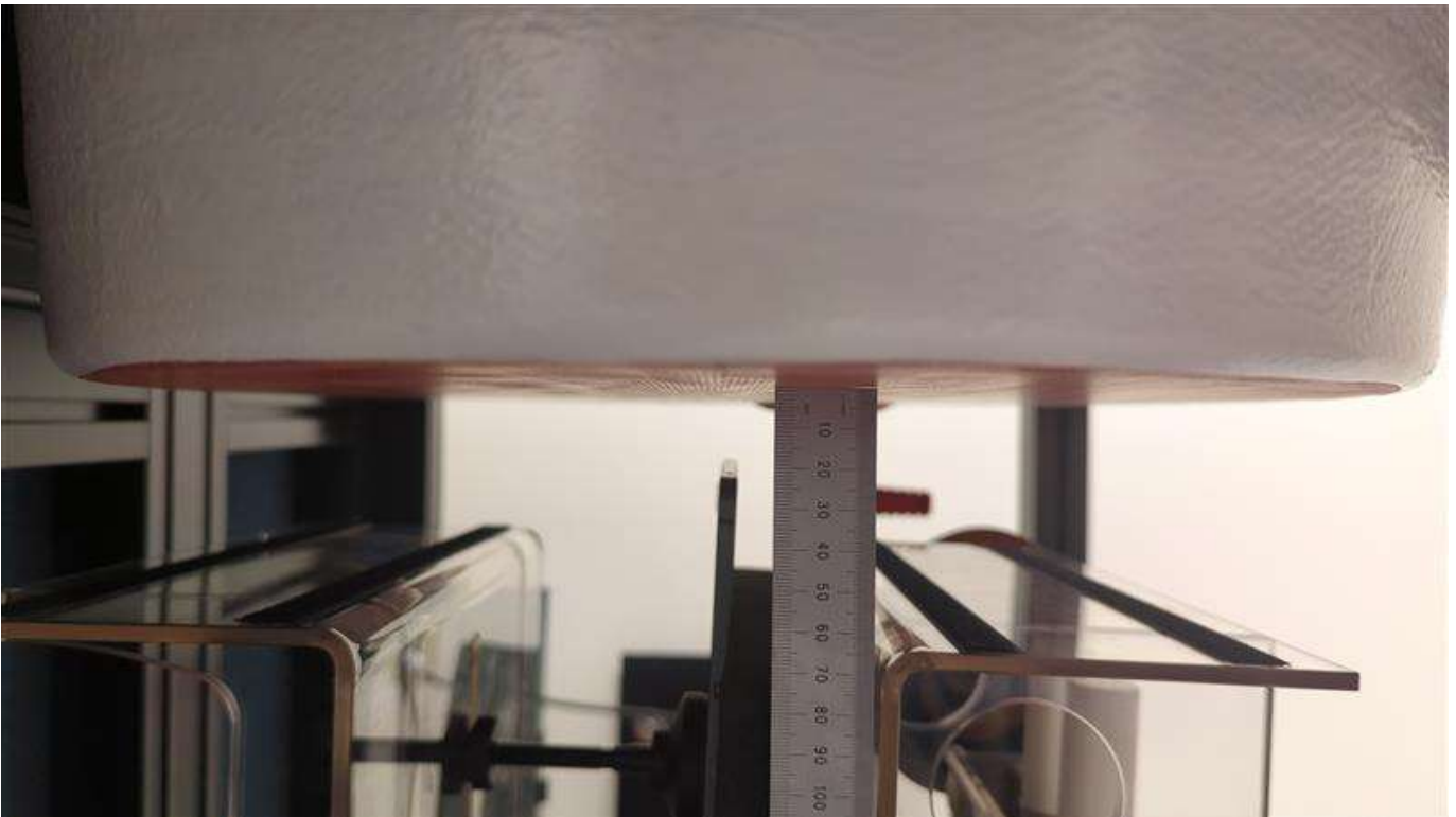
Photograph 5: Body & Hotspot, Edge Top, 26 mm, Side View
