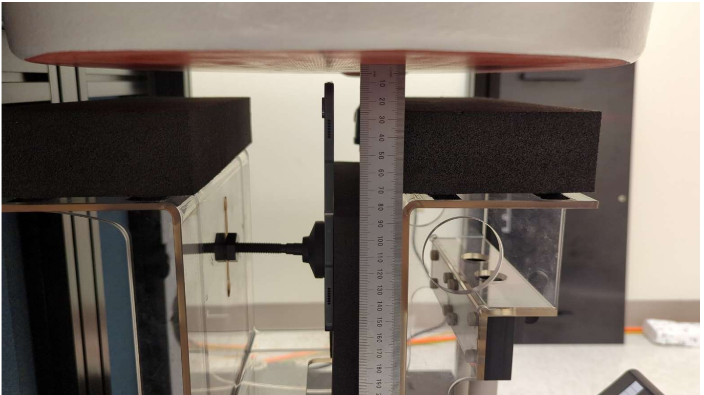
Photograph 10: Body & Hotspot, Edge Right, 10 mm, Side View
