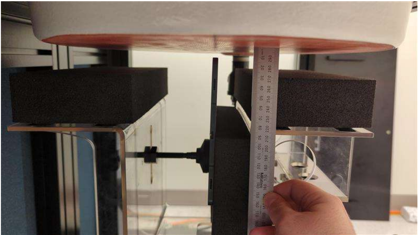
Photograph 16: Body & Hotspot, Edge Left, 10 mm, Side View
