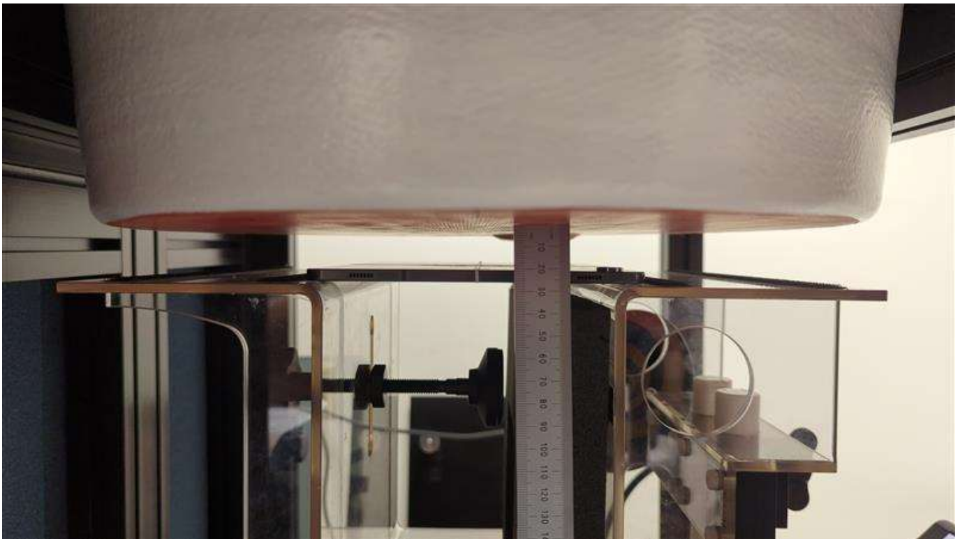
Photograph 11: Body & Hotspot, Back, 21 mm, Side View
