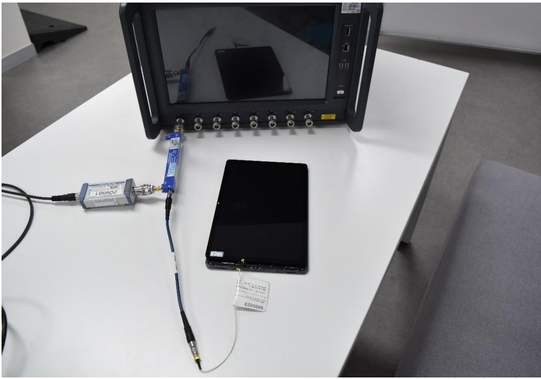
A.2 : Conducted test in UXM callbox
