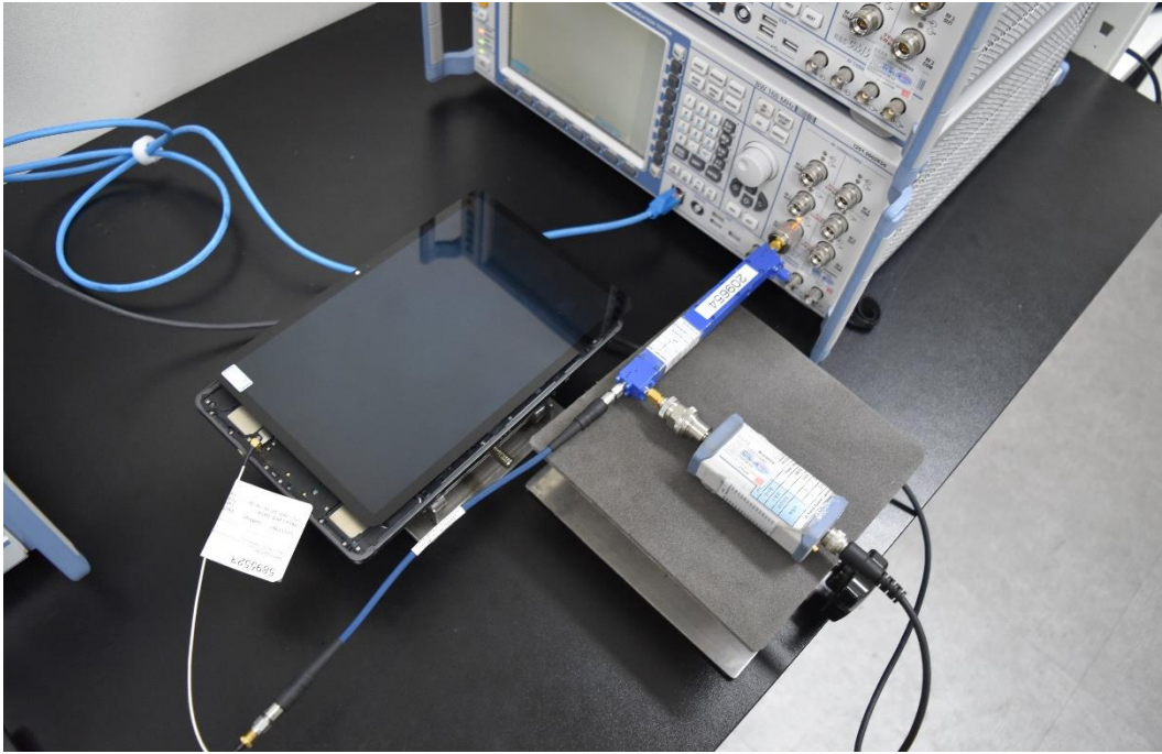
A.1 : Conducted test in CMW500 callbox
