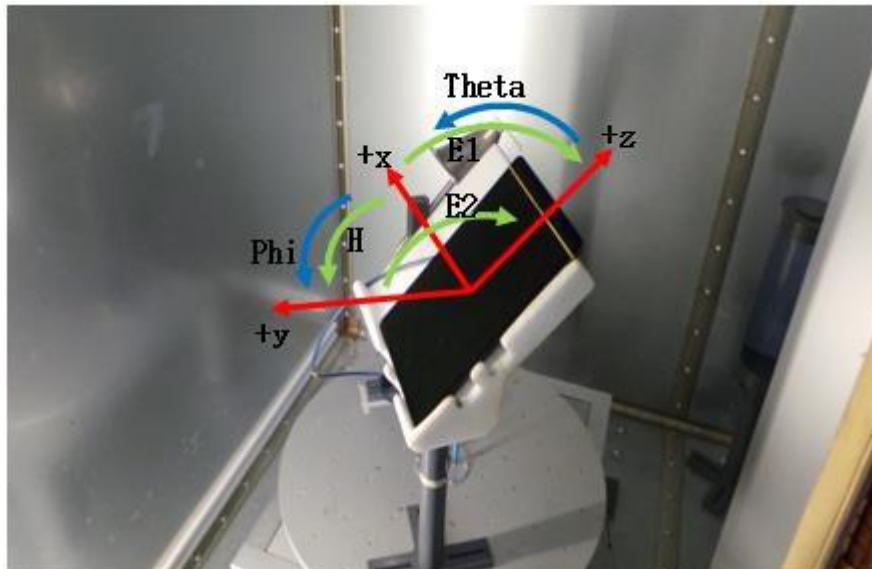
Geometry for SM-X616B for Radiation patterns.
