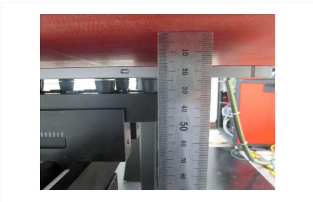
Distance of 17 mm from the EUT[WIFI1]
