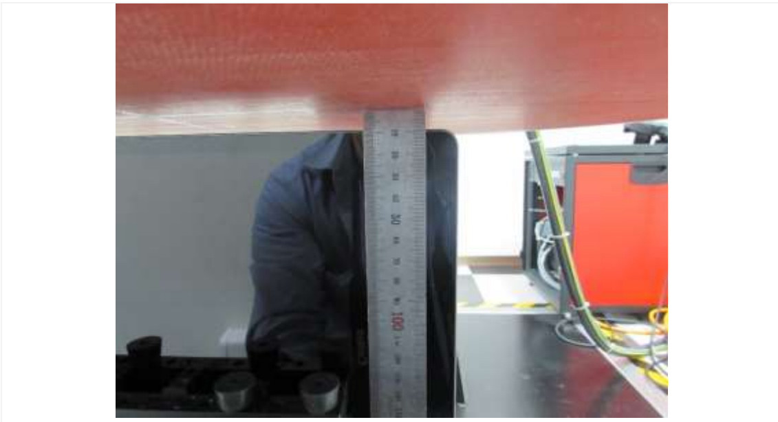
Distance of 9 mm from the EUT(WIF1)
