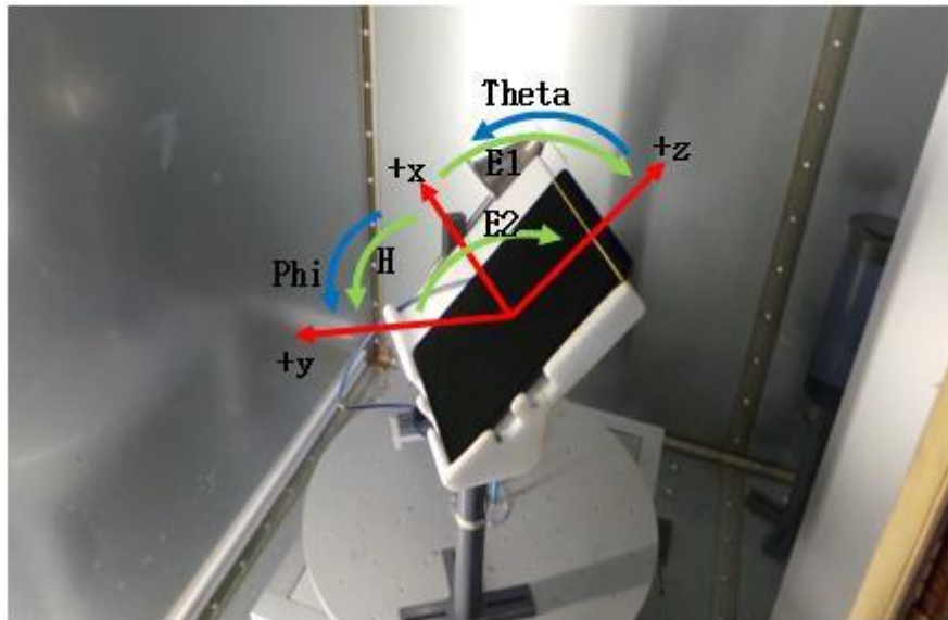
Geometry for SM-X616B, SM-X610 for Radiation patterns.
