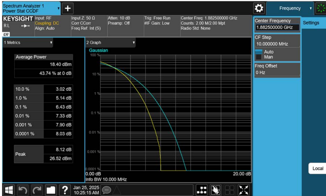
LTE B25_10 M_PAR_Mid_256QAM_FullRB
