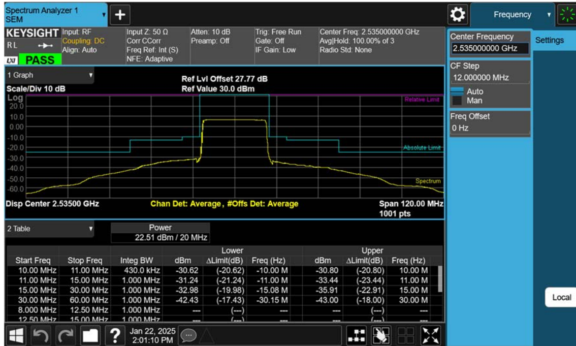
LTE B7_20 M_Channel Edge_Mid_QPSK_FullRB
