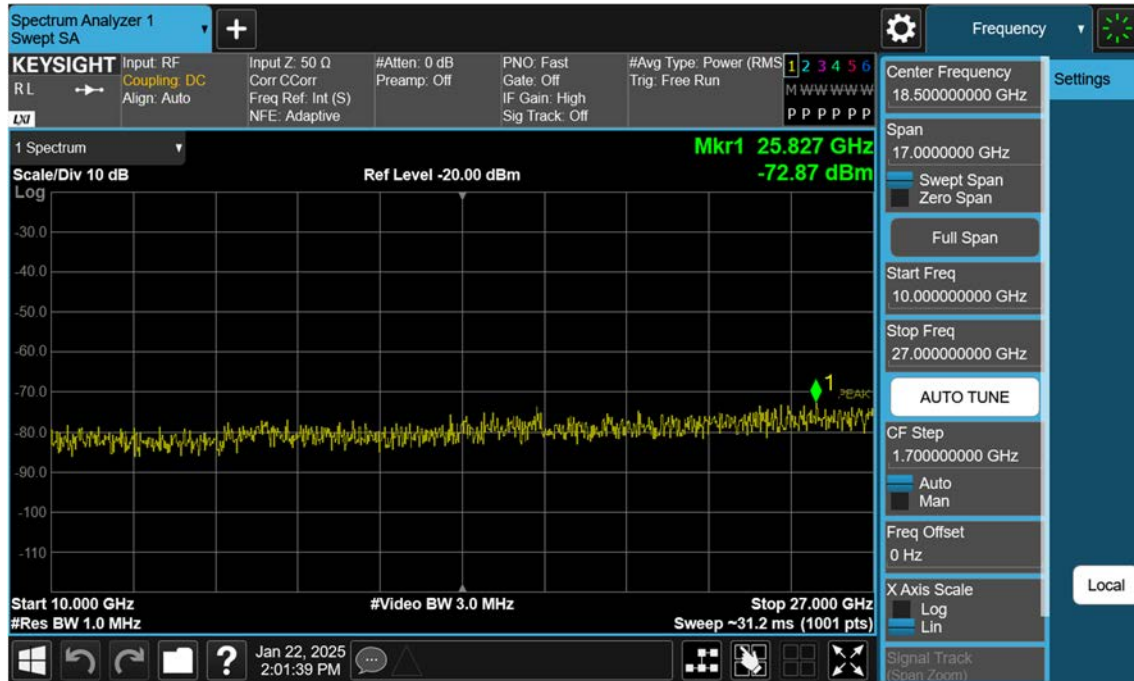
LTE B7_20 M_Conducted Spurious(Above10 G)_Mid_QPSK_1RB
