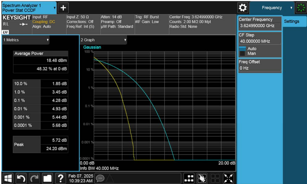
Sub6 n48. Plot (40 MHz Ch. 641666 BPSK RB 100)
