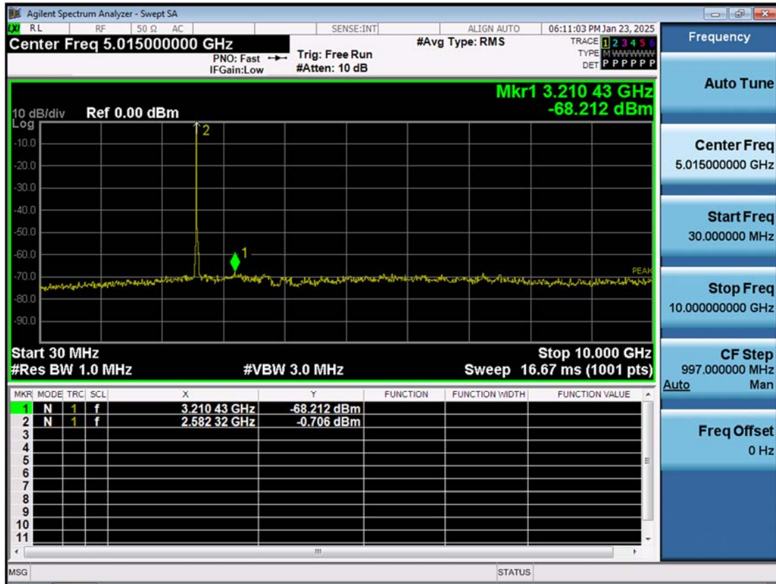
LTE B41_20 M_Conducted Spurious(30 M-10 G)_Mid_QPSK_1RB
