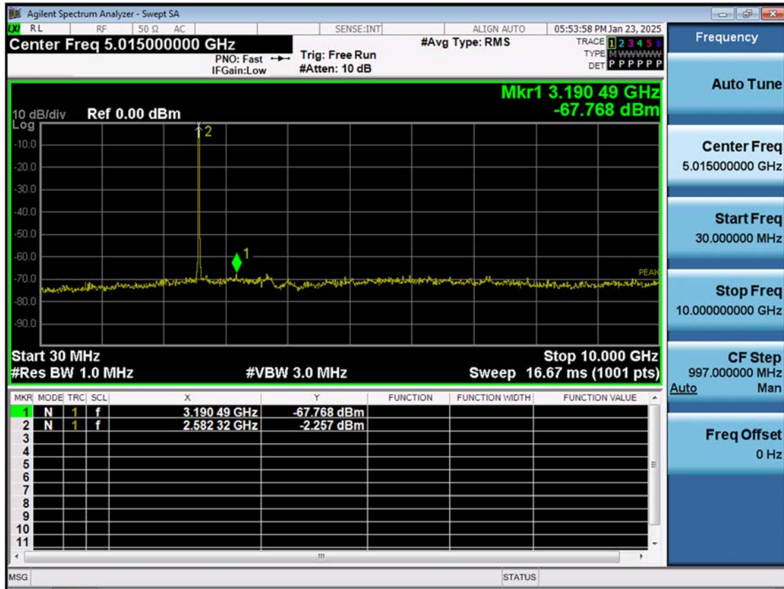
LTE B41_15 M_Conducted Spurious(30 M-10 G)_Mid_QPSK_1RB
