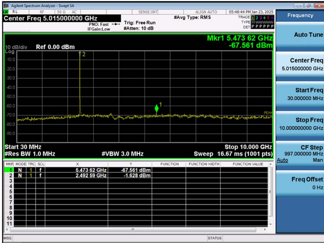
LTE B41_15 M_Conducted Spurious(30 M-10 G)_Low_QPSK_1RB
