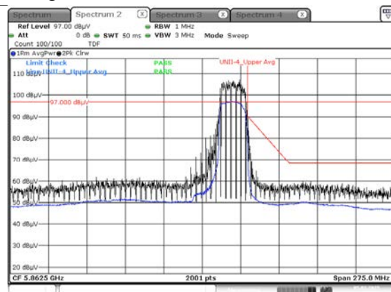
Average result (802.11ax(HE40) Ch.175, 242T RU 62)
