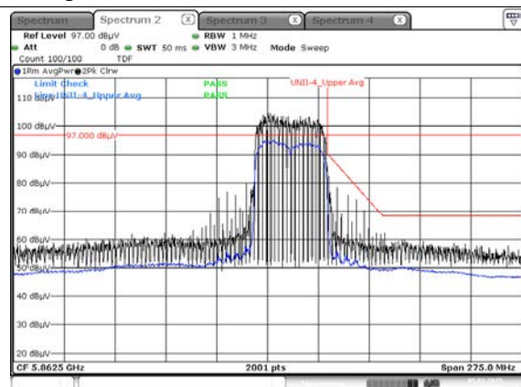
Average result (802.11ax(HE40) Ch.175, 484T RU 65)
