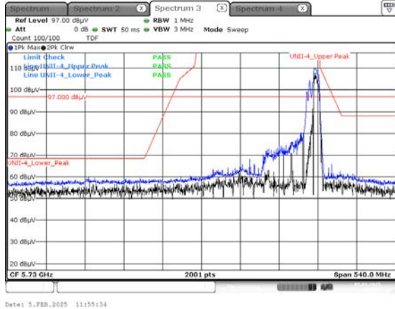
Peak result (802.11ax(HE80) Ch.171, 484T RU 66)
