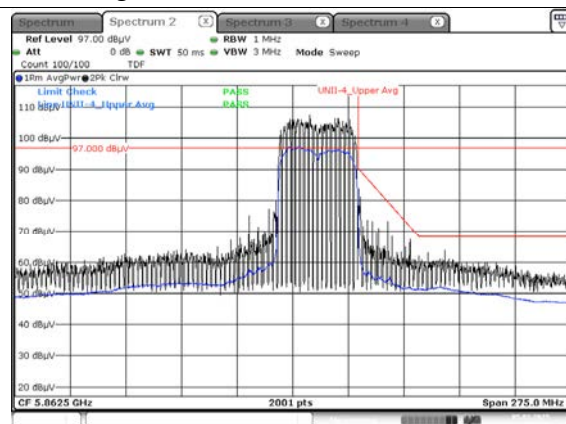
Average result (802.11ax(HE40) Ch.175, SU)
