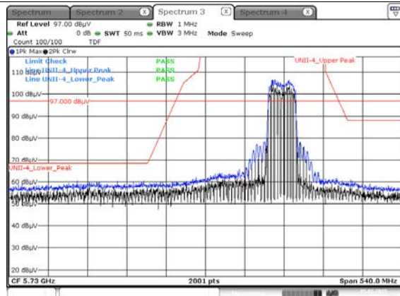
Peak result (802.11ax(HE40) Ch.167, 484T RU 65)
