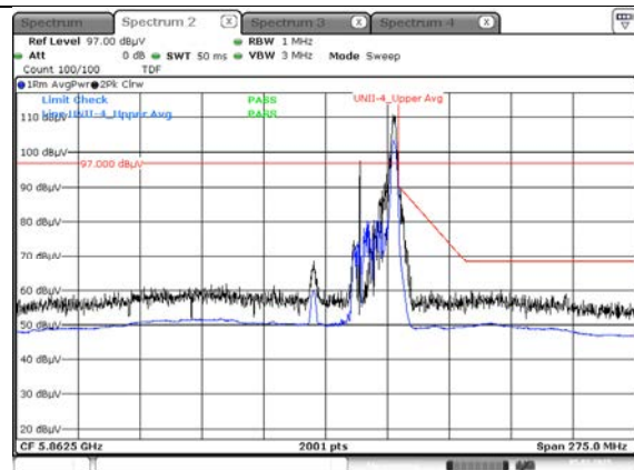
Average result (802.11ax(HE40) Ch.175, 26T RU 17)
