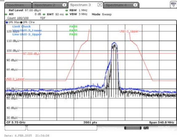
Peak result (802.11ax(HE40) Ch.159, SU)
