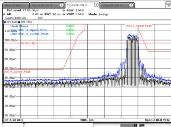
Peak result (802.11ax(HE40) Ch.175, 484T RU 65)
