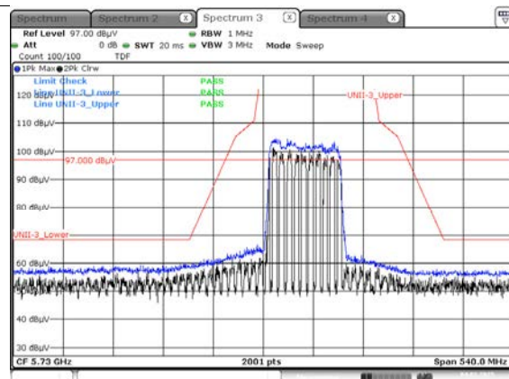
Peak result (802.11ax(HE80) Ch.155, 996T RU 67)
