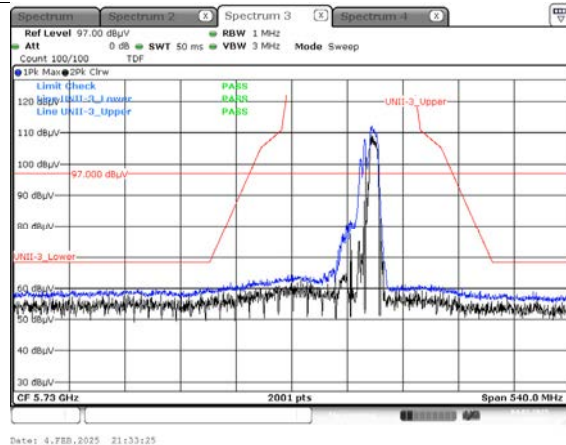
Peak result (802.11ax(HE40) Ch.159, 484T RU 65)
