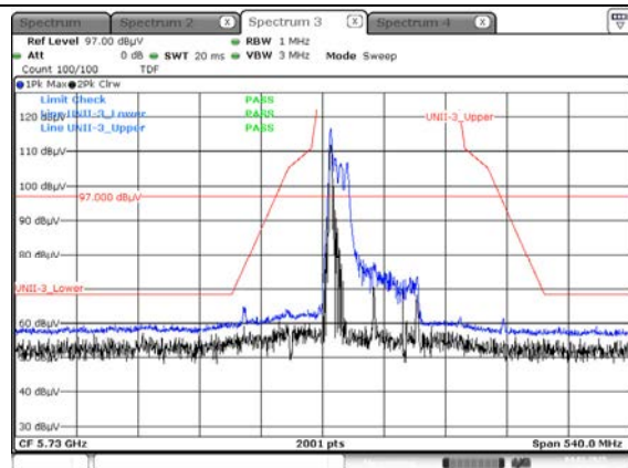
Peak result (802.11ax(HE80) Ch.155, 26T RU 0)
