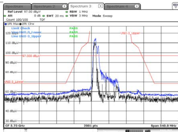
Peak result (802.11ax(HE80) Ch.155, 106T RU 53)
