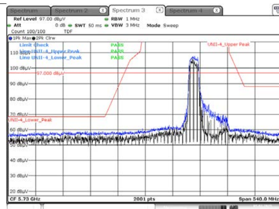
Peak result (802.11ax(HE80) Ch.171, 242T RU 61)
