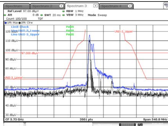
Peak result (802.11ax(HE80) Ch.155, 52T RU 37)
