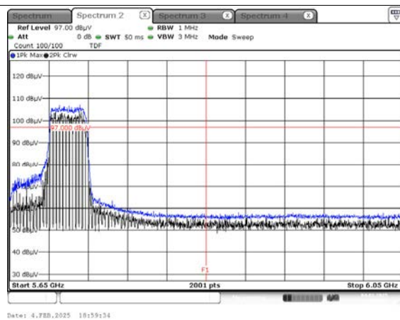
Peak result (802.11ax(HE80) Ch.138, 484T RU 66)
