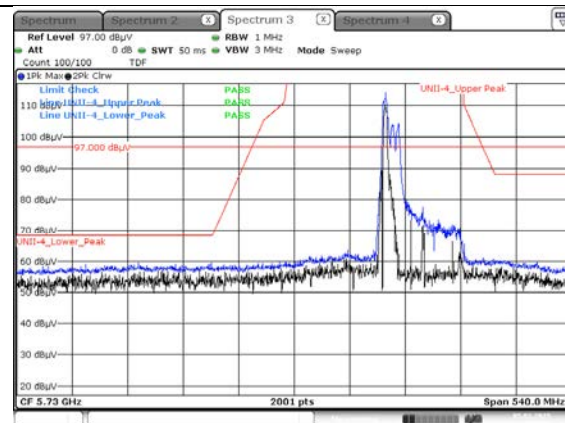
Peak result (802.11ax(HE80) Ch.171, 52T RU 37)
