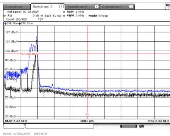
Peak result (802.11ax(HE80) Ch.138, 106T RU 60)
