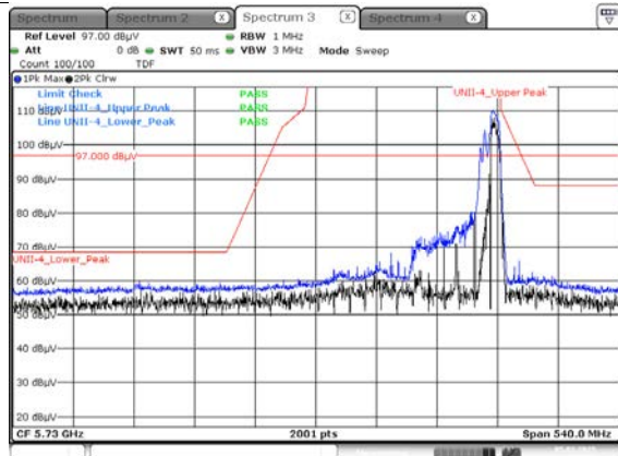
Peak result (802.11ax(HE80) Ch.171, 106T RU 60)
