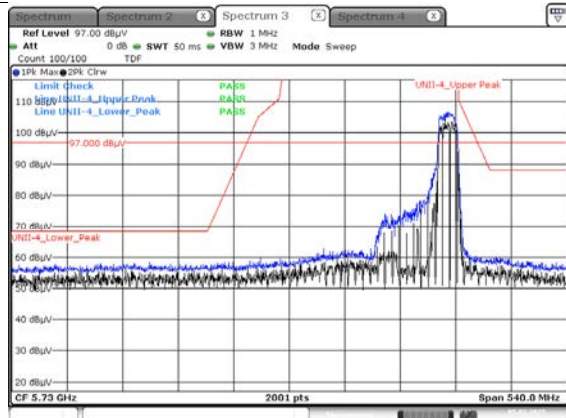
Peak result (802.11ax(HE80) Ch.171, 242T RU 64)
