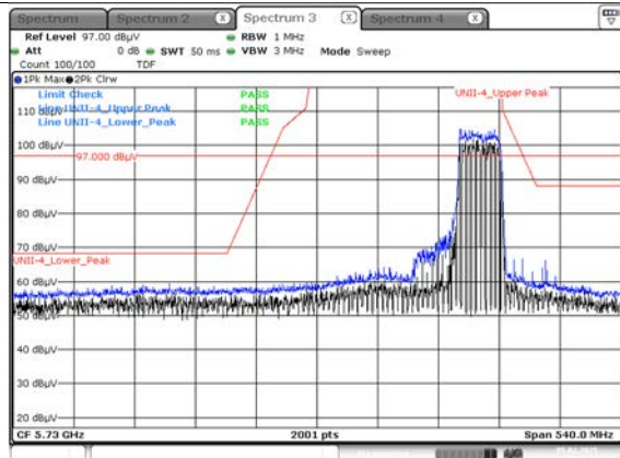
Peak result (802.11ax(HE80) Ch.171, 484T RU 66)
