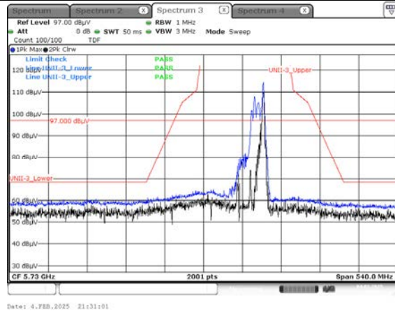
Peak result (802.11ax(HE40) Ch.159, 106T RU 56)
