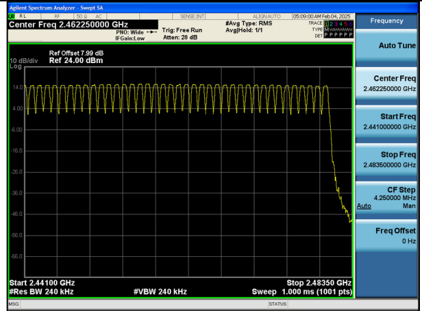
8DPSK (2.441 GHz - 2.483.5 GHz)
