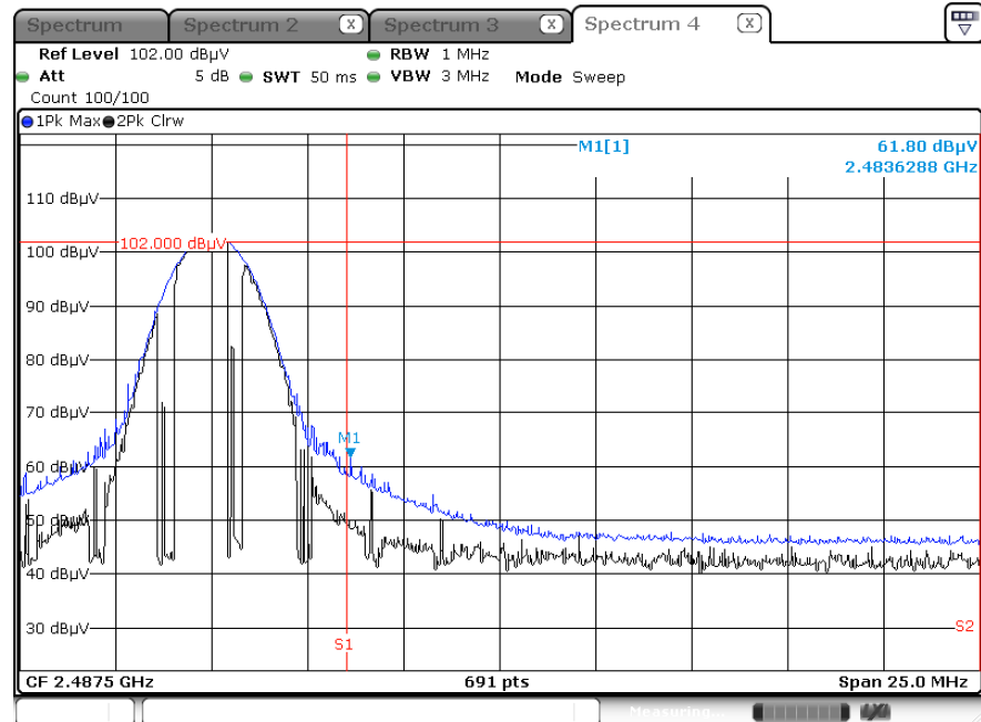
Radiated Restricted Band Edges plot – Average &amp; Peak Result (8DPSK, Ch.78, X-H)
