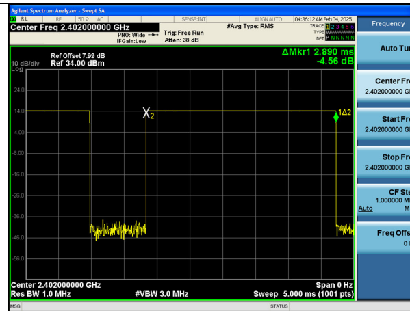
8DPSK : Dwell Time(Ch. 0)
