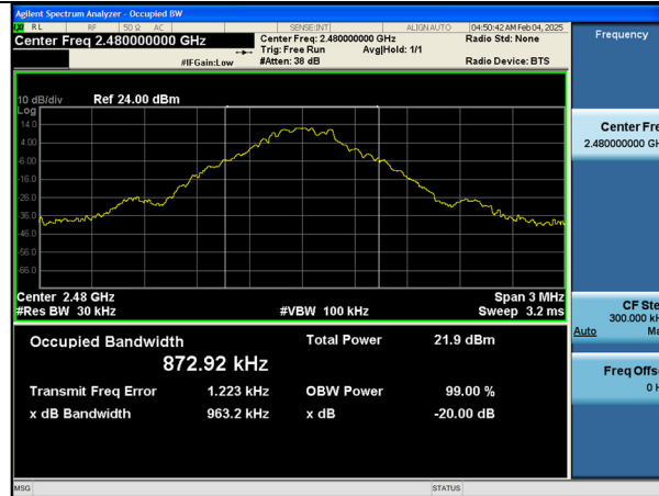
8DPSK 20 dB BW &amp; 99% OBW (Ch. 78)
