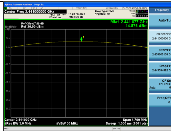
8DPSK : Peak Power (Ch. 39)
