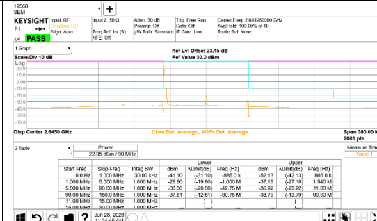
DFT-s_OFDM_16QAM High channel 1RB_Offset Low
