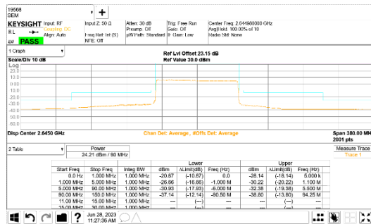
DFT-s_OFDM_16QAM High channel FRB
