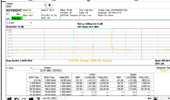
DFT-s_OFDM_16QAM High channel 1RB_Offset High
