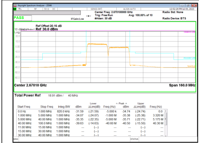
LTE B41 20MHz + 20MHz 16QAM High Ch RB100-0 + RB100-0
