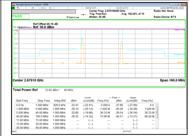
LTE B41 20MHz + 20MHz 16QAM High Ch RB1-0 + RB1-99
