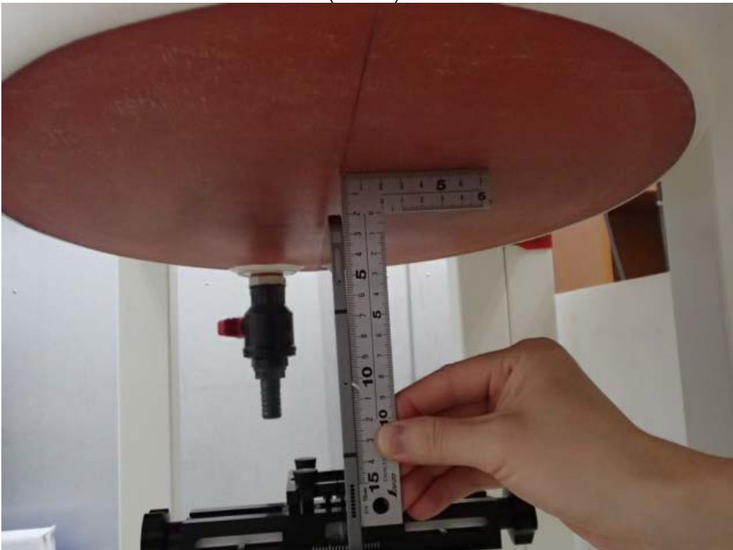
Left Side (19 mm) Side View
