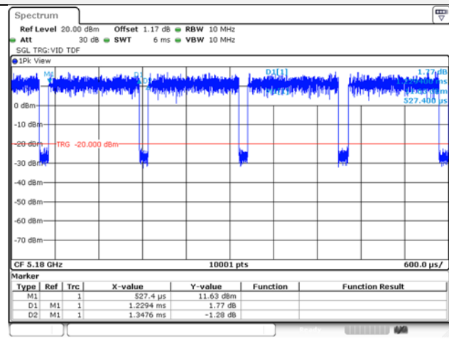
802.11ax_HE20 / 106T
