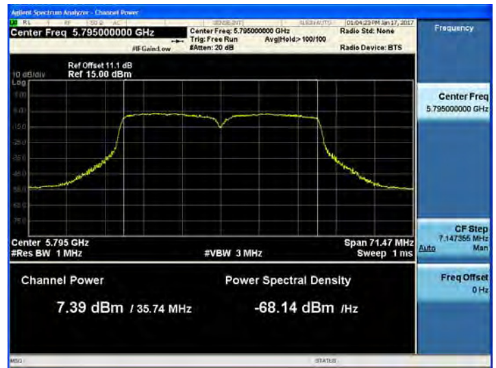
802.11ac_VHT40 UNII 3 BAND Average Power (5755 MHz ~5795 MHz) CH 159 MCS6
