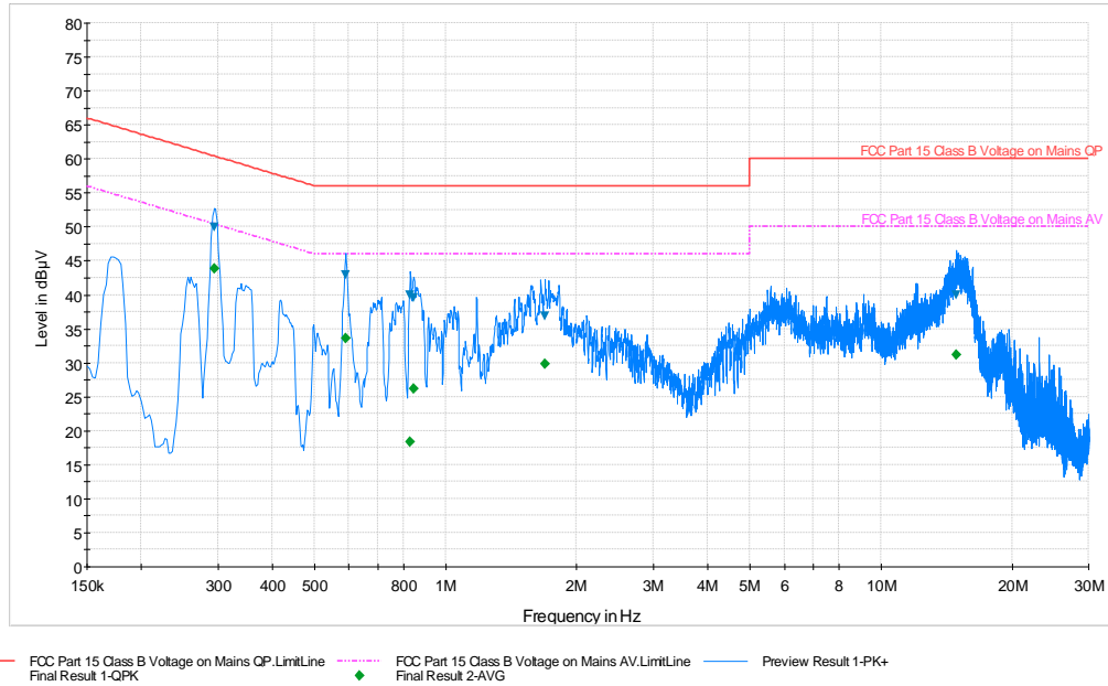
Plot 6-68. Line Conducted Plot with 802.11b (N)
