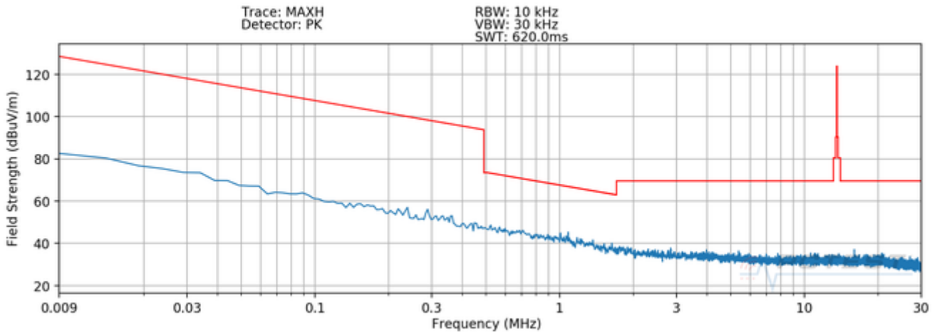
Plot 7-9. Radiated Spurious Plot 9kHz – 30MHz (Pol. Z – WPT - Digitizer S-Pen Click)
