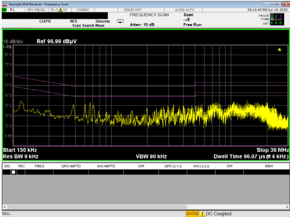
Plot 7-13. Line-Conducted Test Plot (N) – Digitizer S-Pen Click
