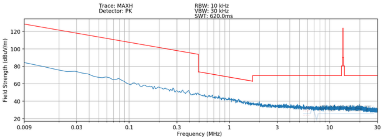
Plot 7-3. Radiated Spurious Plot 9kHz – 30MHz (Pol. Z – WPT - Device to S-Pen)
