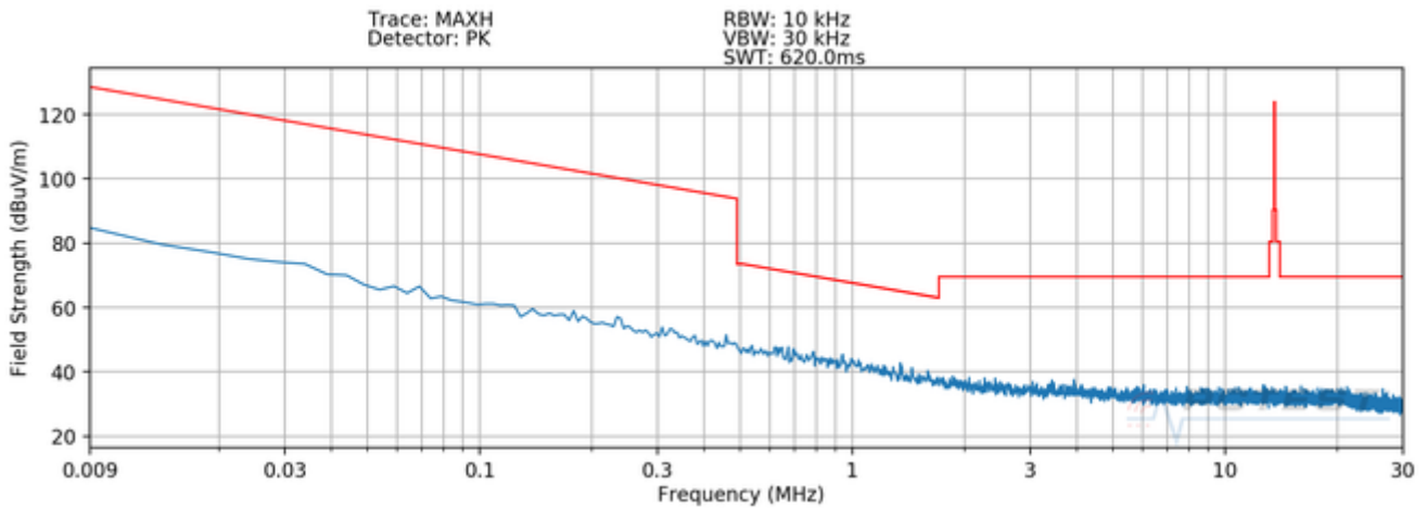
Plot 7-2. Radiated Spurious Plot 9kHz – 30MHz (Pol. Y – WPT - Device to S-Pen)
