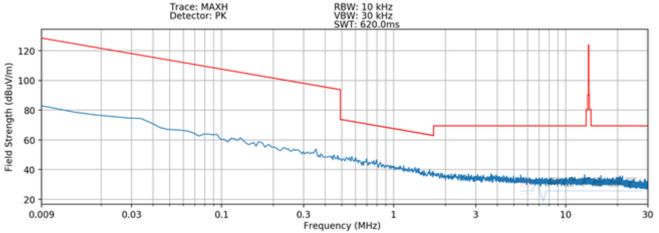
Plot 7-1. Radiated Spurious Plot 9kHz – 30MHz (Pol. X – WPT - Device to S-Pen)
