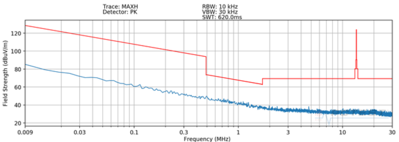
Plot 7-6. Radiated Spurious Plot 9kHz – 30MHz (Pol. Z – WPT - Digitizer Hover)
