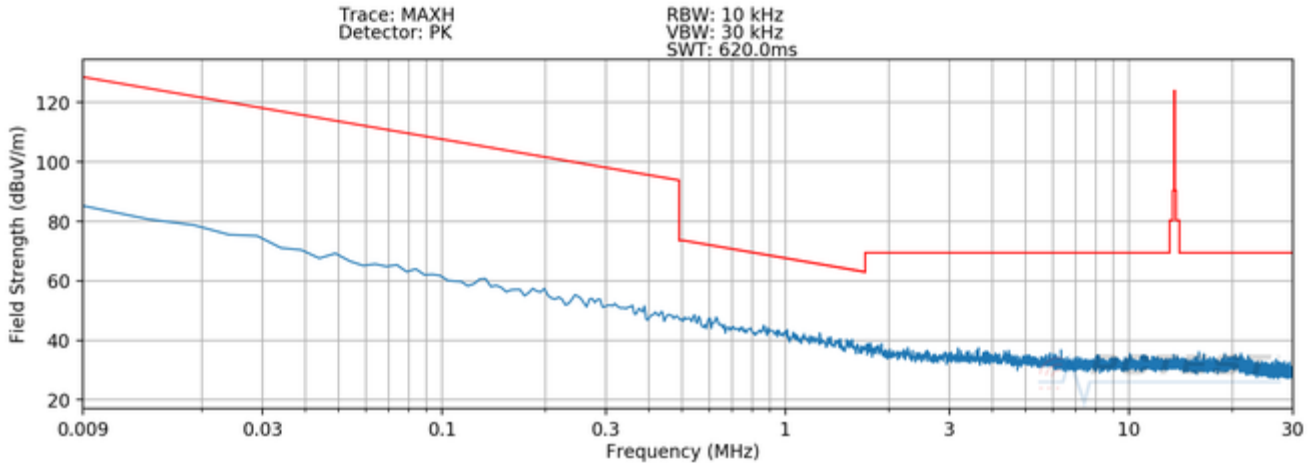
Plot 7-4. Radiated Spurious Plot 9kHz – 30MHz (Pol. X – WPT – Digitizer Hover)
