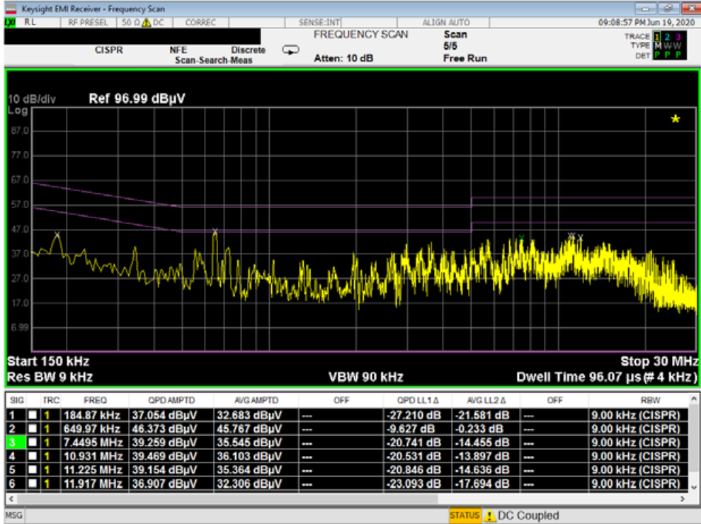
Plot 7-10. Line-Conducted Test Plot (L1) – Digitizer Hover
