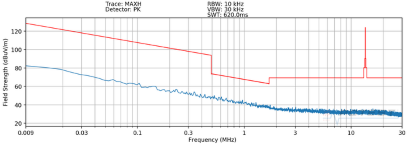
Plot 7-7. Radiated Spurious Plot 9kHz – 30MHz (Pol. X – WPT – Digitizer S-Pen Click)
