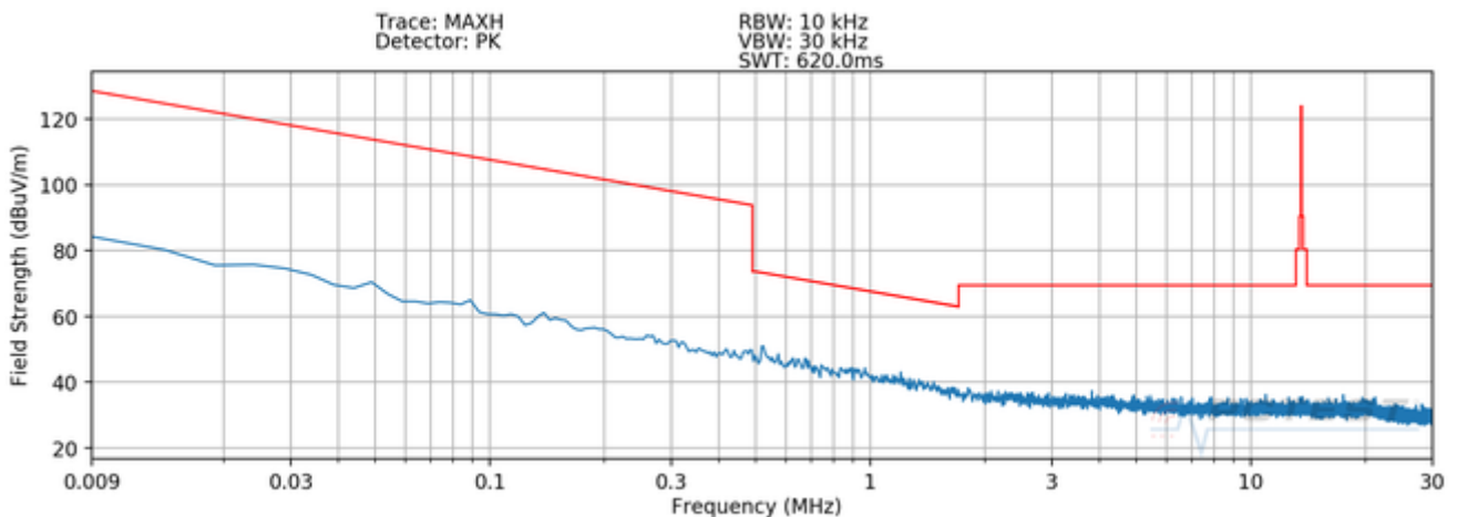
Plot 7-5. Radiated Spurious Plot 9kHz – 30MHz (Pol. Y – WPT - Digitizer Hover)
