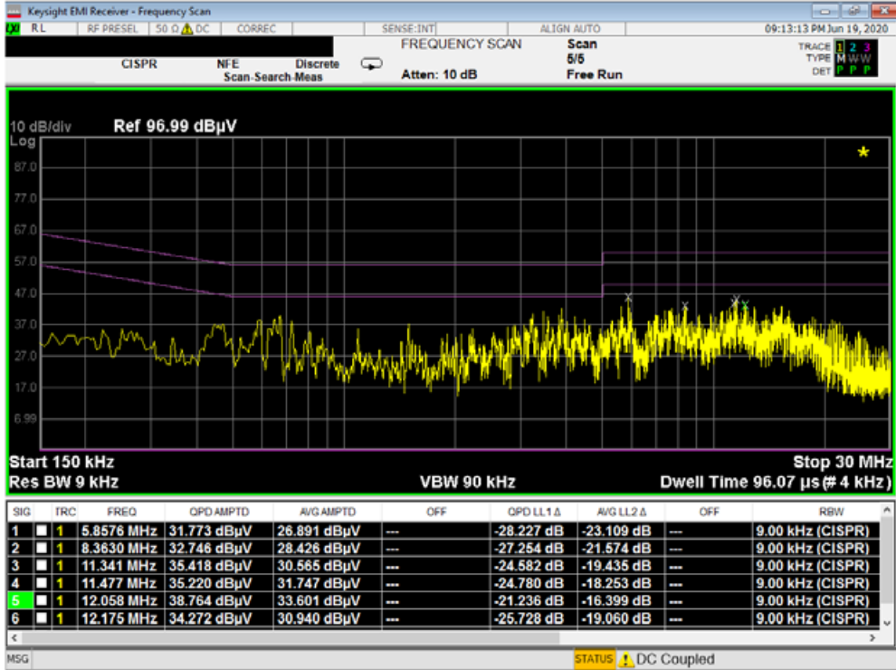
Plot 7-12. Line-Conducted Test Plot (L1) – Digitizer S-Pen Click
