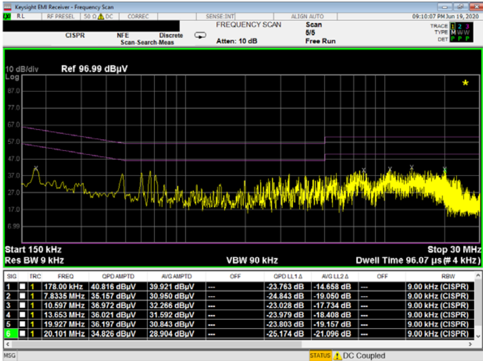
Plot 7-11. Line-Conducted Test Plot (N) – Digitizer Hover
