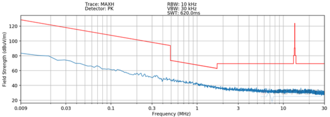
Plot 7-8. Radiated Spurious Plot 9kHz – 30MHz (Pol. Y – WPT - Digitizer S-Pen Click)
