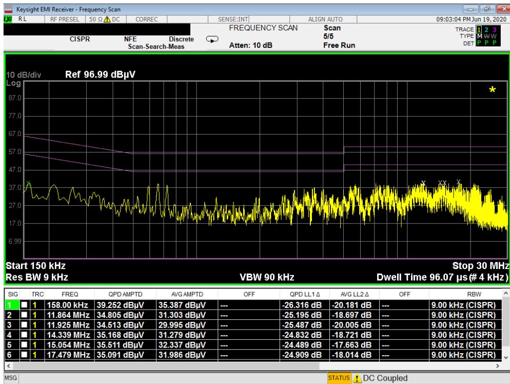
Plot 7-98. Line-Conducted Test Plot (N) – ANTO
