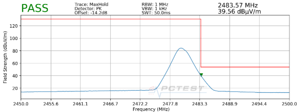
Plot 7-93. Radiated Restricted Upper Band Edge Measurement (Average)
