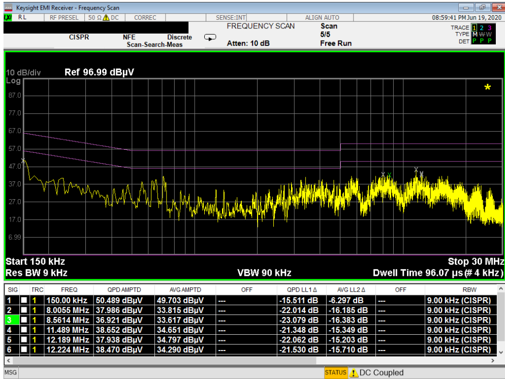
Plot 7-97. Line-Conducted Test Plot (L1) – ANTO
