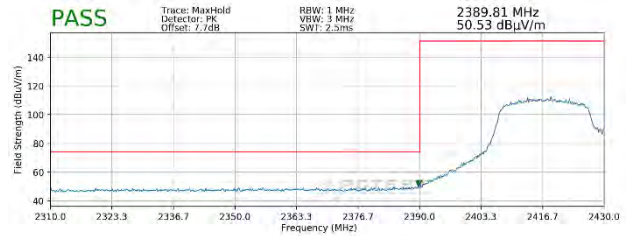
Plot 7-130. Radiated Restricted Lower Band Edge Measurement SISO ANT2 (Peak)
