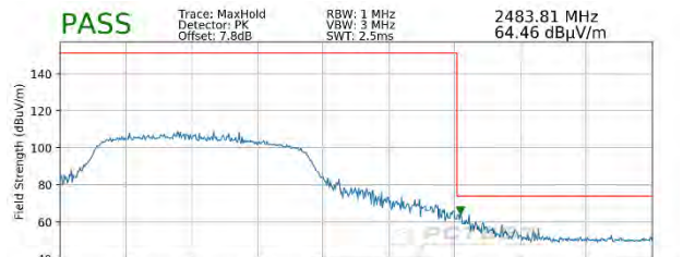
Plot 7-134. Radiated Restricted Upper Band Edge Measurement SISO ANT2 (Peak)
