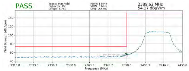
Plot 7-128. Radiated Restricted Lower Band Edge Measurement SISO ANT2 (Peak)
