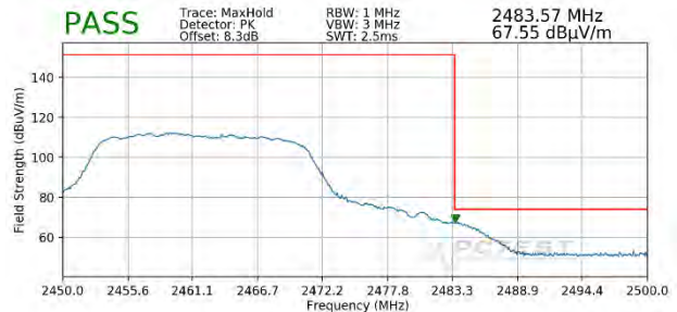
Plot 7-142. Radiated Restricted Upper Band Edge Measurement MIMO (Peak)
