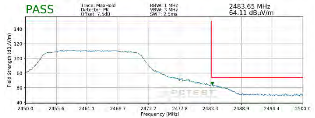
Plot 7-126. Radiated Restricted Upper Band Edge Measurement SISO ANT1 (Peak)
