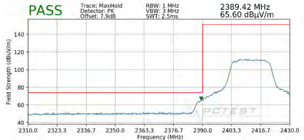
Plot 7-136. Radiated Restricted Lower Band Edge Measurement MIMO (Peak)
