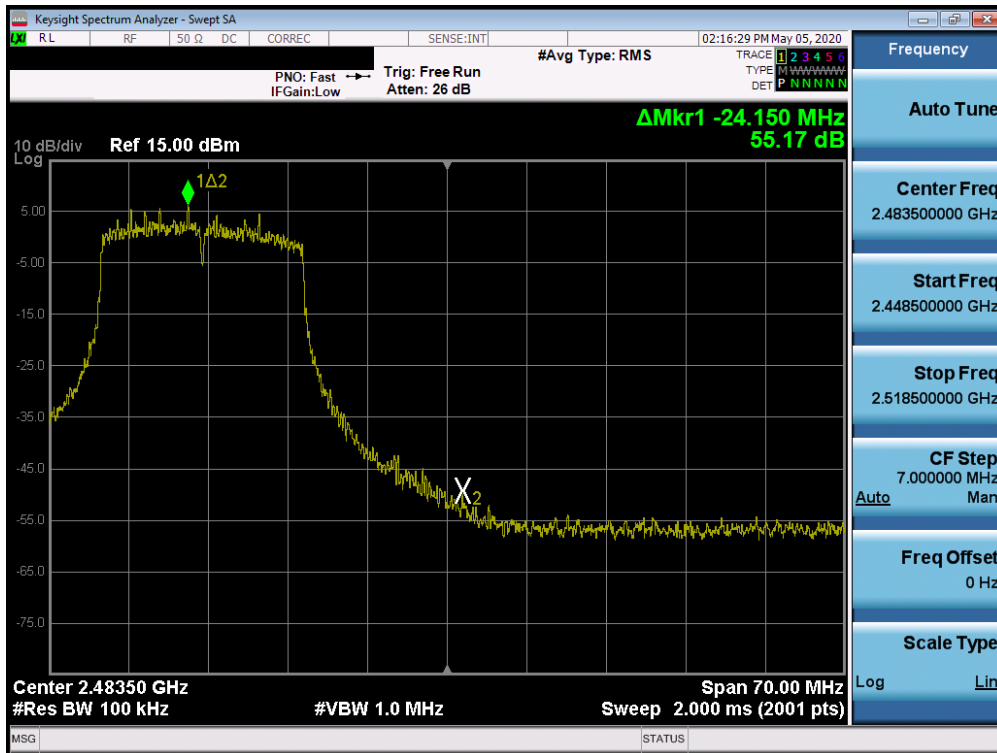
Plot 7-90. Band Edge Plot SISO ANT2 (802.11ax SU (2.4GHz) – Ch. 11)
