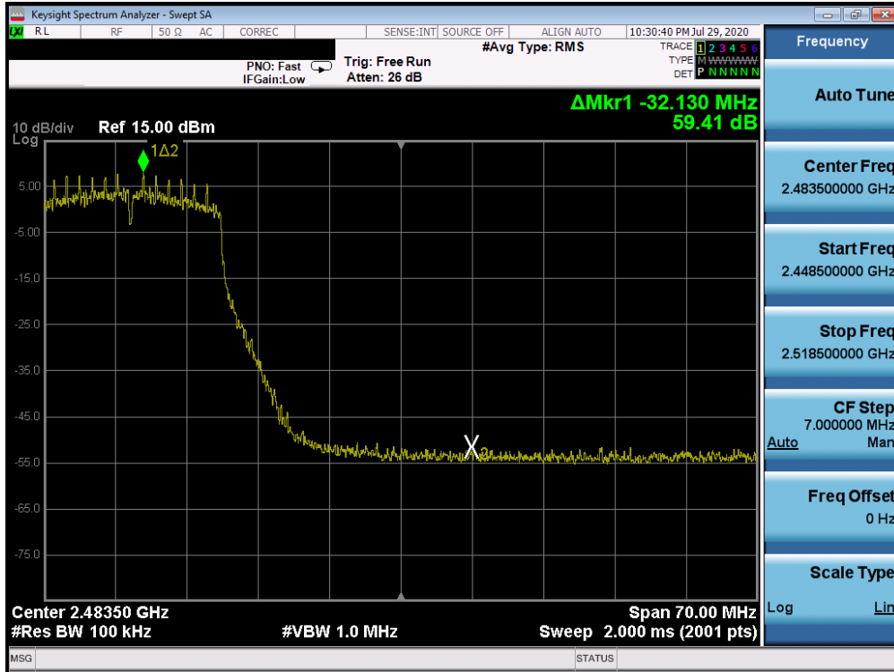
Plot 7-83. Band Edge Plot SISO ANT2 (802.11n (2.4GHz) – Ch. 10)
