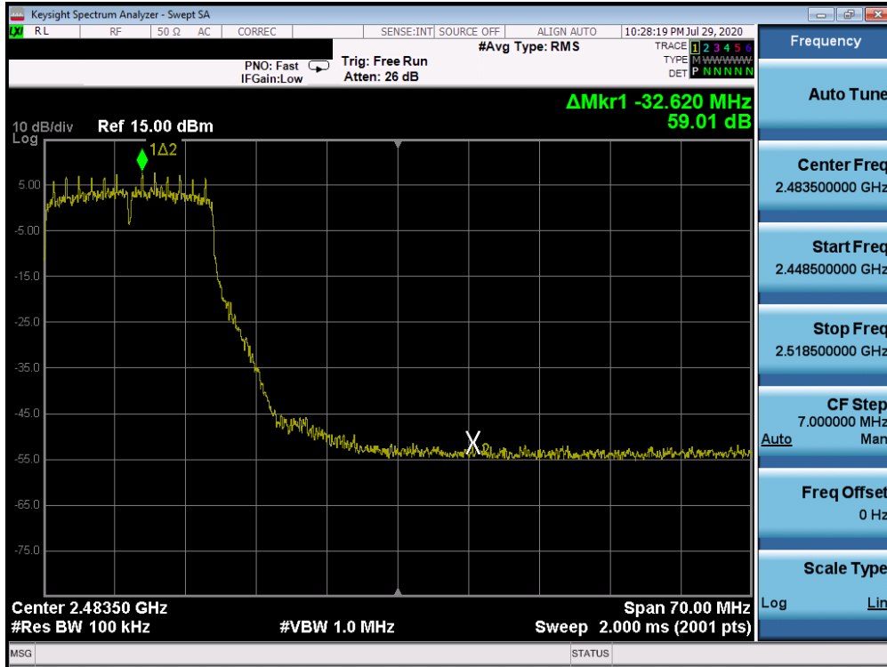
Plot 7-65. Band Edge Plot SISO ANT1 (802.11g – Ch. 10)
