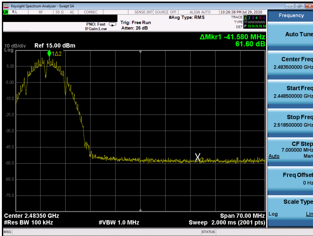
Plot 7-62. Band Edge Plot SISO ANT1 (802.11b – Ch. 10)
