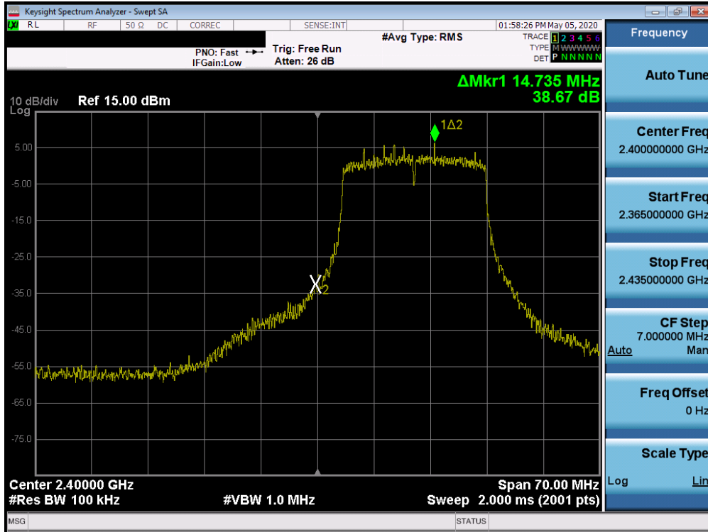
Plot 7-85. Band Edge Plot SISO ANT2 (802.11ac (2.4GHz) – Ch. 1)
