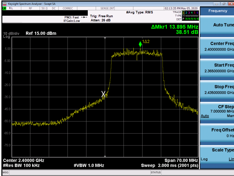
Plot 7-89. Band Edge Plot SISO ANT2 (802.11ax SU (2.4GHz) – Ch. 1)
