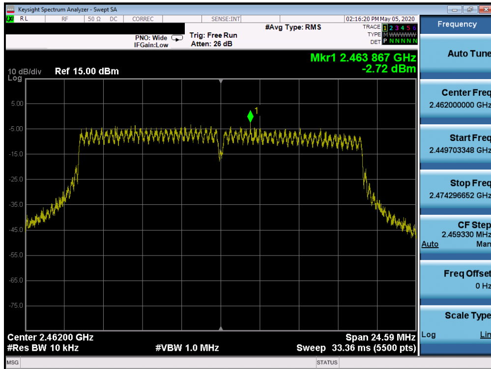
Plot 7-60. Power Spectral Density Plot SISO ANT2 (802.11ax SU (2.4GHz) – Ch. 11)
