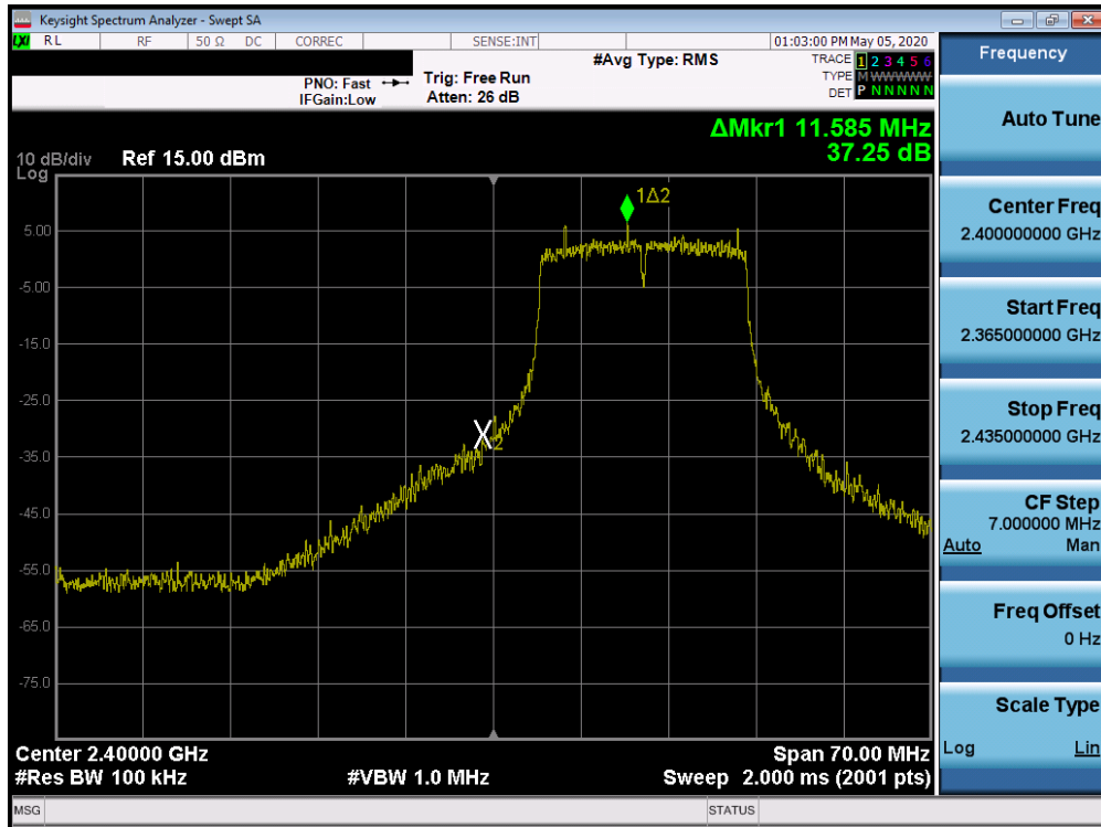
Plot 7-79. Band Edge Plot SISO ANT2 (802.11g- Ch. 1)
