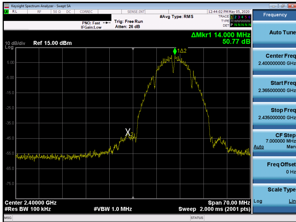
Plot 7-77. Band Edge Plot SISO ANT2 (802.11b – Ch. 1)
