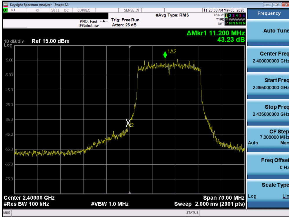
Plot 7-75. Band Edge Plot SISO ANT1 (802.11ax SU (2.4GHz) – Ch. 1)
