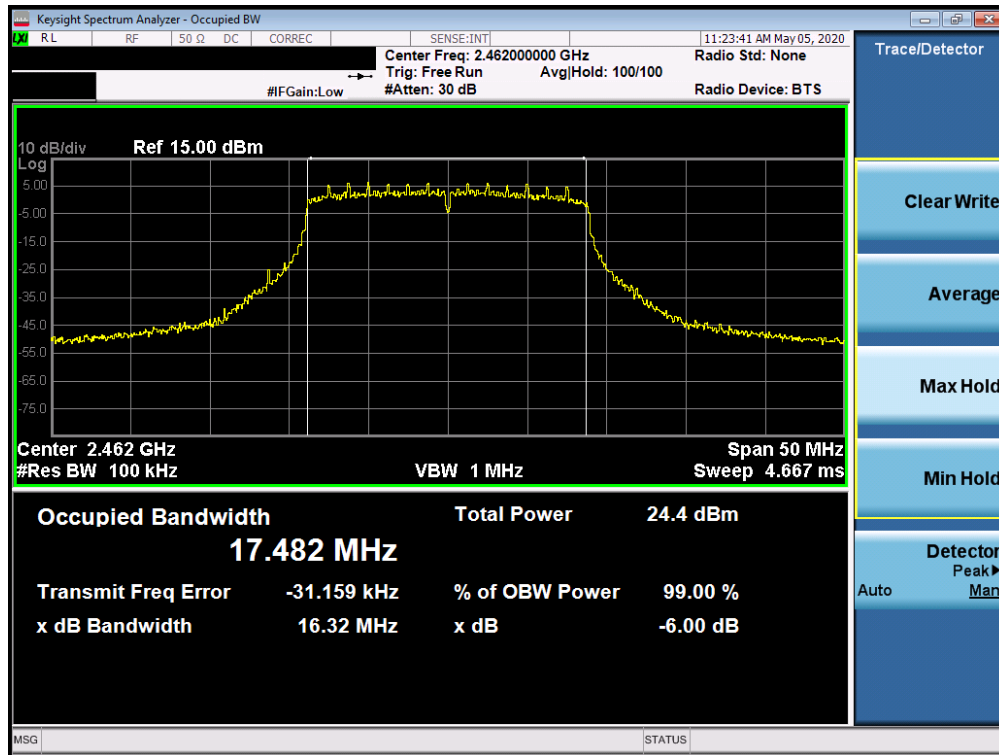
Plot 7-15. 6dB Bandwidth Plot SISO ANT1 (802.11ax SU (2.4GHz) – Ch. 11)
