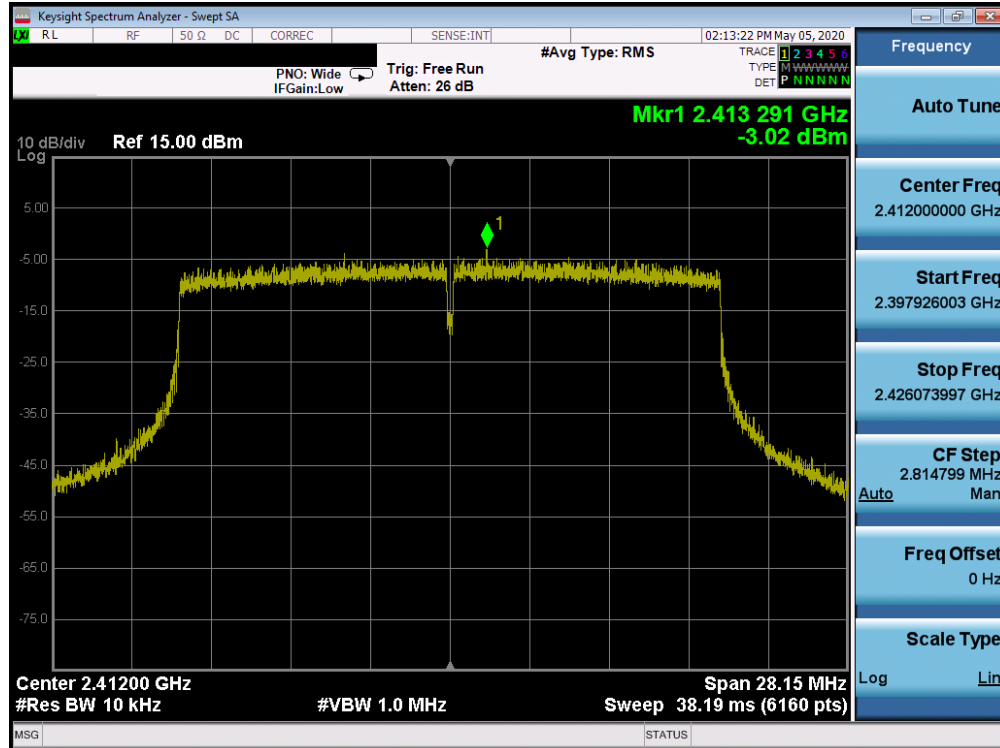
Plot 7-58. Power Spectral Density Plot SISO ANT2 (802.11ax SU (2.4GHz) – Ch. 1)
