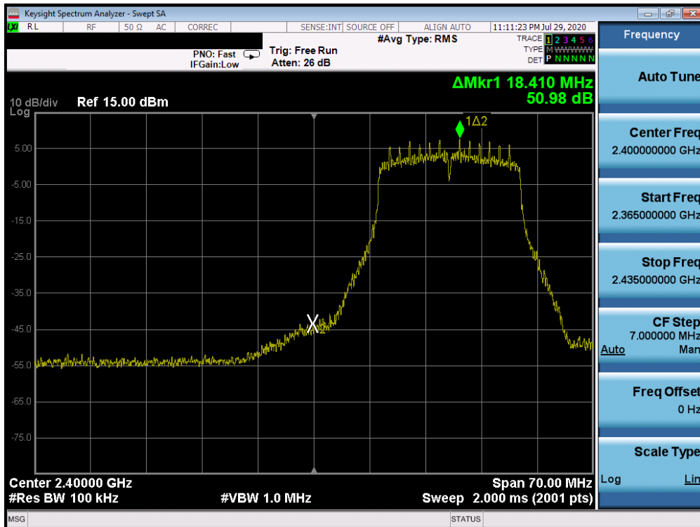
Plot 7-68. Band Edge Plot SISO ANT1 (802.11n (2.4GHz) – Ch. 2)
