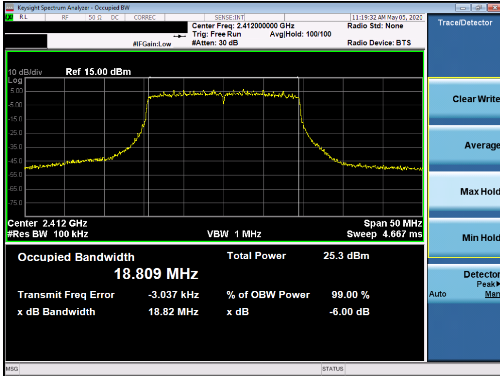
Plot 7-13. 6dB Bandwidth Plot SISO ANT1 (802.11ax SU (2.4GHz) – Ch. 1)
