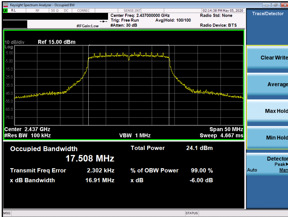
Plot 7-29. 6dB Bandwidth Plot SISO ANT2 (802.11ax SU (2.4GHz) – Ch. 6)
