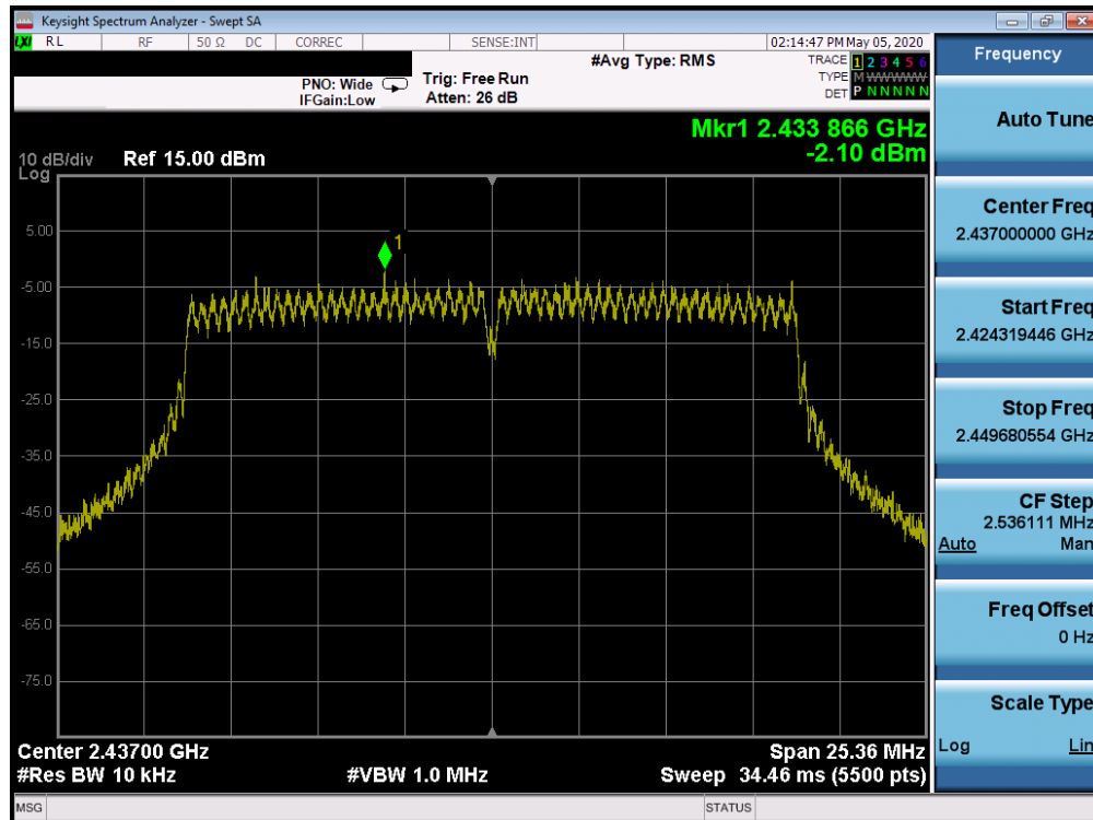
Plot 7-59. Power Spectral Density Plot SISO ANT2 (802.11ax SU (2.4GHz) – Ch. 6)
