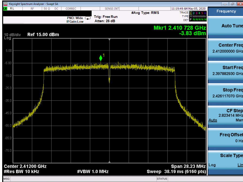
Plot 7-43. Power Spectral Density Plot SISO ANT1 (802.11ax SU (2.4GHz) – Ch. 1)
