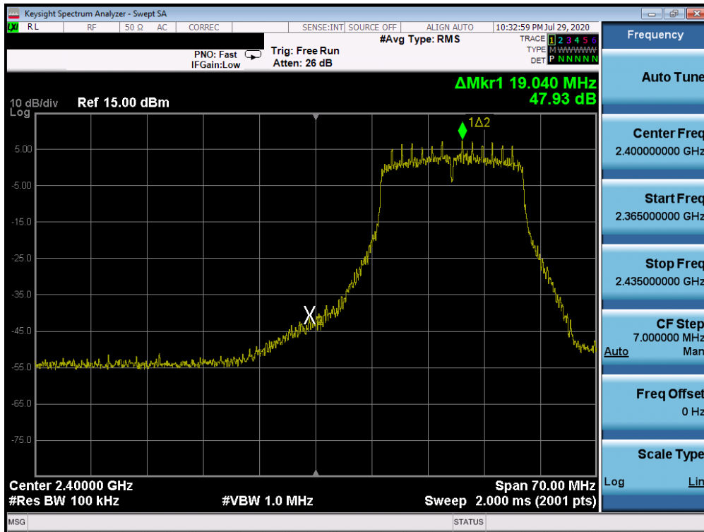
Plot 7-86. Band Edge Plot SISO ANT2 (802.11ac (2.4GHz) – Ch. 2)
