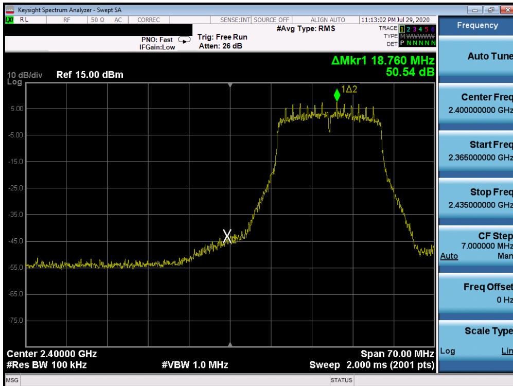
Plot 7-72. Band Edge Plot SISO ANT1 (802.11ac (2.4GHz) – Ch. 2)
