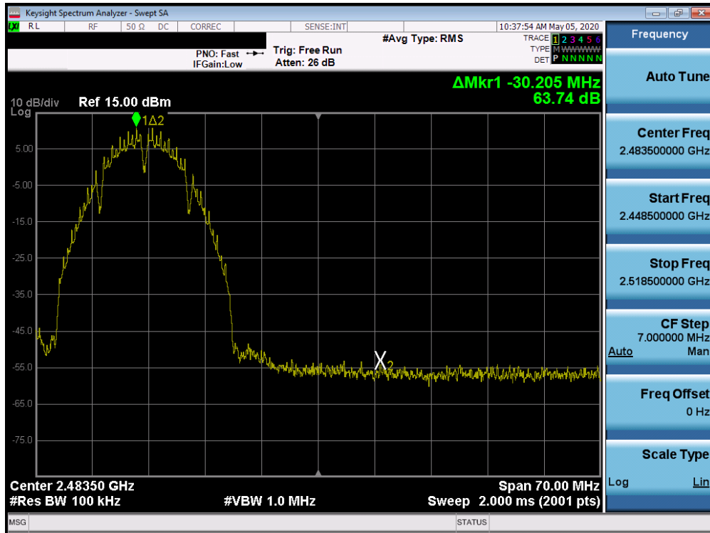
Plot 7-63. Band Edge Plot SISO ANT1 (802.11b – Ch. 11)
