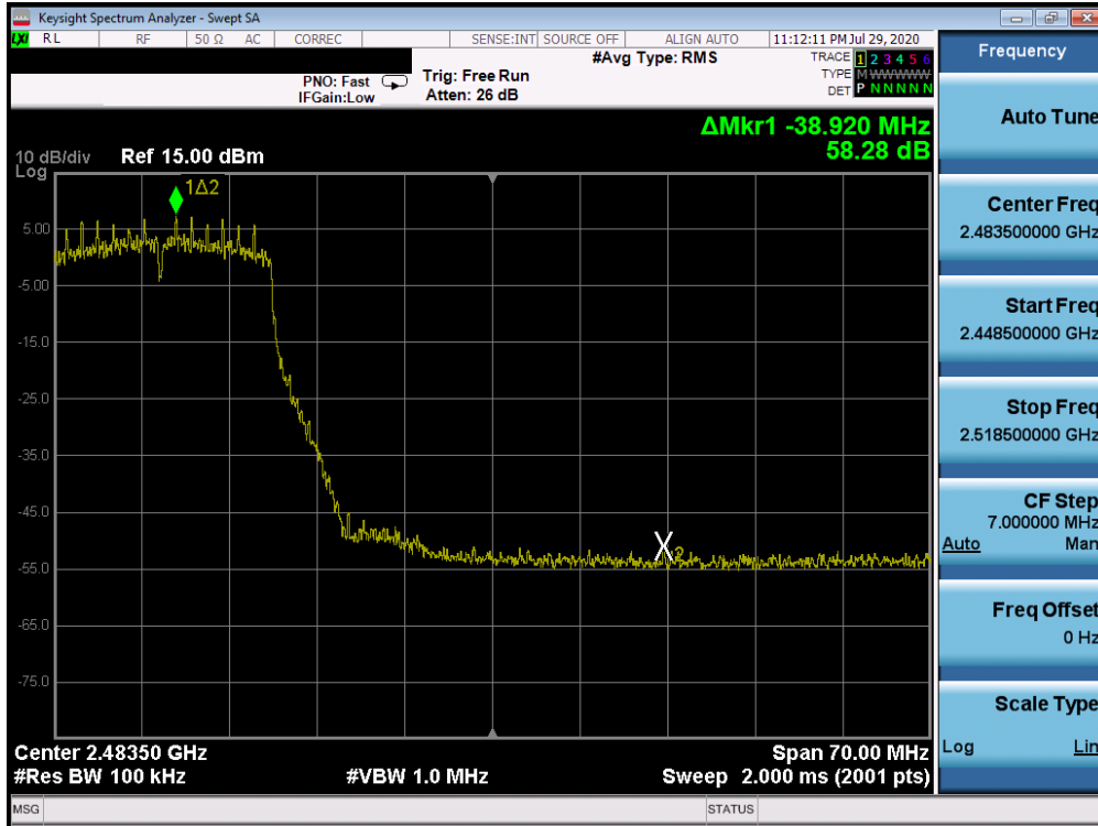
Plot 7-69. Band Edge Plot SISO ANT1 (802.11n (2.4GHz) – Ch. 10)
