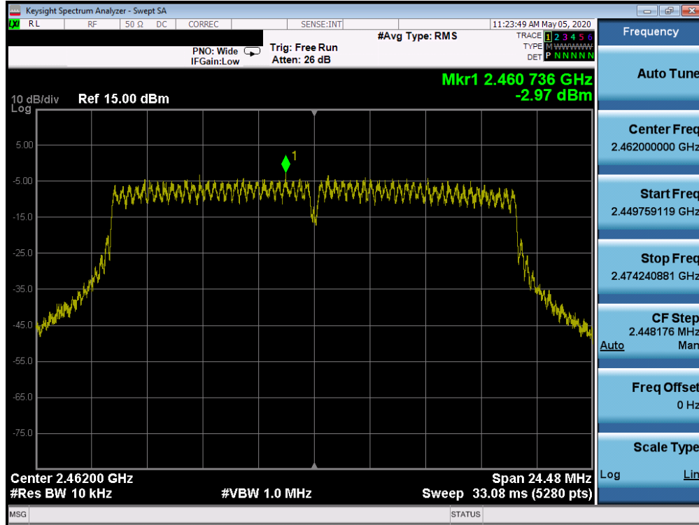
Plot 7-45. Power Spectral Density Plot SISO ANT1 (802.11ax SU (2.4GHz) – Ch. 11)
