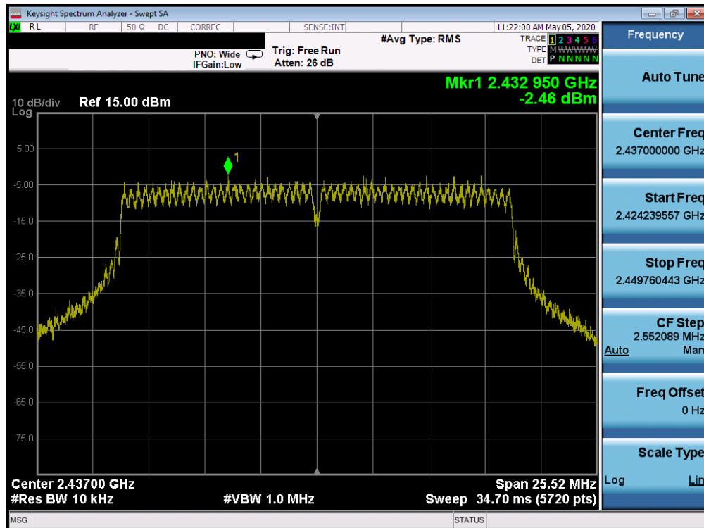
Plot 7-44. Power Spectral Density Plot SISO ANT1 (802.11ax SU (2.4GHz) – Ch. 6)
