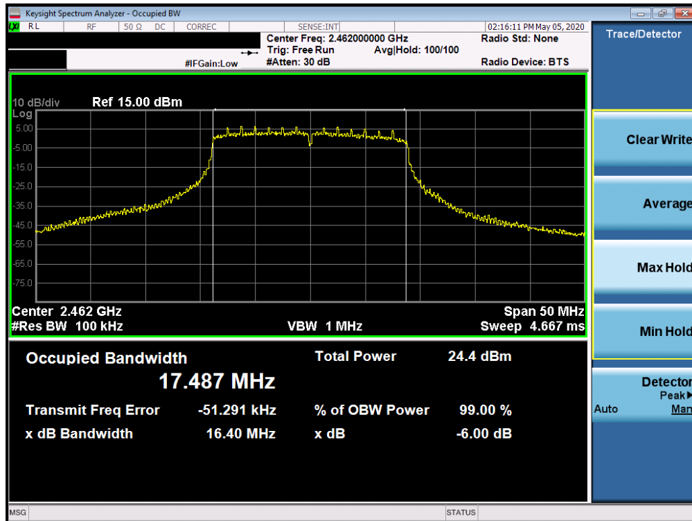
Plot 7-30. 6dB Bandwidth Plot SISO ANT2 (802.11ax SU (2.4GHz) – Ch. 11)
