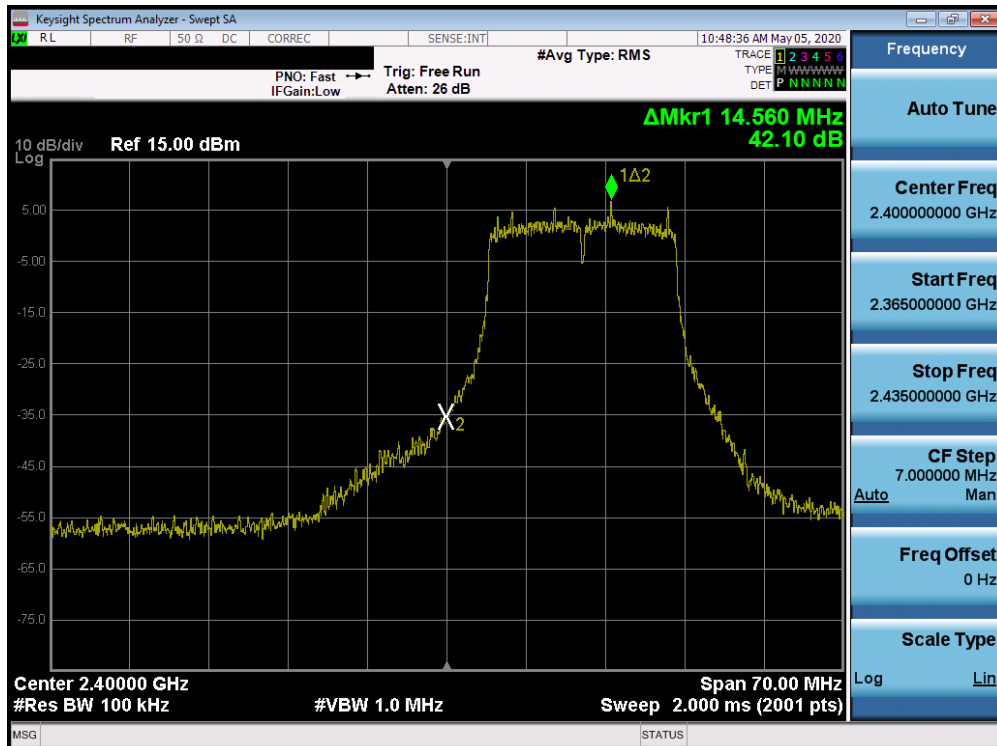
Plot 7-64. Band Edge Plot SISO ANT1 (802.11g– Ch. 1)
