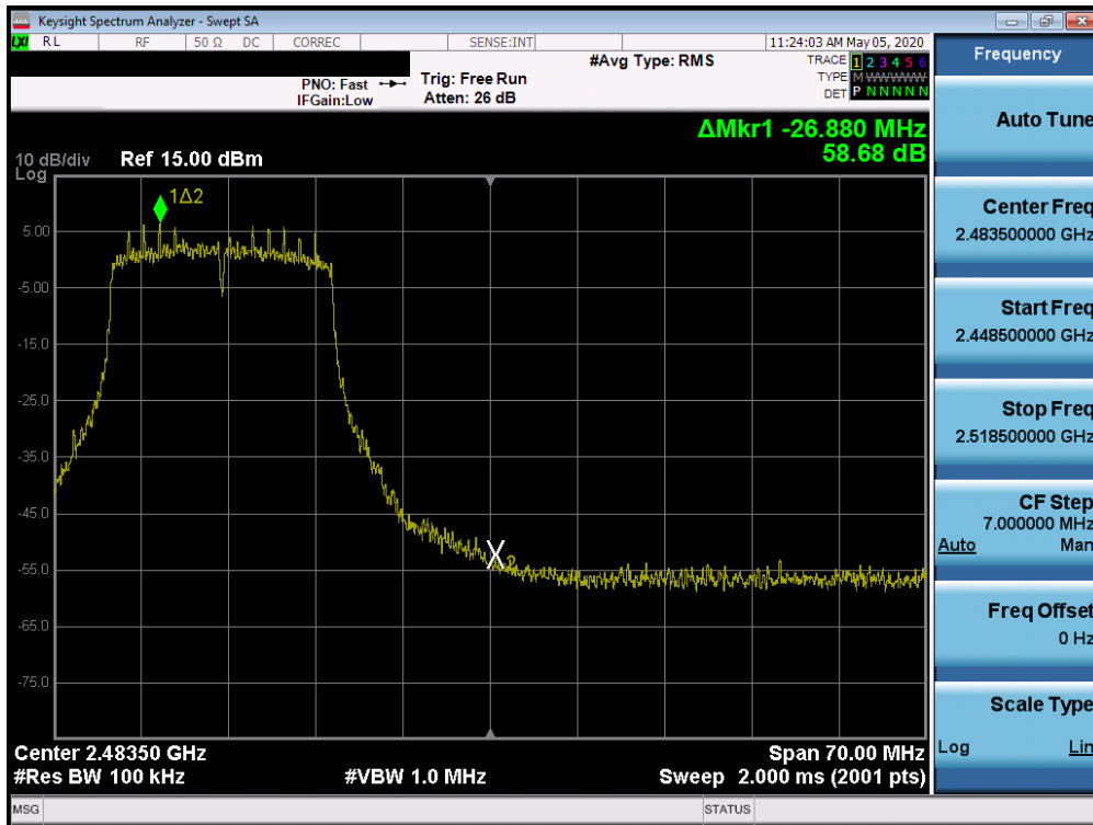
Plot 7-76. Band Edge Plot SISO ANT1 (802.11ax SU (2.4GHz) – Ch. 11)
