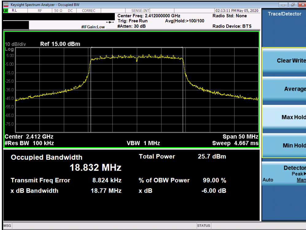
Plot 7-28. 6dB Bandwidth Plot SISO ANT2 (802.11ax SU (2.4GHz) – Ch. 1)
