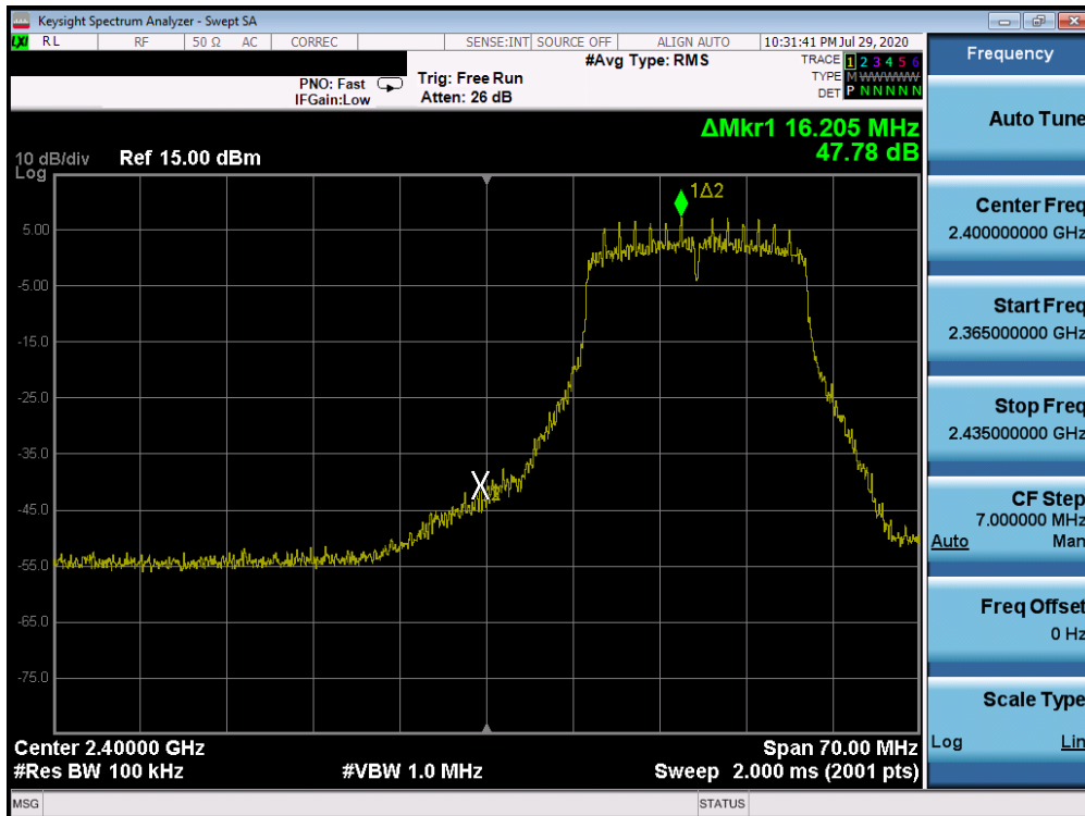
Plot 7-82. Band Edge Plot SISO ANT2 (802.11n (2.4GHz) – Ch. 2)
