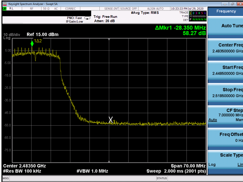
Plot 7-87. Band Edge Plot SISO ANT2 (802.11ac (2.4GHz) – Ch. 10)
