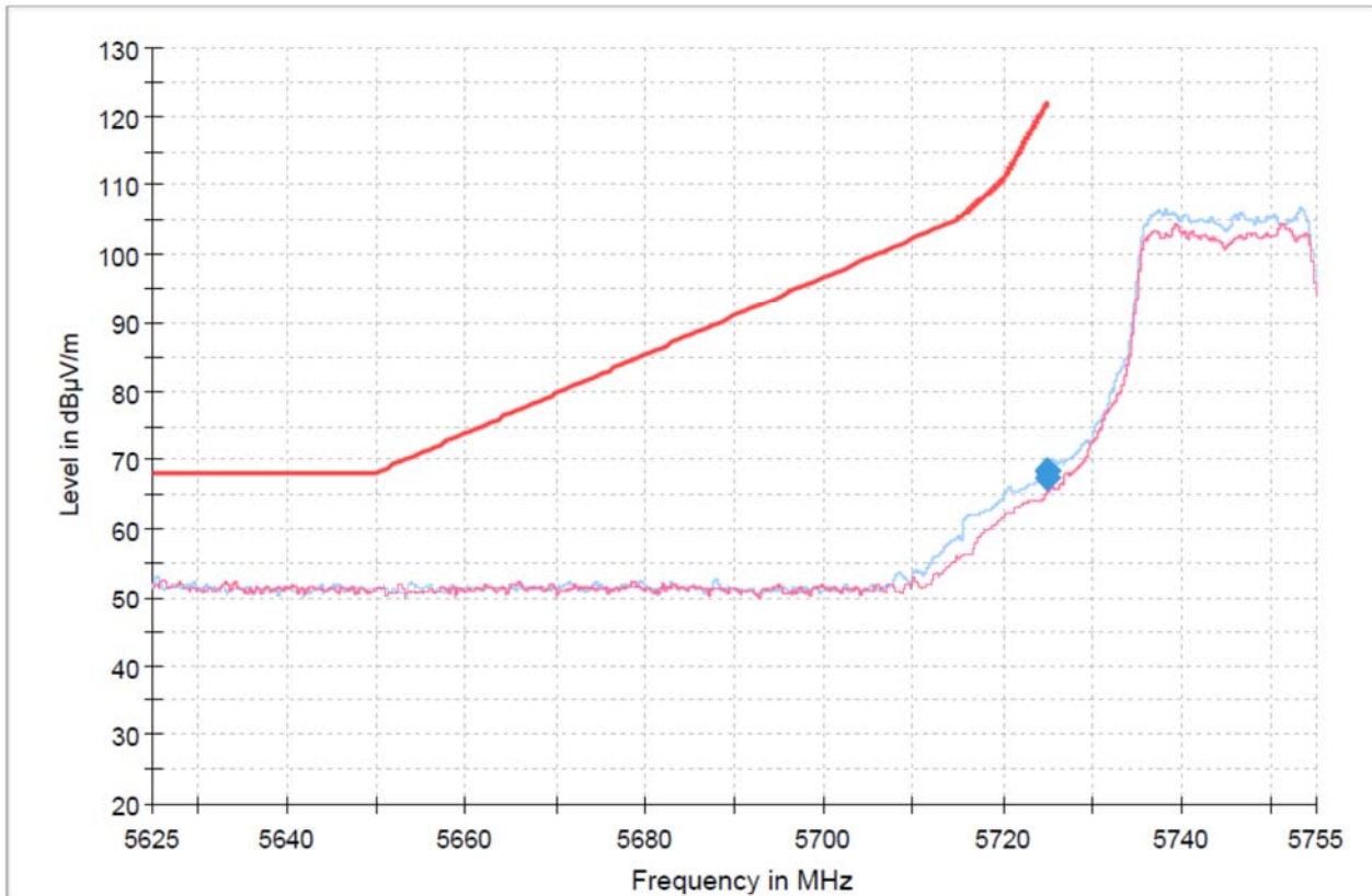
Band Edge_MIMO_UNII-3_802.11ax HE20_5745_SU
