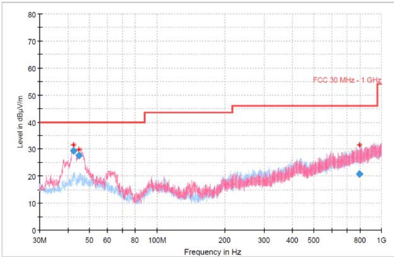
RSE(Below 1G)_MIMO_UNII-3_802.11a_5745
