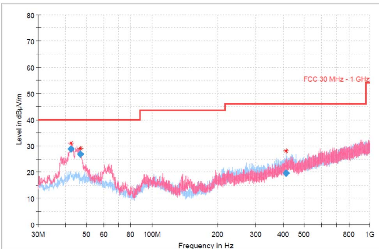
RSE_MIMO_UNII-2A_802.11a_5320
