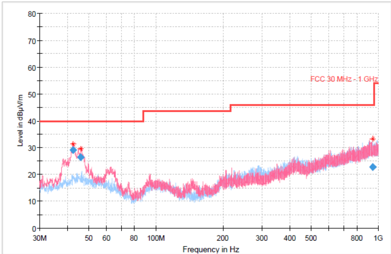
RSE_MIMO_UNII-2C_802.11a_5500
