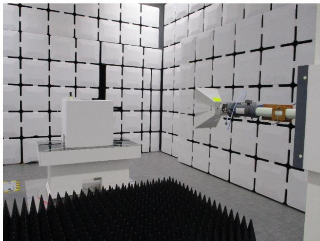
RADIATED FRONT PHOTO (ABOVE 1 GHz)
