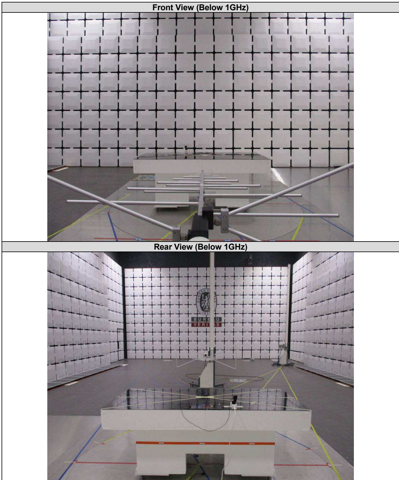
Figure 1. Photo of Radiated emission test setup
