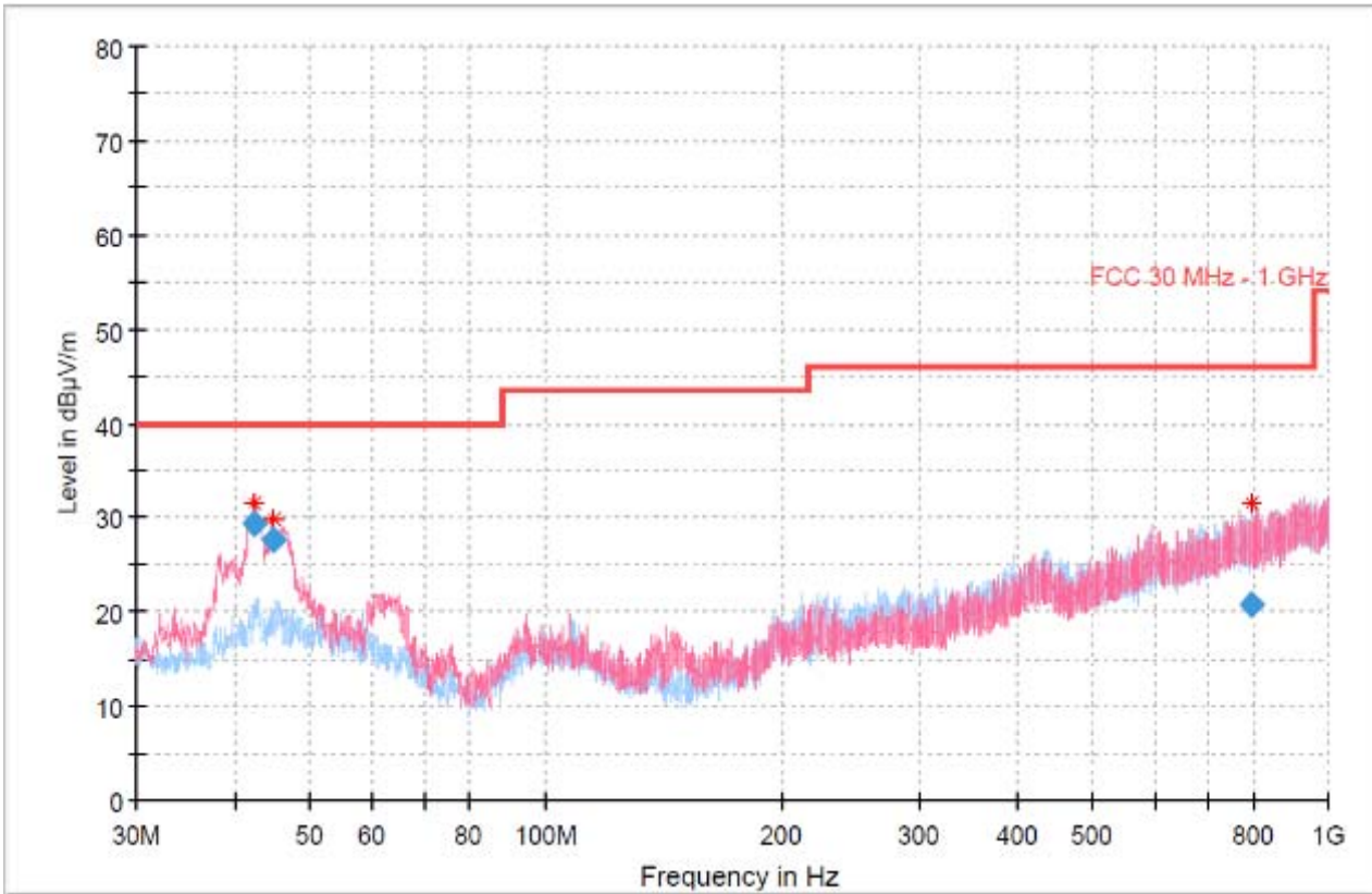
RSE(Below 1G)_MIMO_UNII-3_802.11a_5745
