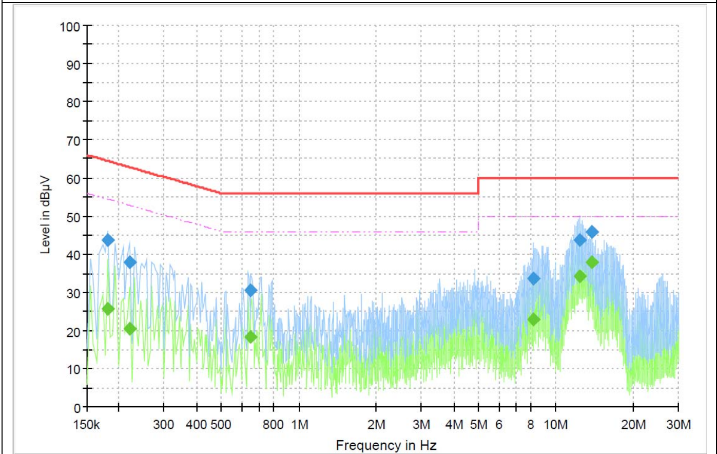
SISO_ANT1_UNII-1_802.11a_5180
