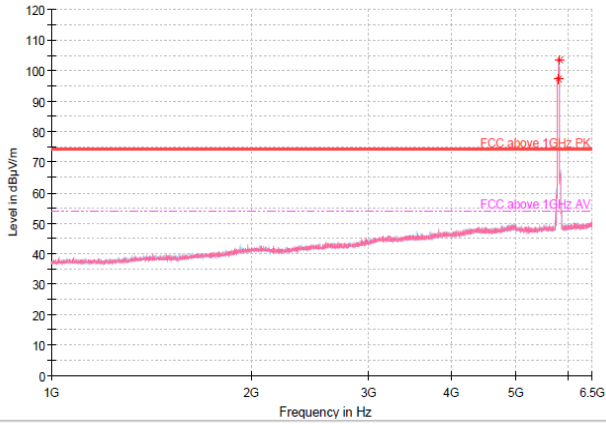
1 GHz - 6.5 GHz
