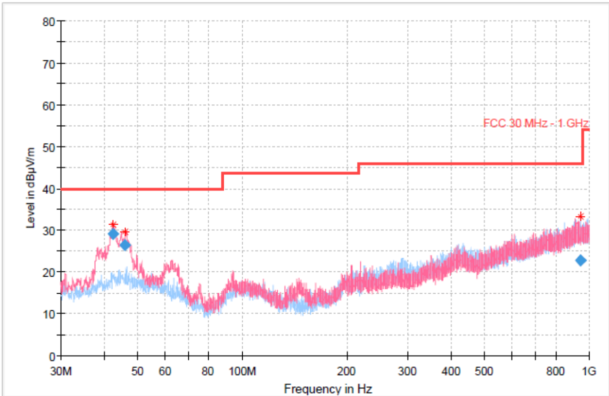
RSE_MIMO_UNII-2C_802.11a_5500
