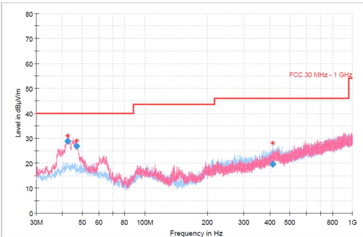
RSE_MIMO_UNII-2A_802.11a_5320
