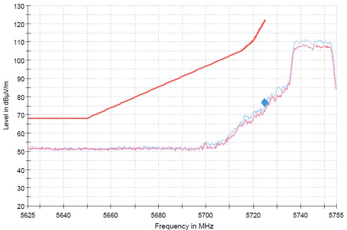
Band Edge_MIMO_UNII-3_802.11a_5745
