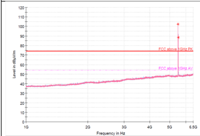
1 GHz - 6.5 GHz
