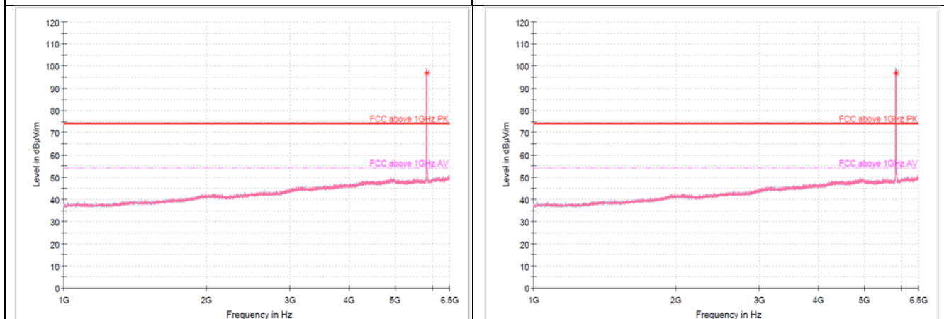
1 GHz - 6.5 GHz
