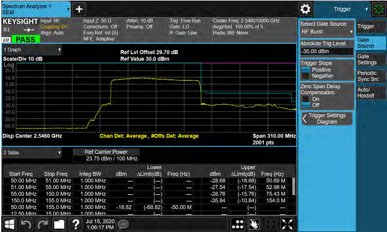
Sub6 n41. Low Channel Edge Plot (100 MHz Ch.509202 BPSK_RB25_Offset 0)-2
