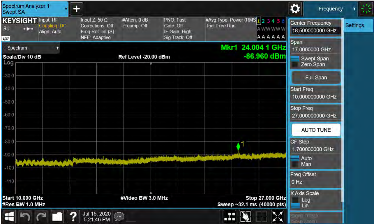
Sub6 n41. Conducted Spurious Plot 2 (80 MHz Ch.52998 BPSK RB 1, Offset 0)
