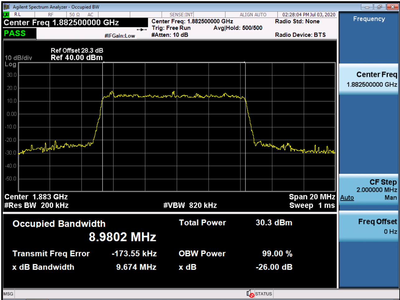
Sub6 n25(2). Occupied Bandwidth Plot (10M BW Ch.376500 16QAM RB 50_0)
