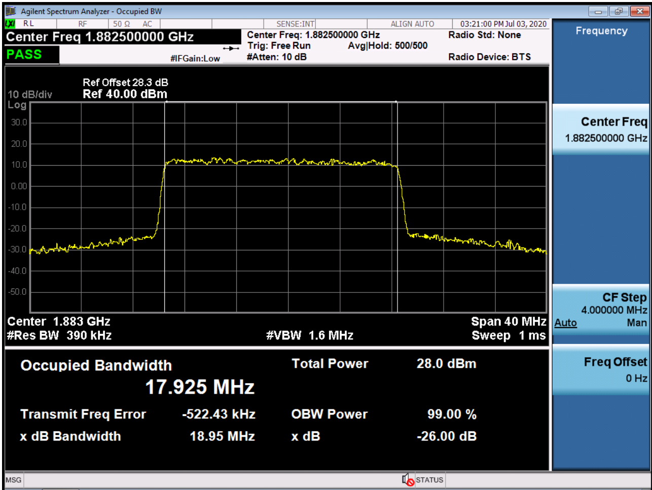
Sub6 n25(2). Occupied Bandwidth Plot (20M BW Ch.376500 256QAM RB 100_0)
