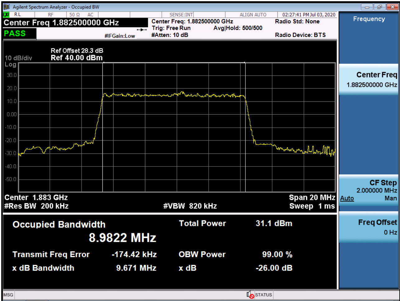
Sub6 n25(2). Occupied Bandwidth Plot (10M BW Ch.376500 QPSK RB 50_0)
