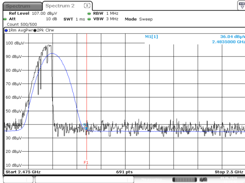
Radiated Restricted Band Edges plot – Average Reading (Ch.39, Z-H)
