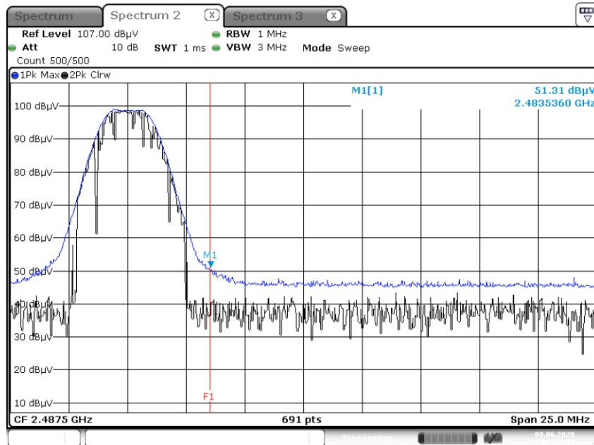
Radiated Restricted Band Edges plot – Peak Reading (Ch.39, Z-H)
