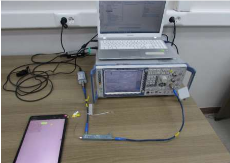
Test setup photo-1 (8-1(a) Legacy)
