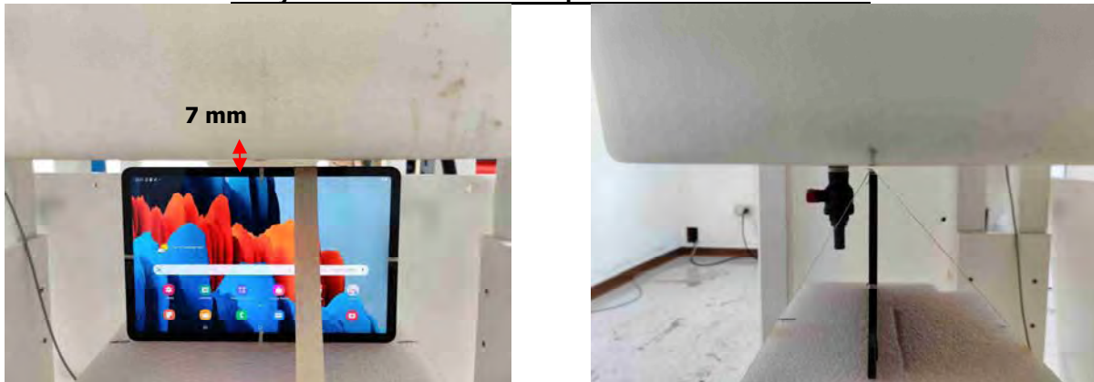
Fig.10 EUT Left side to flat phantom
