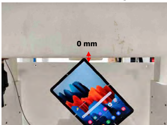
Fig.8 EUT Right corner side to flat phantom
